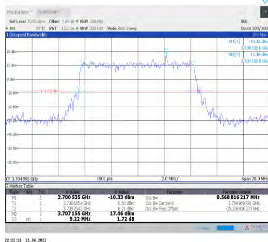
1-N77-3700-3980--30-10-L-2-DFT-PI2BPSK-Outer_Full -24@0-Ant1-8.569-9.220-≤10-PASS
