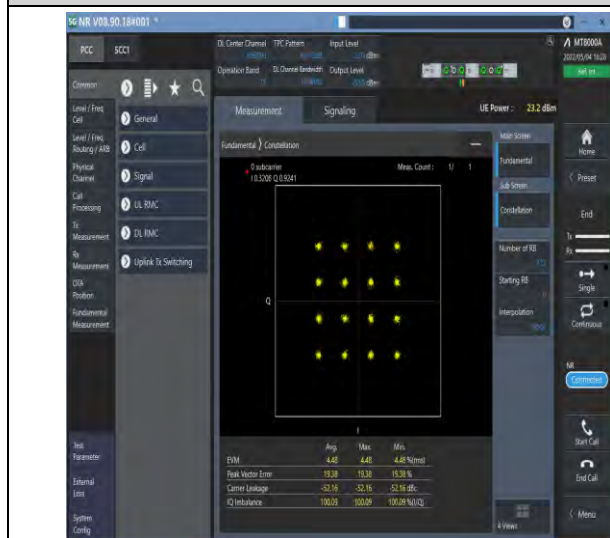
1-N77-3700-3980-PC2-30-100-M-7-CP-16QAM-Outer_Full-273@0-Ant1-see graph-PASS
