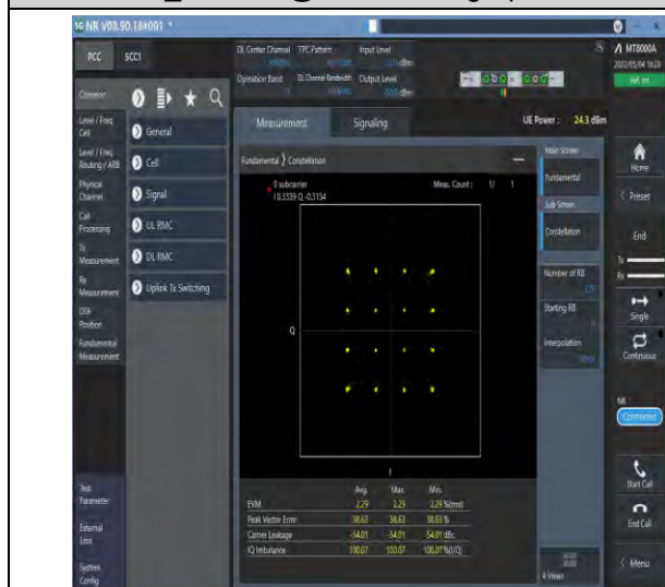
1-N77-3700-3980-PC2-30-100-M-3-DFT-16QAM-Out_uter_Full-270@0-Ant1-see graph-PASS
