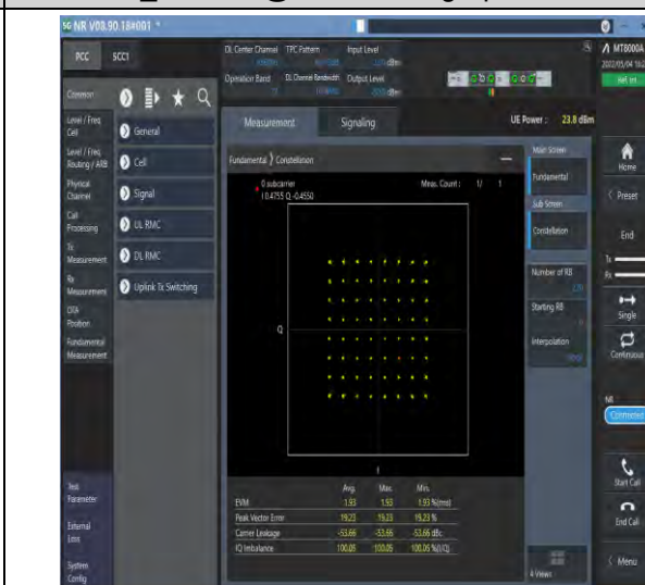
1-N77-3700-3980-PC2-30-100-M-4-DFT-64QAM-Out_uter_Full-270@0-Ant1-see graph-PASS
