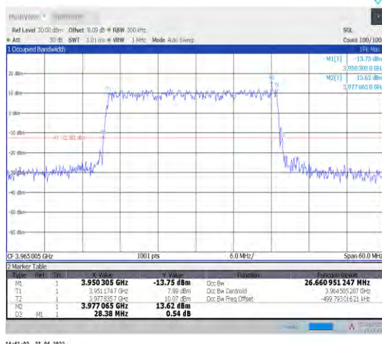
1-N77-3700-3980--30-30-H-3-DFT-16QAM-Outer_Full-75@0-Ant1-26.665-28.380-<30-PASS
