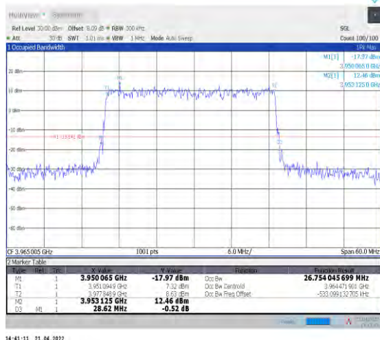
1-N77-3700-3980--30-30-H-4-DFT-64QAM-Outer_Full-75@0-Ant1-26.756-28.620-<30-PASS
