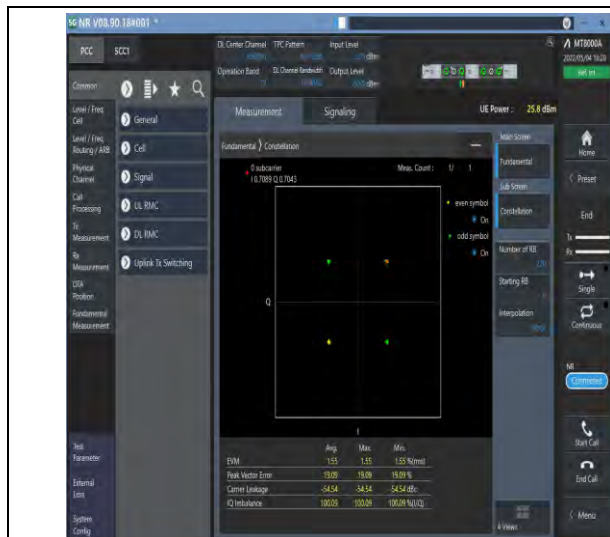
1-N77-3700-3980-PC2-30-100-M-1-DFT-PI2BPSK-Out_uter_Full-270@0-Ant1-see graph-PASS
