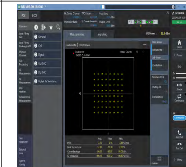
1-N77-3700-3980-PC2-30-100-M-8-CP-64QAM-Outer_Full-273@0-Ant1-see graph-PASS
