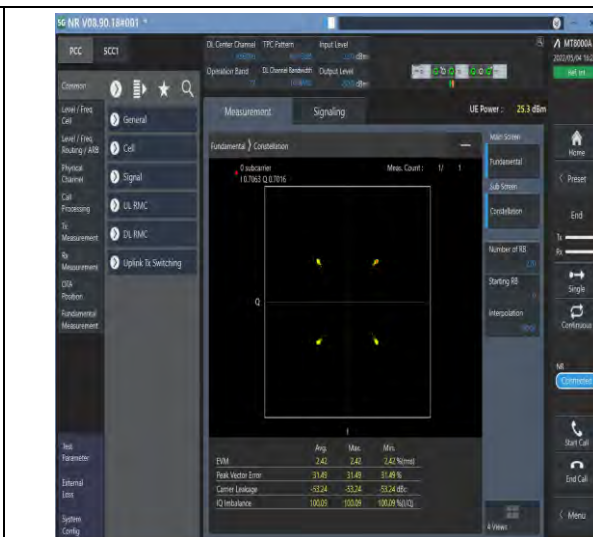
1-N77-3700-3980-PC2-30-100-M-2-DFT-QPSK-Out_uter_Full-270@0-Ant1-see graph-PASS
