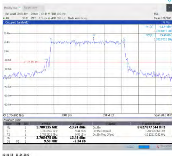
1-N77-3700-3980--30-10-L-1-DFT-QPSK-Outer_Full -24@0-Ant1-8.628-9.580-≤10-PASS
