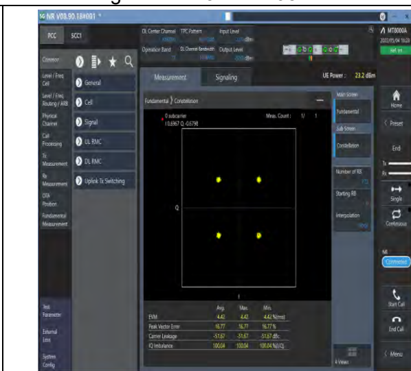
1-N77-3700-3980-PC2-30-100-M-6-CP-QPSK-Outer_Full-273@0-Ant1-see graph-PASS
