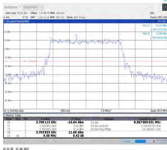
1-N77-3700-3980--30-10-L-4-DFT-64QAM-Outer_Full -24@0-Ant1-8.567-9.580-≤10-PASS
