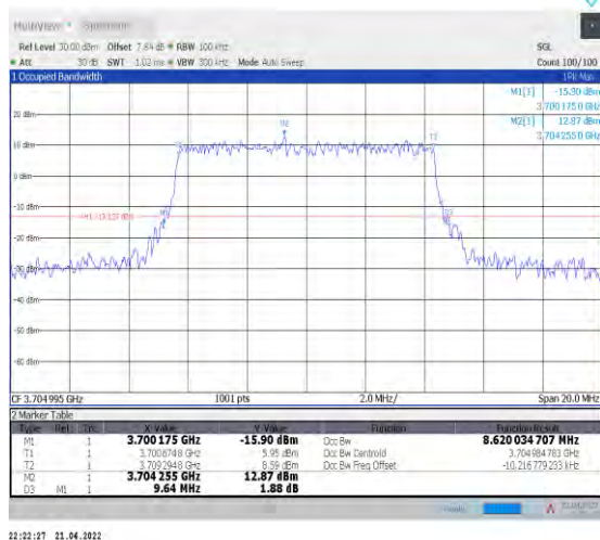
1-N77-3700-3980--30-10-L-3-DFT-16QAM-Outer_Full -24@0-Ant1-8.62-9.640-≤10-PASS
