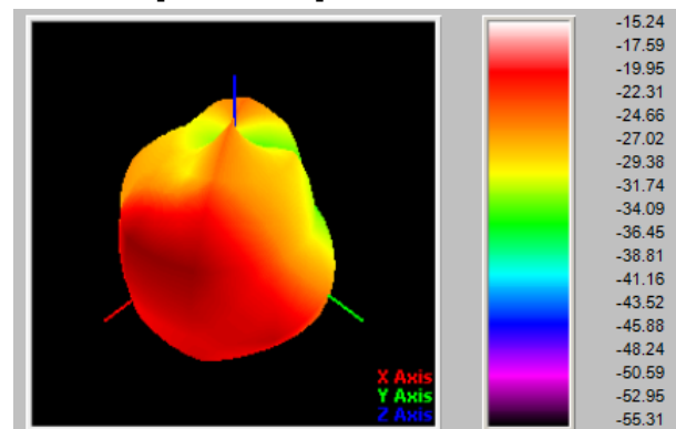
LTEB4[1710MHz]
