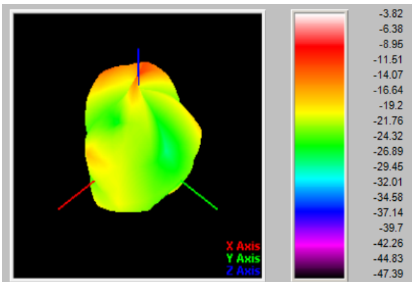
LTEB40[2300MHz]
