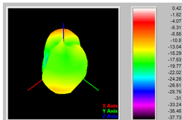
LTEB7[2500MHz]
