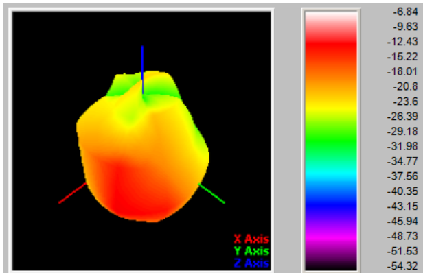
LTEB3[1710MHz]
