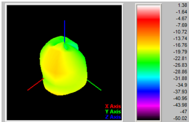
LTEB17[704MHz]
