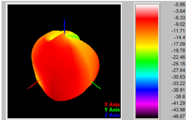
LTEB17[704MHz]
