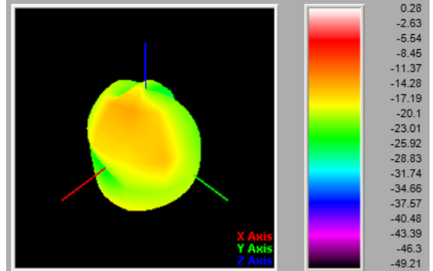
LTEB20[832MHz]
