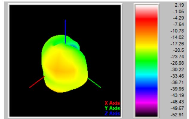
EGSM[900MHz]
