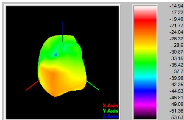
DCS[1800MHz]
