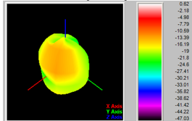
LTEB26[814MHz]
