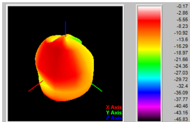
GSM850[850MHz]
