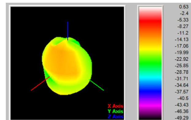
LTEB5[824MHz]
