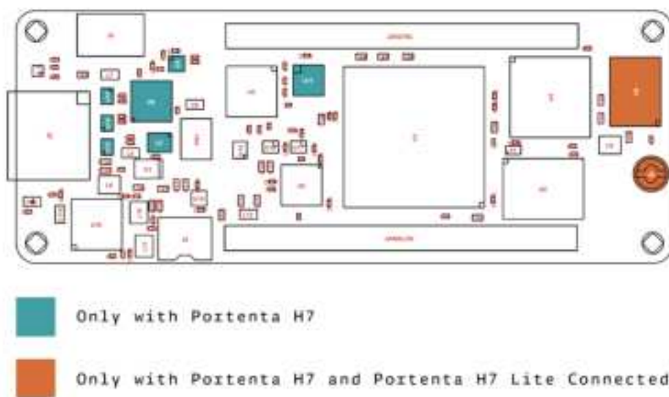
Board Topology
