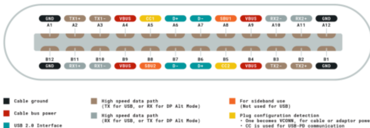
USB-C Pinout
