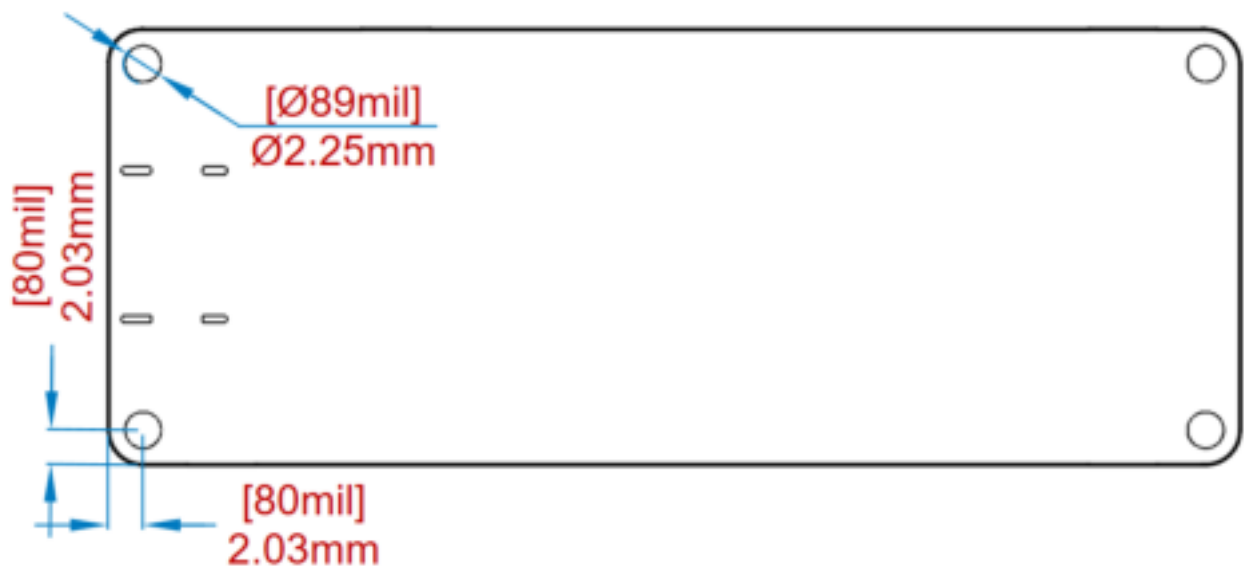
Mounting outline
