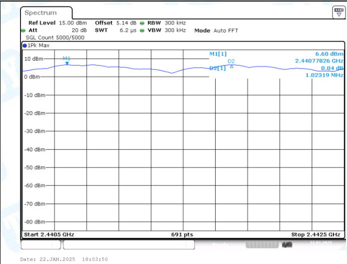
2DH5-Ant1-Hop-PASS
