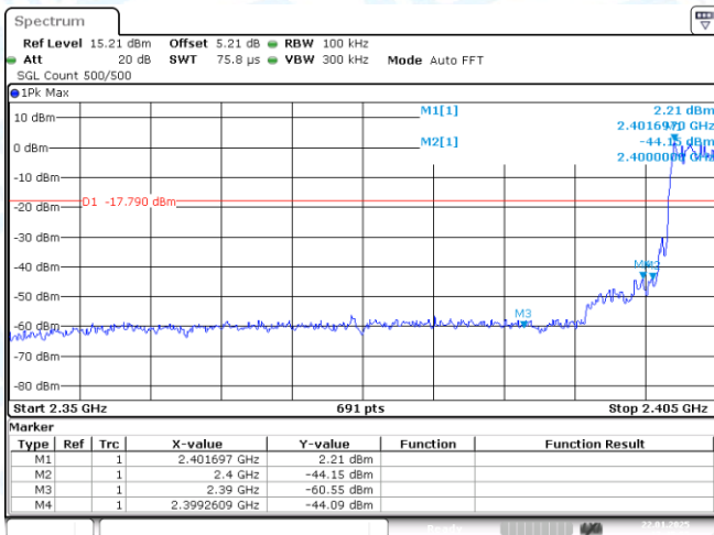
3DH5-Ant1-2402-PASS
