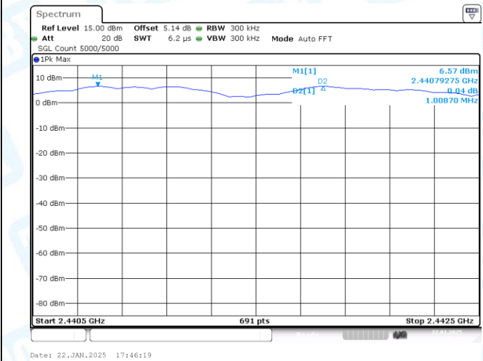
3DH5-Ant1-Hop-PASS
