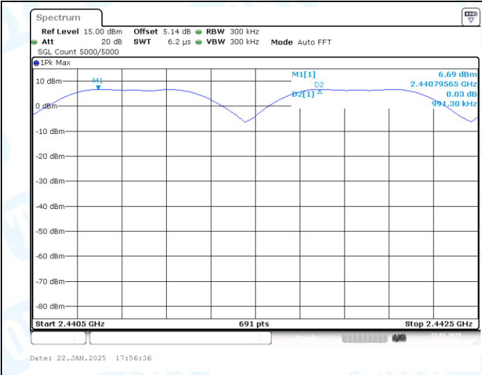
DH5-Ant1-Hop-PASS
