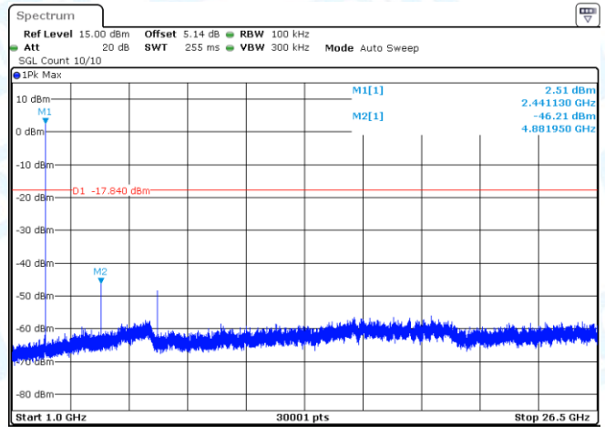
DH5-Ant1-2441-0~Reference-PASS
