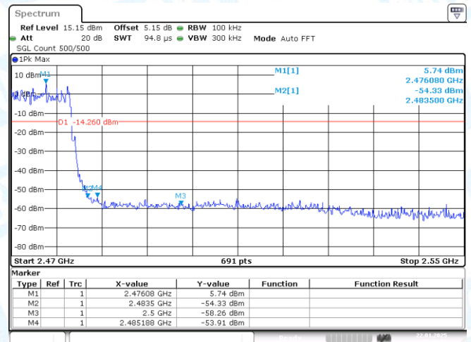
3DH5-Ant1-2480-PASS
