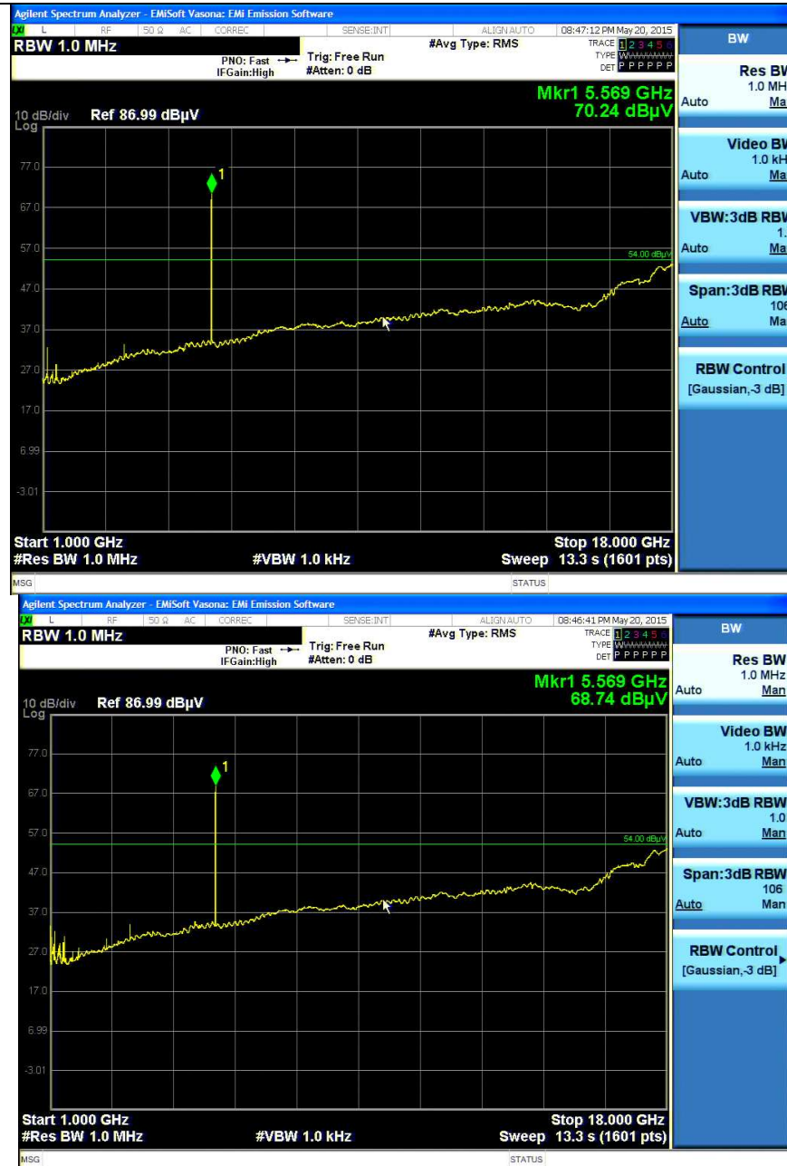
Title: 1 - 18GHz Test Results at 5560MHz (Average)
