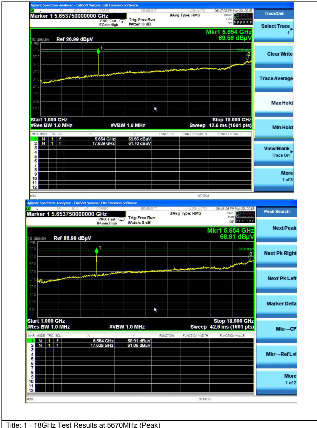
Title: 1 - 18GHz Test Results at 5670MHz (Peak)
