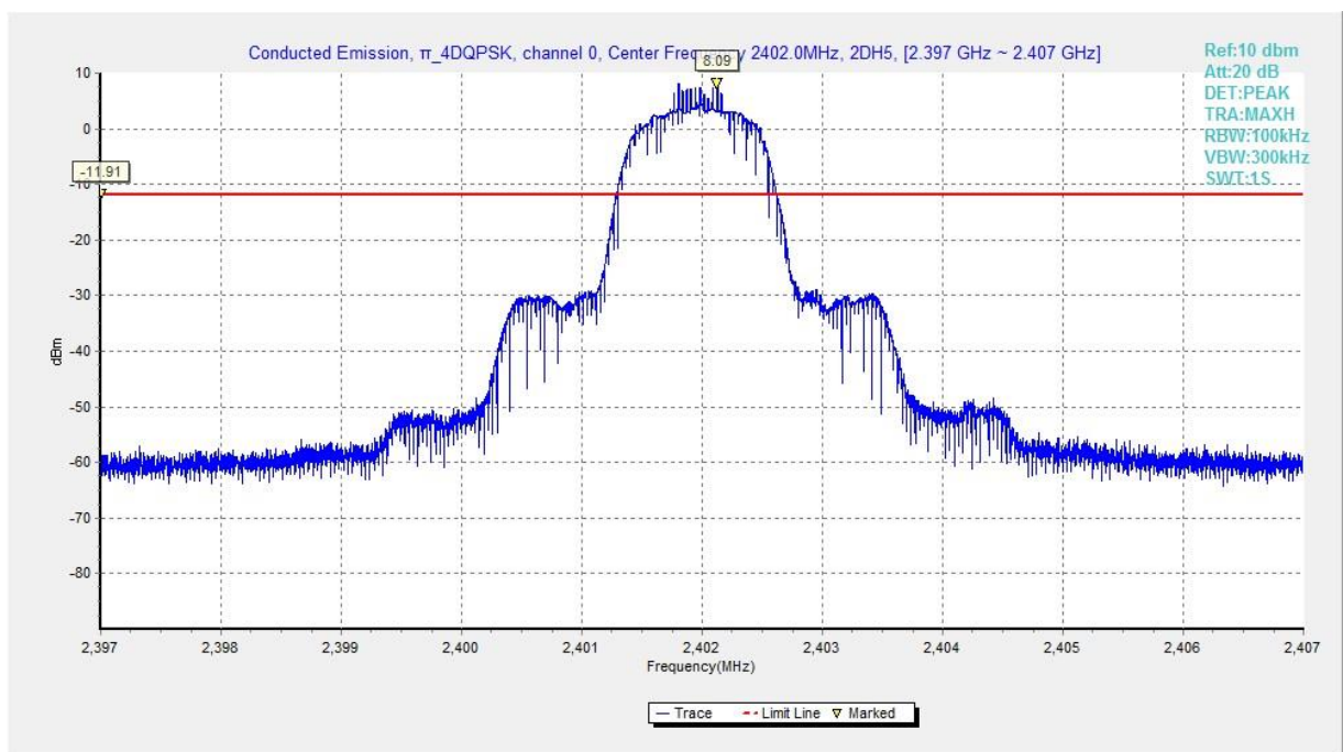
Fig. 22 Conducted Spurious Emission ( \pi_4 QPSK, Ch0, 2.402GHz)
