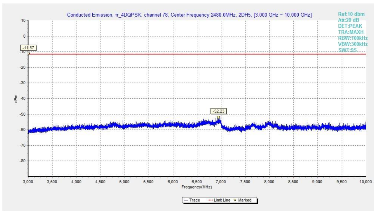
Fig. 30 Conducted Spurious Emission ( \pi/4 DQPSK, Ch78, 3GHz-10 GHz)
