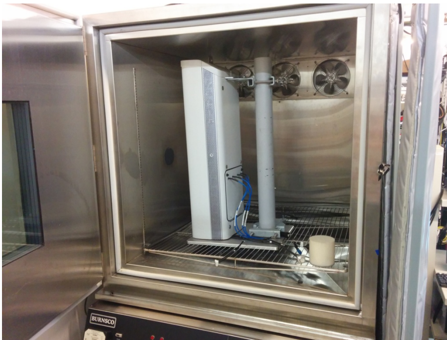
Lab Testing – Base Station in Temperature Chamber
