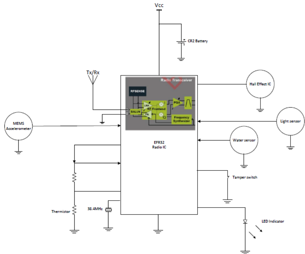
Figure 3.6-1: Setup diagram Multi sensor
