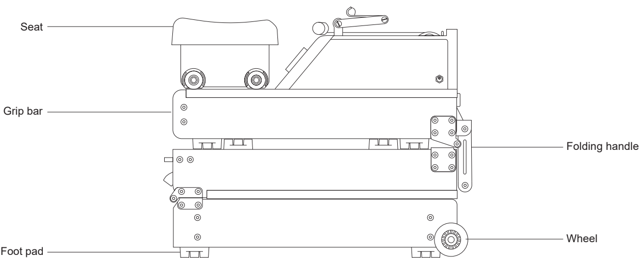
Folded state
