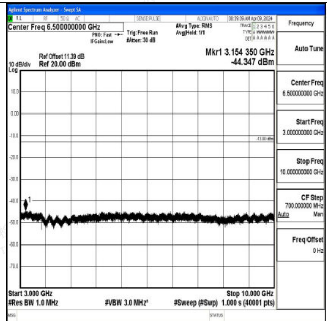
Band26_1.4MHz_16QAM_26783_1RB#0_3000~10000_300 0~10000
