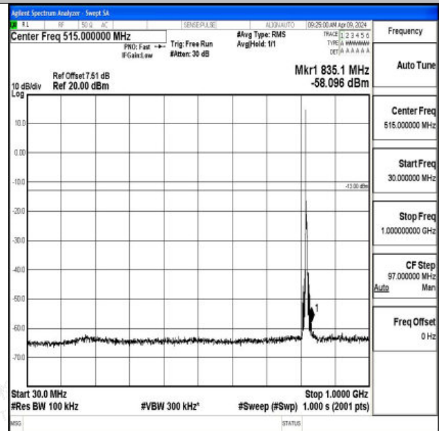
Band26_5MHz_16QAM_26765_1RB#0_30~1000_30~1000
