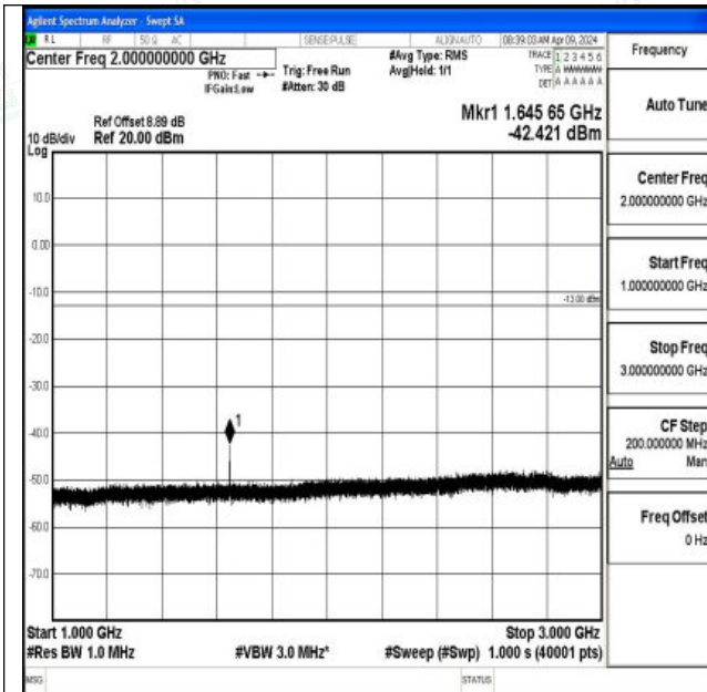
Band26_1.4MHz_16QAM_26783_1RB#0_1000~3000_100 0~3000
