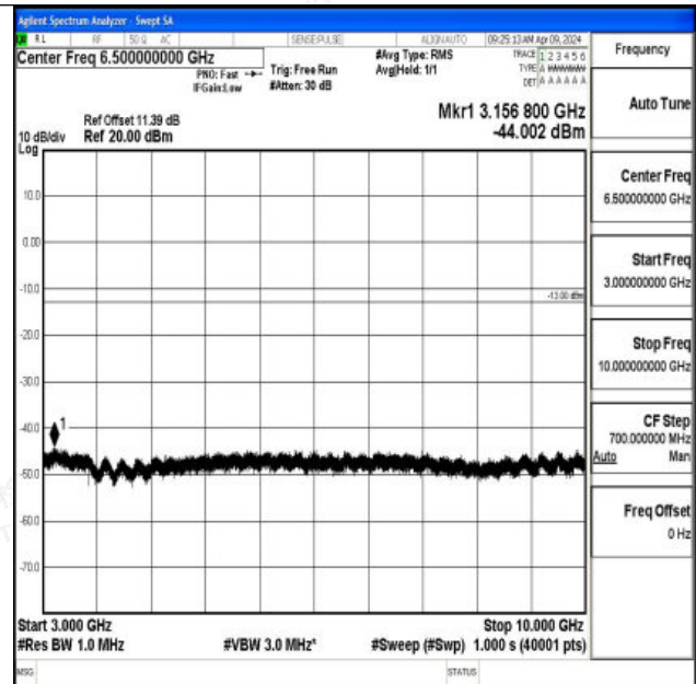
Band26_5MHz_16QAM_26765_1RB#0_3000~10000_3000 ~10000
