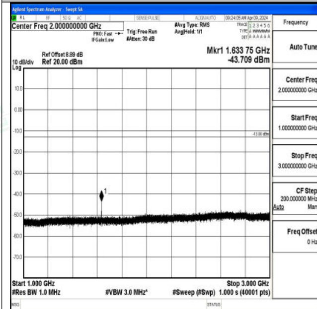
Band26_5MHz_16QAM_26740_1RB#0_1000~3000_1000~3000
