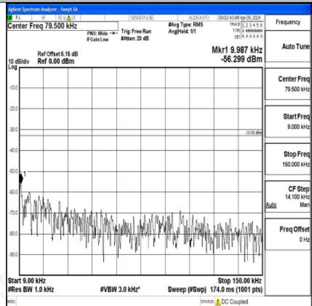
Band26_3MHz_16QAM_26705_1RB#0_0.009~0.15_0.009~0.15
