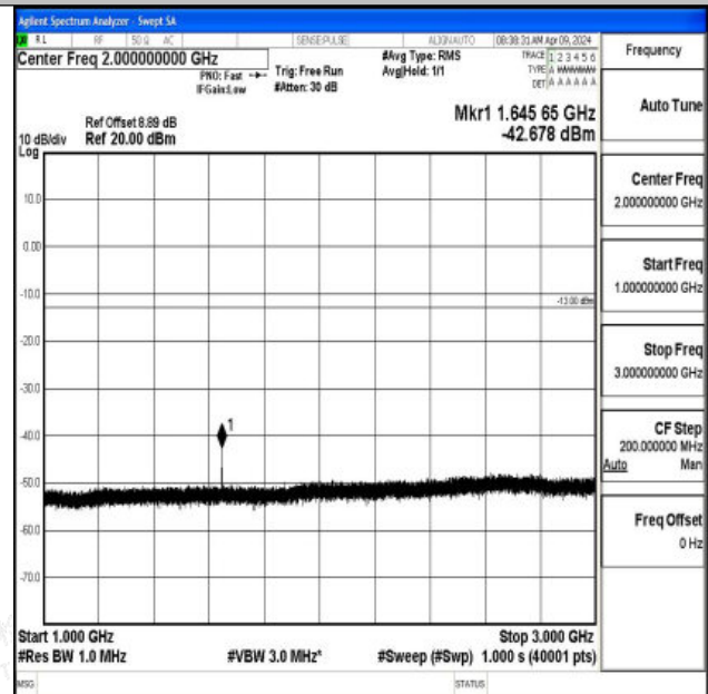
Band26_1.4MHz_QPSK_26783_1RB#0_1000~3000_1000~ 3000
