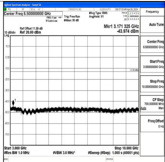
Band26_1.4MHz_16QAM_26697_1RB#0_3000~10000_300 0~10000
