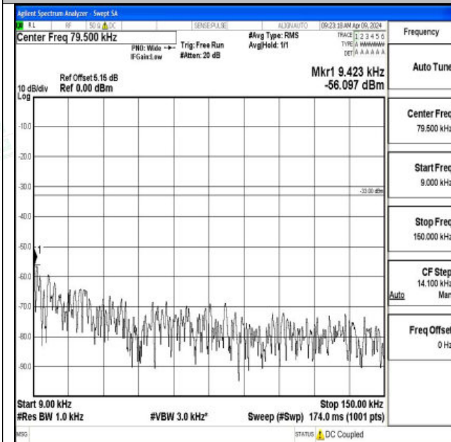
Band26_5MHz_QPSK_26740_1RB#0_0.009~0.15_0.009~0.15 0.15
