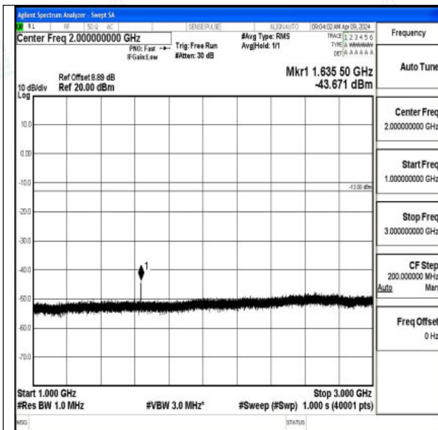
Band26_3MHz_16QAM_26740_1RB#0_1000~3000_1000 ~3000
