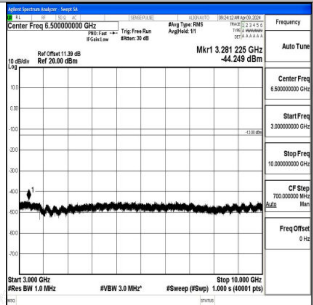
Band26_5MHz_16QAM_26740_1RB#0_3000~10000_3000~10000
