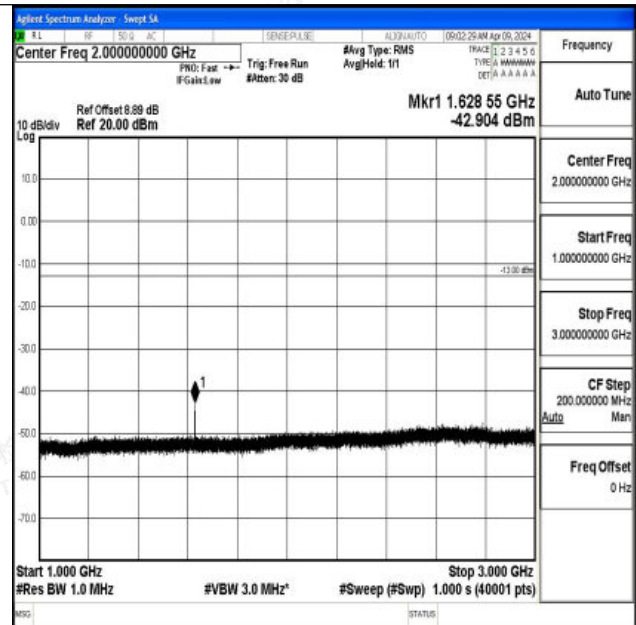
Band26_3MHz_QPSK_26705_1RB#0_1000~3000_1000~3000
