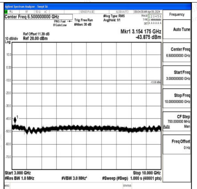
Band26_3MHz_16QAM_26740_1RB#0_3000~10000_3000 ~10000
