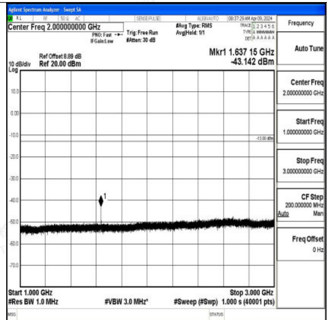
Band26_1.4MHz_QPSK_26740_1RB#0_1000~3000_1000~3000
