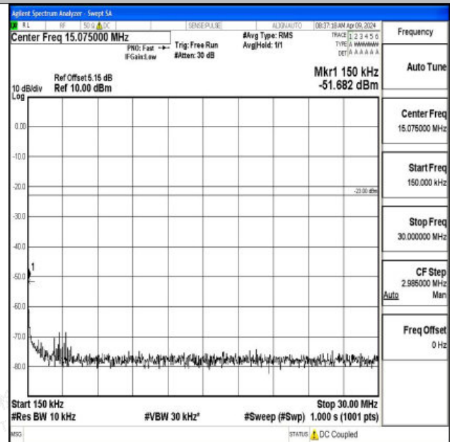
Band26_1.4MHz_QPSK_26740_1RB#0_0.15~30_0.15~30
