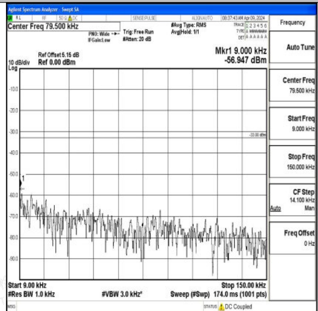
Band26_1.4MHz_16QAM_26740_1RB#0_0.009~0.15_0.009~0.15
