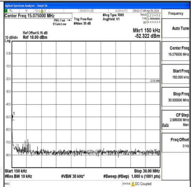
Band26_3MHz_QPSK_26705_1RB#0_0.15~30_0.15~30
