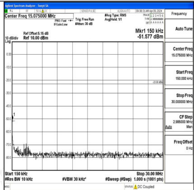
Band26_10MHz_QPSK_26740_1RB#0_0.15~30_0.15~30
