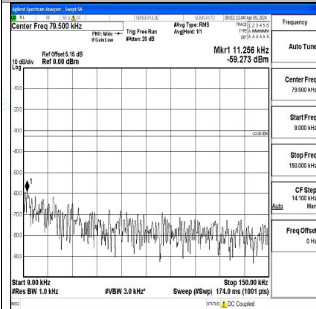
Band26_3MHz_QPSK_26705_1RB#0_0.009~0.15_0.009~0.15
