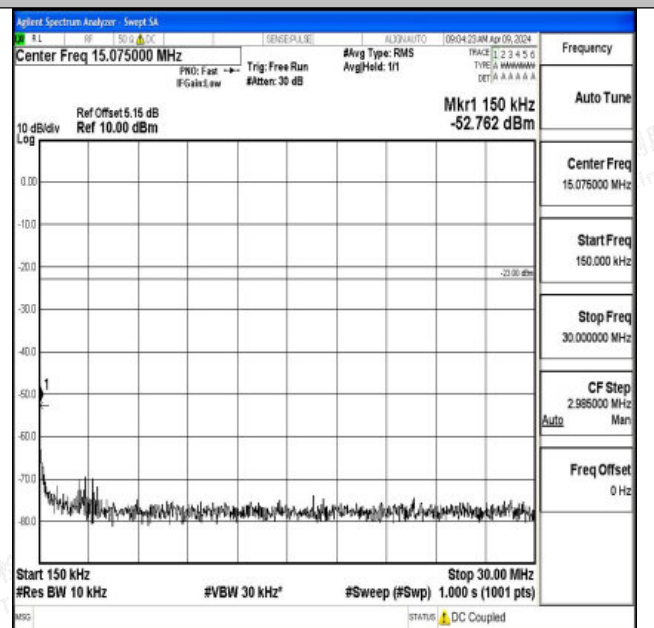
Band26_3MHz_QPSK_26775_1RB#0_0.15~30_0.15~30
