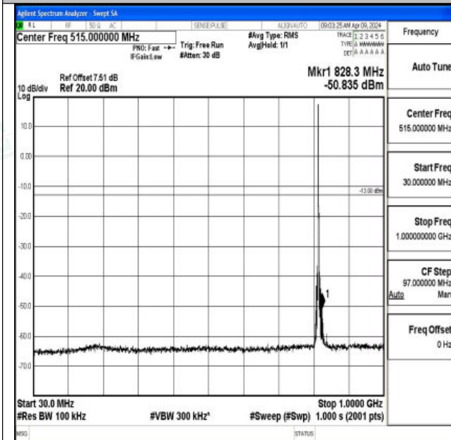
Band26_3MHz_QPSK_26740_1RB#0_30~1000_30~1000
