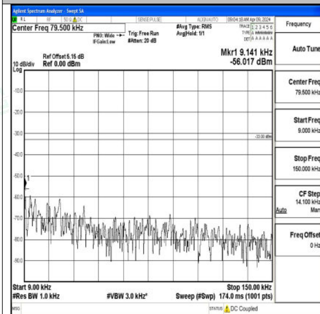
Band26_3MHz_QPSK_26775_1RB#0_0.009~0.15_0.009~0.15
