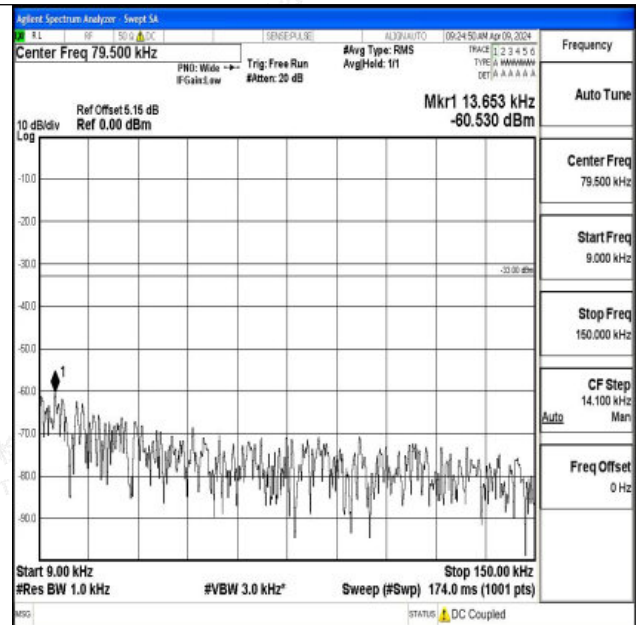
Band26_5MHz_16QAM_26765_1RB#0_0.009~0.15_0.009~0.15
