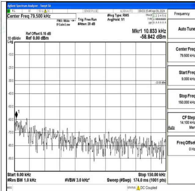
Band26_3MHz_QPSK_26740_1RB#0_0.009~0.15_0.009~0.15
