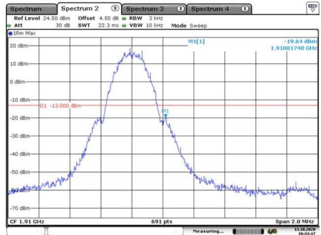
PCS 1900 Band, GSM, Right Band Edge
