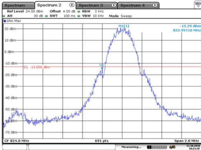
Cellular 850 Band, GSM, Left Band Edge
