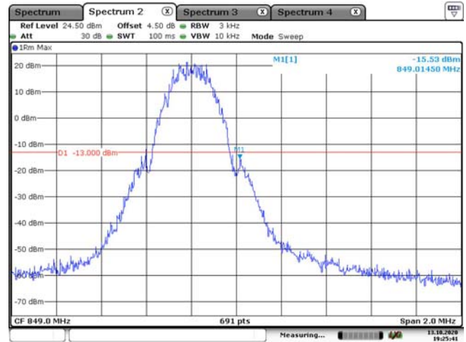
Cellular 850 Band, GSM, Right Band Edge
