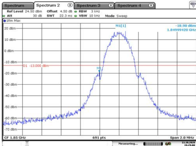
PCS 1900 Band, GSM, Left Band Edge
