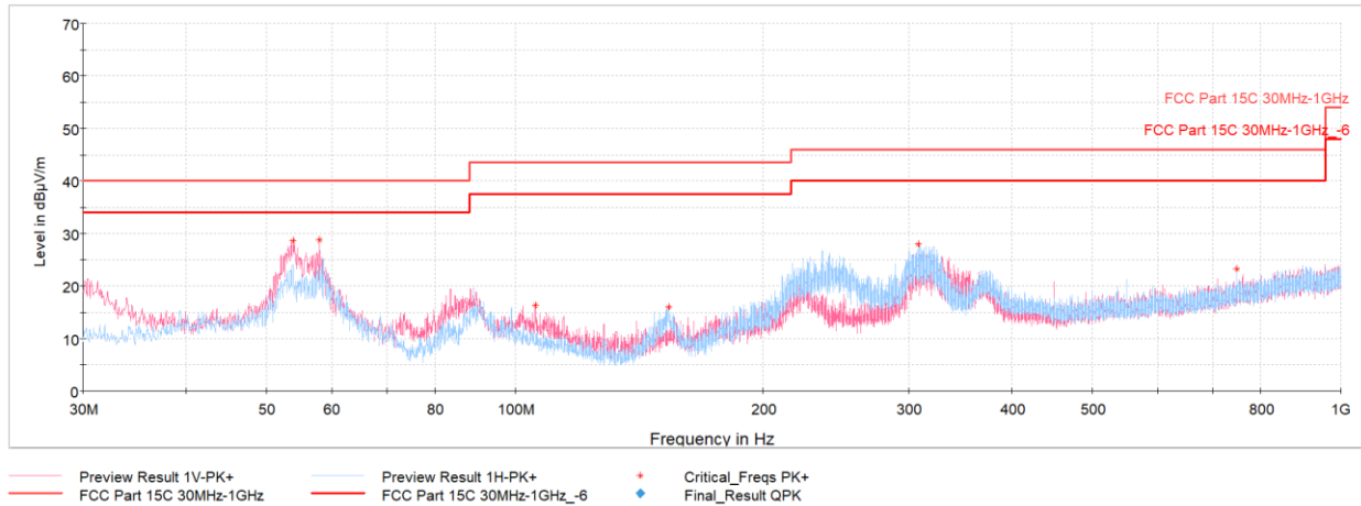
Plot 7-46. Radiated Spurious Emissions 30MHz-1GHz Antenna 4a (250kbps, ePA - Ch.25, with Laptop)
