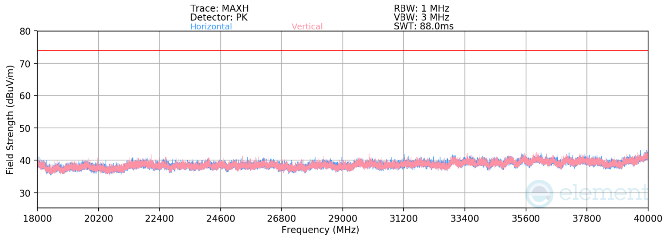
Plot 7-38. Radiated Spurious Emissions Above 18GHz Antenna 4a (802.15.4 ePA – Ch.25)
