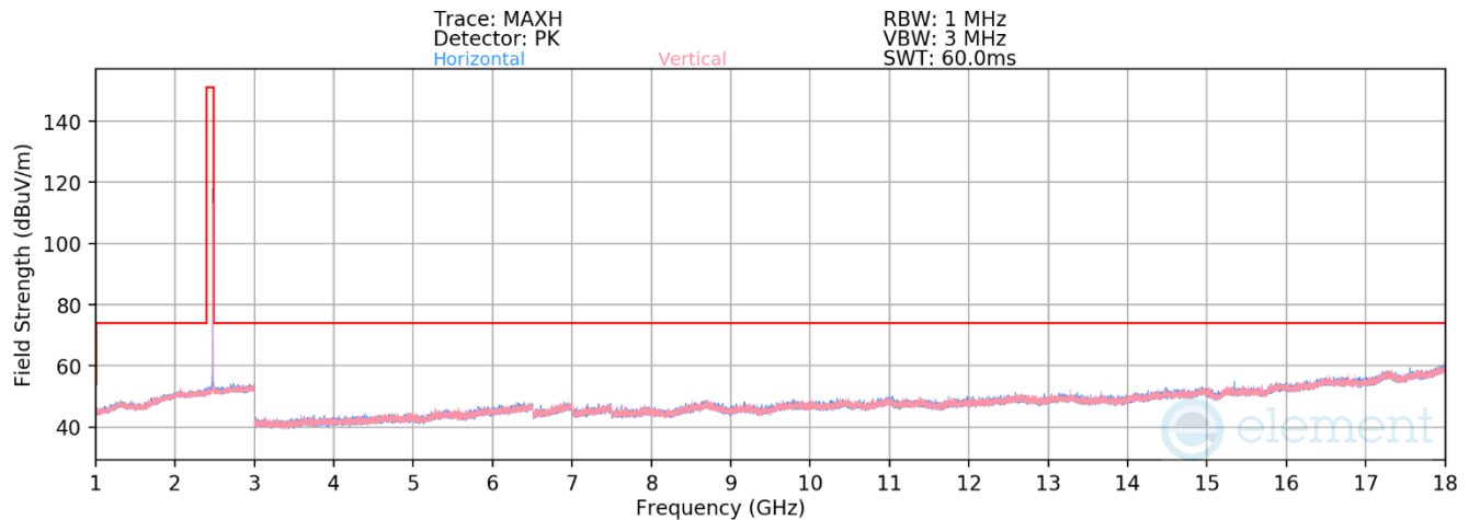
Plot 7-41. Radiated Spurious Emissions 1-18GHz Antenna 2a (802.15.4 ePA – Ch. 25)
