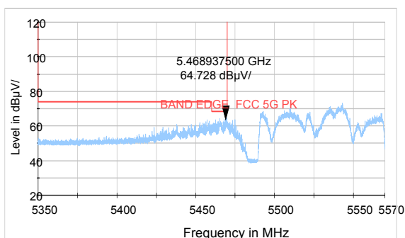
802.11ax HE80 -Channel 106: Peak
