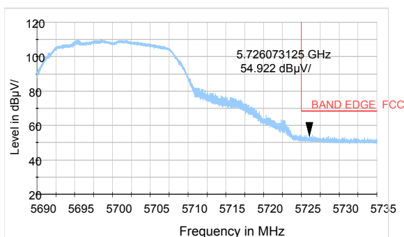
802.11a-Channel 140: Peak
