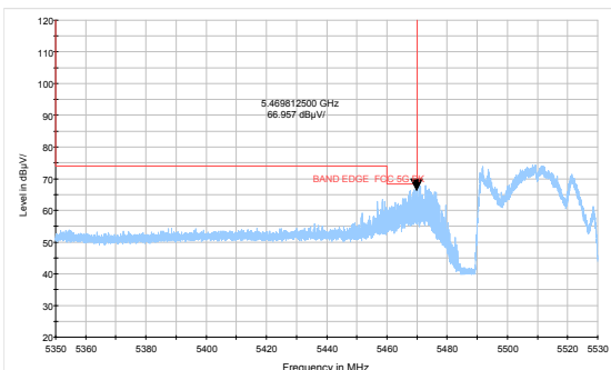
802.11ax HE40-Channel 102: Peak
