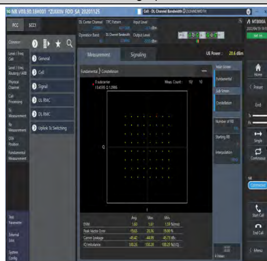
1-N66-PC3-15-20-M-4-DFT-64QAM-Out_Full-100 @0-Ant1-see graph-PASS
