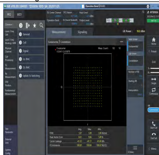
1-N66-PC3-15-40-M-5-DFT-256QAM-Outer_Full-216 @0-Ant1-see graph-PASS
