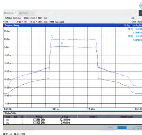
1-N66-PC3-15-40-M-2-CP-256QAM-Outer_Full-216 @0-Ant1-9.37-100%-0.00-9.37-PASS-≤13
