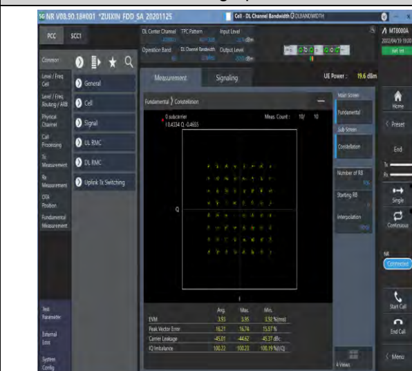
1-N66-PC3-15-20-M-8-CP-64QAM-Outer_Full-106@ 0-Ant1-see graph-PASS
