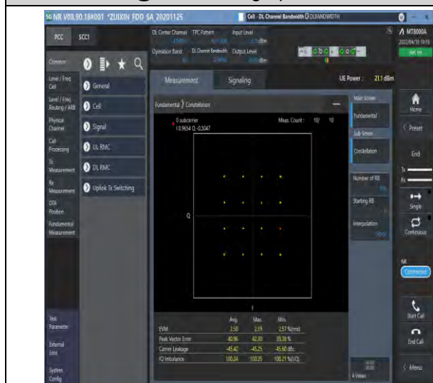
1-N66-PC3-15-20-M-3-DFT-16QAM-Out_Full-100 @0-Ant1-see graph-PASS
