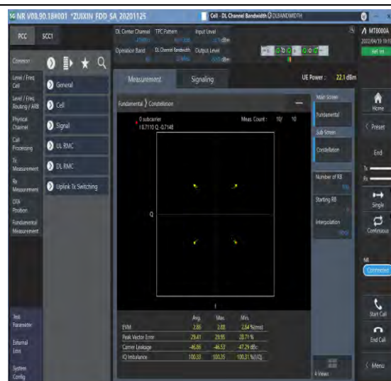
1-N66-PC3-15-20-M-2-DFT-QPSK-Out_Full-100@ 0-Ant1-see graph-PASS
