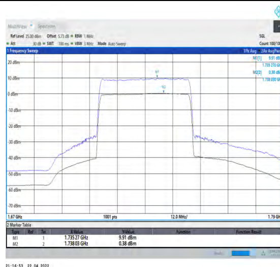
1-N66-PC3-15-40-L-2-CP-256QAM-Outer_Full-216 @0-Ant1-9.53-100%-0.00-9.53-PASS-≤13
