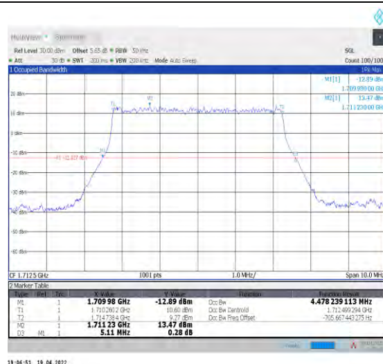
1-N66-PC3-15-5-L-2-DFT-PI2BPSK-Outer_Full-25@ 0-Ant1-4.478-5.110-≤5-PASS
