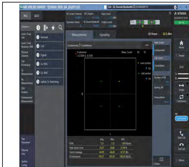
1-N66-PC3-15-20-M-1-DFT-PI2BPSK-Out_Full-10 0@0-Ant1-see graph-PASS
