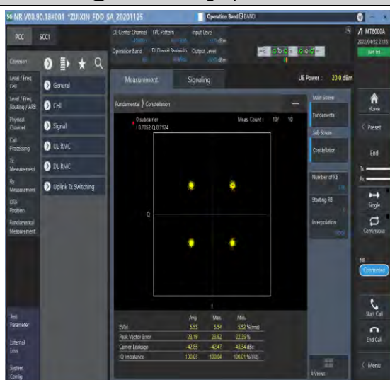
1-N66-PC3-15-40-M-6-CP-QPSK-Outer_Full-216@0 -Ant1-see graph-PASS
