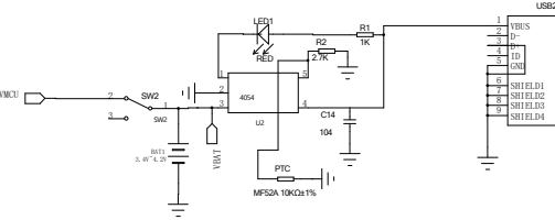
Charging Circuit
