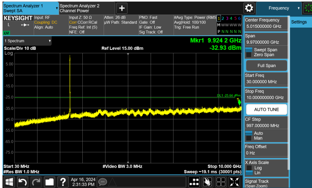
Plot 7-72. Conducted Spurious Plot SISO ANT2 (802.11be OFDMA – 242 Tones – Ch. 11)
