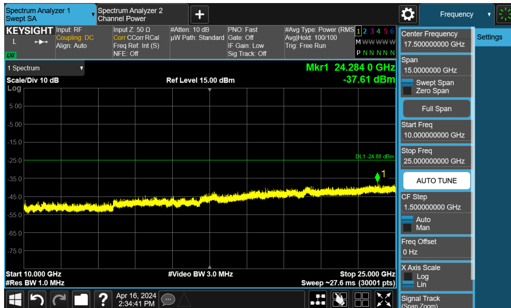
Plot 7-71. Conducted Spurious Plot SISO ANT2 (802.11be OFDMA – 242 Tones – Ch. 6)
