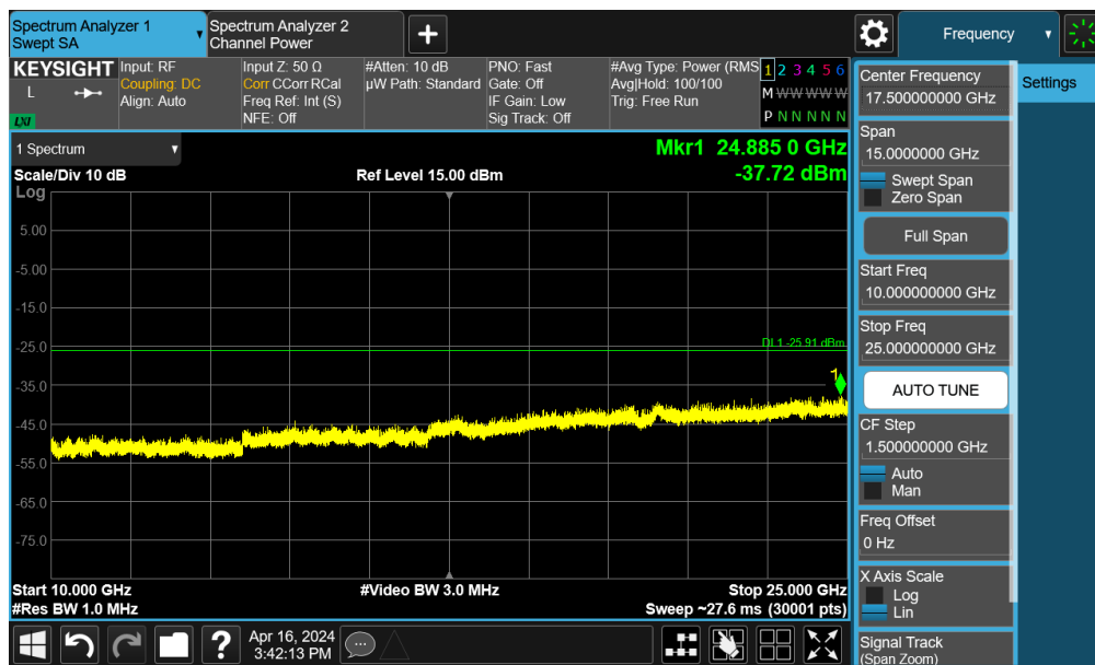
Plot 7-85. Conducted Spurious Plot MIMO ANT1 (802.11be OFDMA – 242 Tones – Ch. 11)
