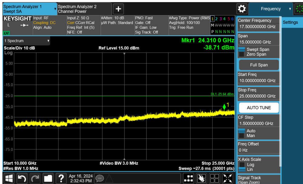
Plot 7-73. Conducted Spurious Plot SISO ANT2 (802.11be OFDMA – 242 Tones – Ch. 11)
