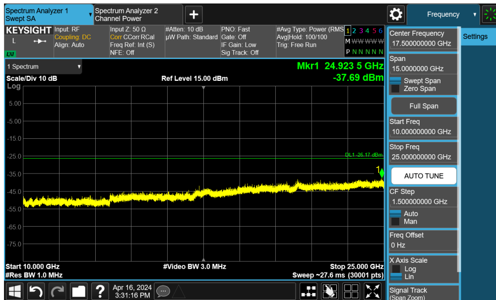
Plot 7-93. Conducted Spurious Plot MIMO ANT2 (802.11be OFDMA – 242 Tones – Ch. 1)
