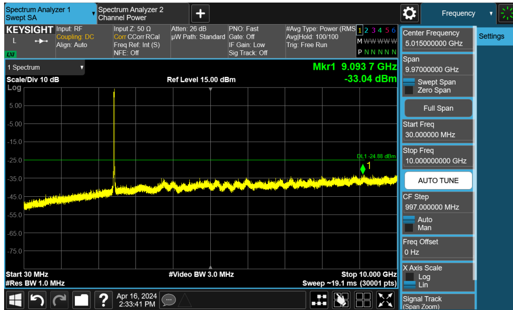
Plot 7-70. Conducted Spurious Plot SISO ANT2 (802.11be OFDMA – 242 Tones – Ch. 6)
