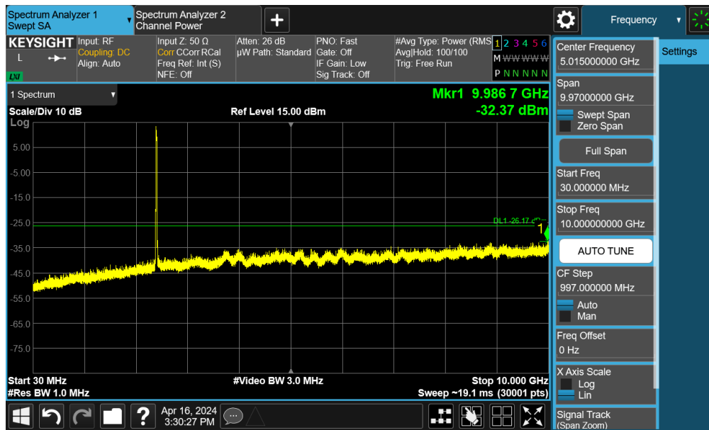
Plot 7-92. Conducted Spurious Plot MIMO ANT2 (802.11be OFDMA – 242 Tones – Ch. 1)
