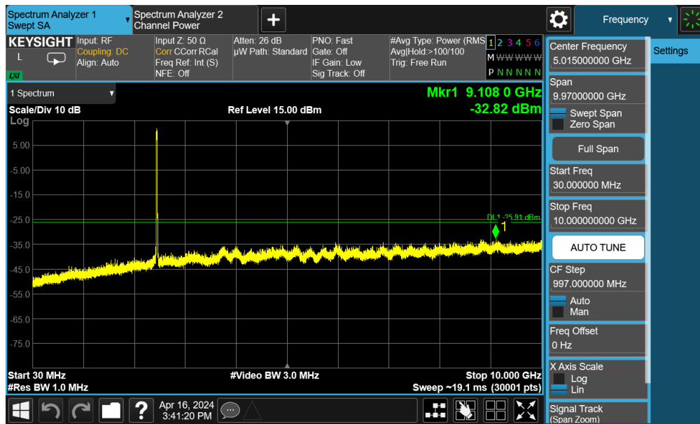
Plot 7-84. Conducted Spurious Plot MIMO ANT1 (802.11be OFDMA – 242 Tones – Ch. 11)
