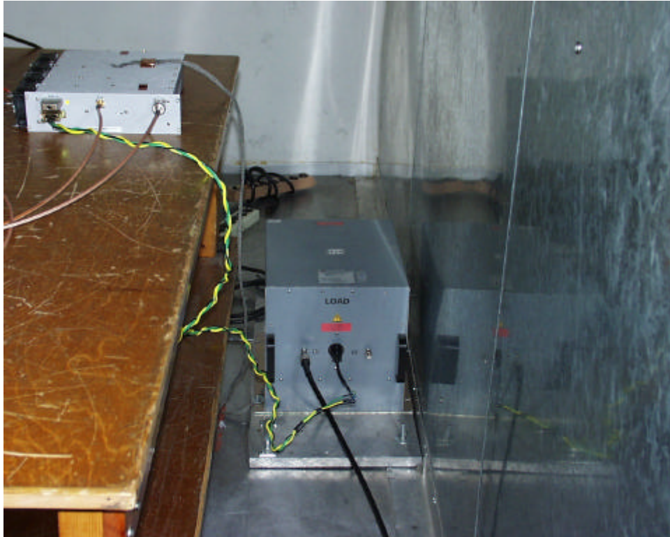
Part15 back view Conducted Emission Setup
