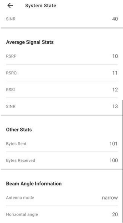
Figure 29 System state screen with Beam Angle information for a Nokia FastMile 4G Receiver managed by the Nokia Altiplano FastMile Controller
