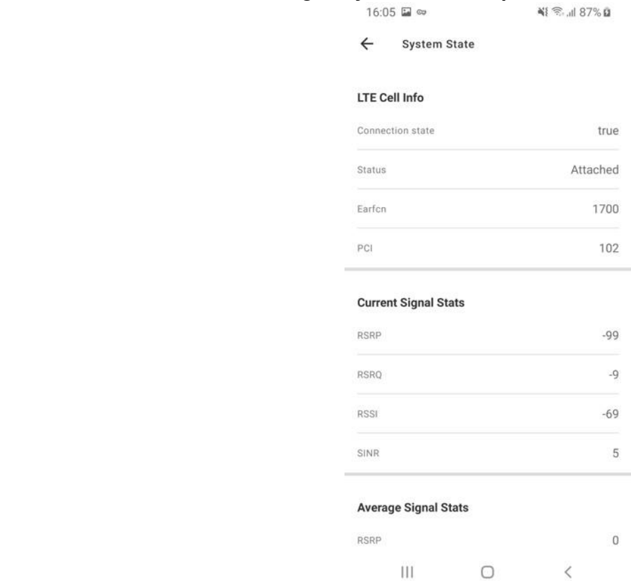
Figure 28 System state screen example for a Nokia FastMile 4G Receiver managed by the Nokia Altiplano FastMile Controller
