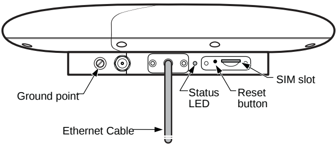
Figure 11 Location of physical interfaces on the Compact mono-band and ABA models of the
