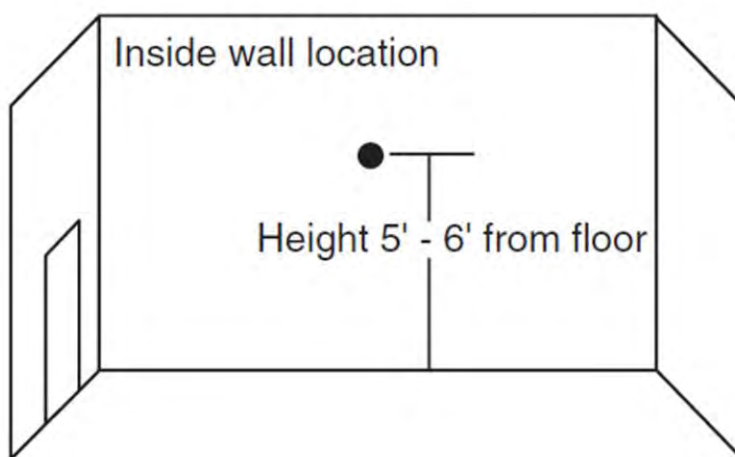
Figure 62: Recommended CO Sensor Mounting Location
