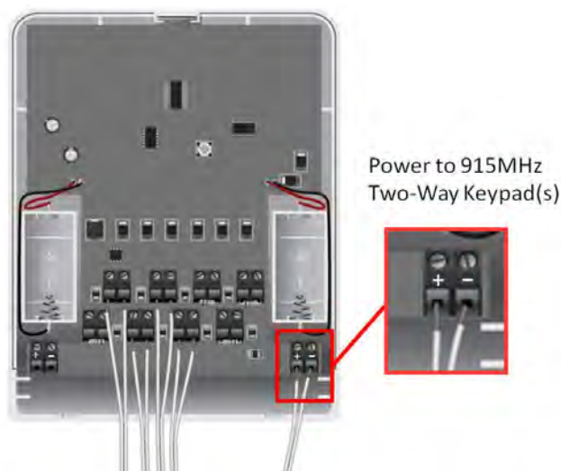
Figure 87: Conversion Kit (Model SW-ATT-TAKRF) - Powering 915 MHz Two-Way Keypad
