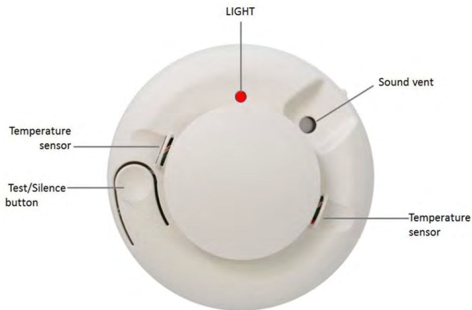
Figure 53: Smoke Sensor (Model SW-ATT-SMKT)
