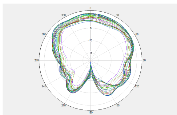
PHI=90 2D
