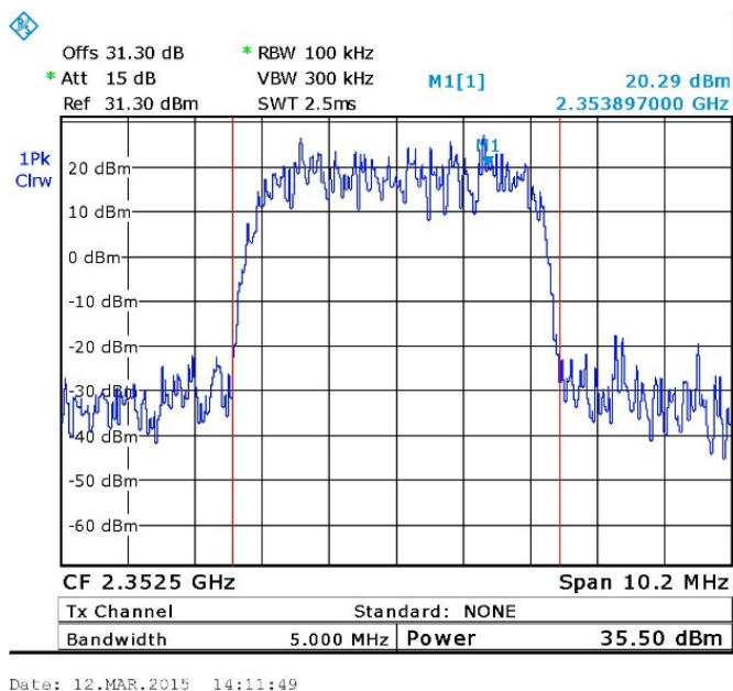
Figure 11. — 2352.5 MHz – W-CDMA
