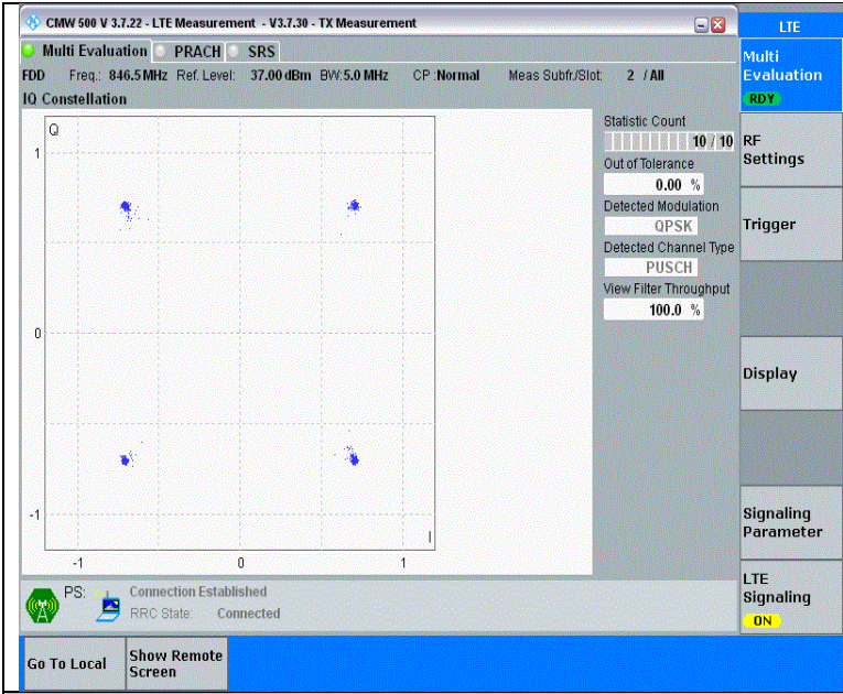
Band5-5MHz-QPSK-20625-25RB#0-PASS
