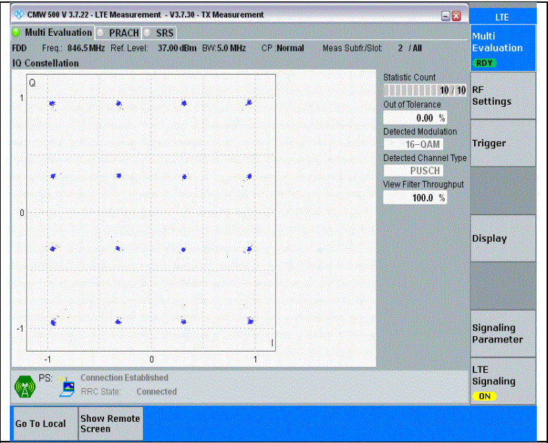
Band5-5MHz-16QAM-20625-25RB#0-PASS
