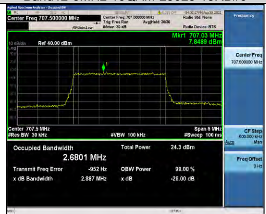
Band12-3MHz-16QAM-23095-15RB#0
