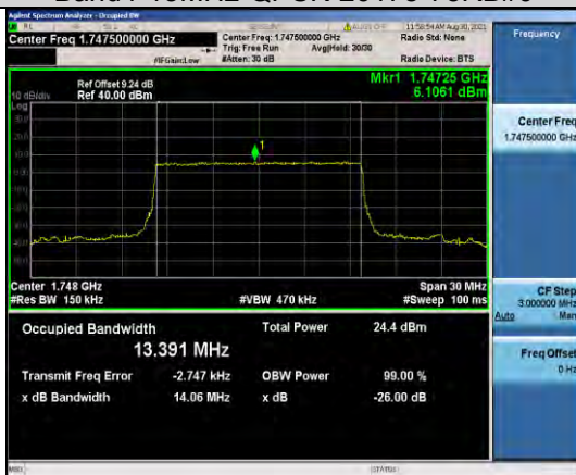
Band4-15MHz-QPSK-20325-75RB#0
