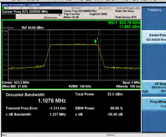
Band26-1.4MHz-16QAM-26783-6RB#0
