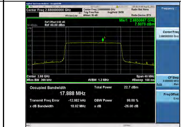
Band41-20MHz-16QAM-41490-100RB#0
