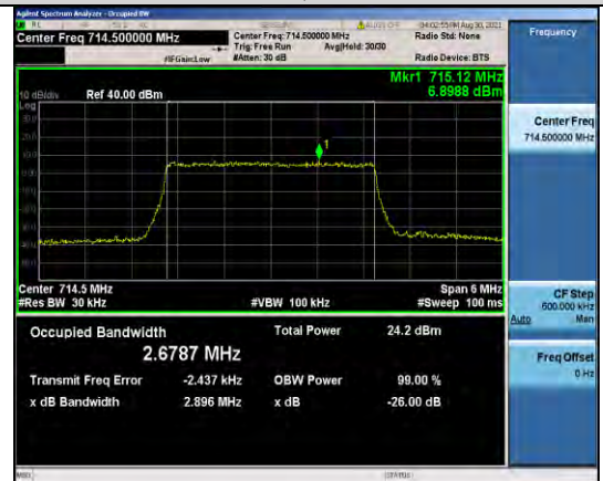
Band12-3MHz-16QAM-23165-15RB#0
