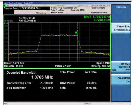
Band66-1.4MHz-16QAM-132665-6RB#0
