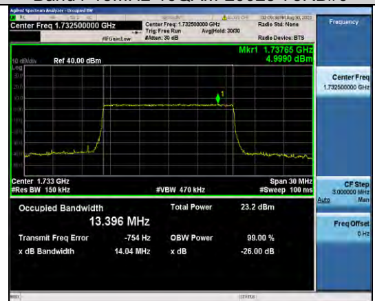
Band4-15MHz-16QAM-20175-75RB#0
