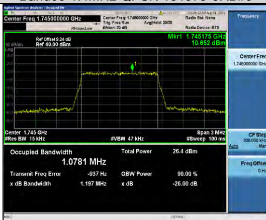
Band66-1.4MHz-QPSK-132322-6RB#0
