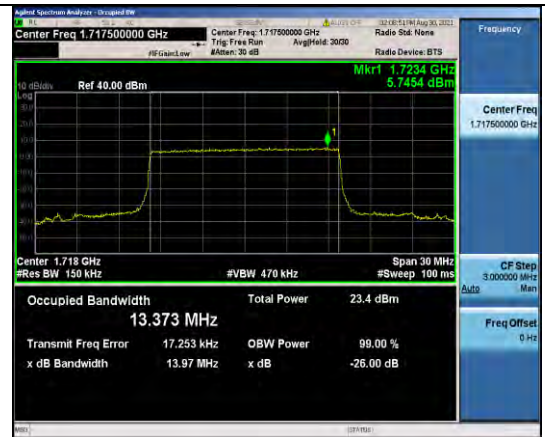
Band4-15MHz-16QAM-20025-75RB#0
