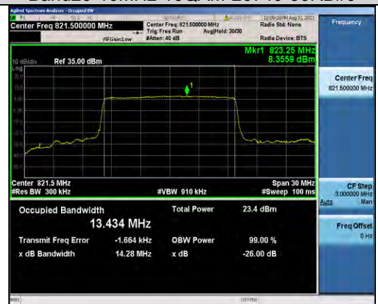
Band26-15MHz-QPSK-26765-75RB#0
