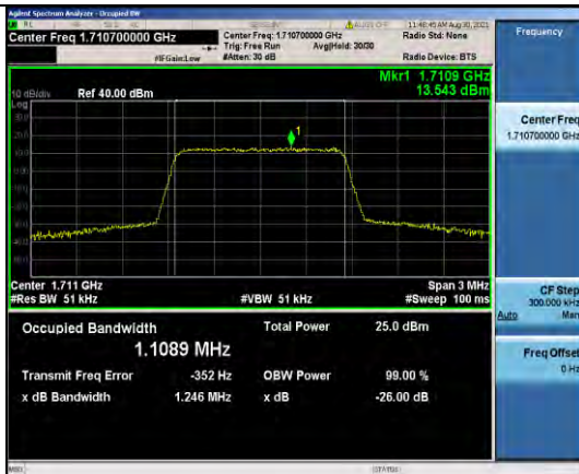
Band4-1.4MHz-QPSK-19957-6RB#0
