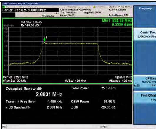
Band5-3MHz-QPSK-20415-15RB#0
