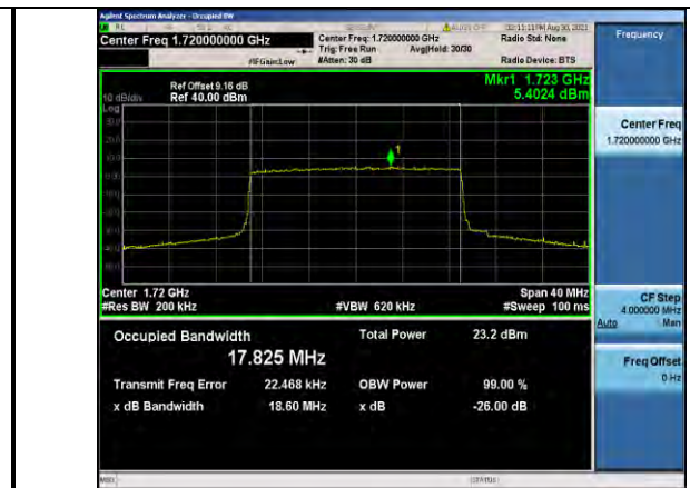
Band4-20MHz-16QAM-20050-100RB#0
