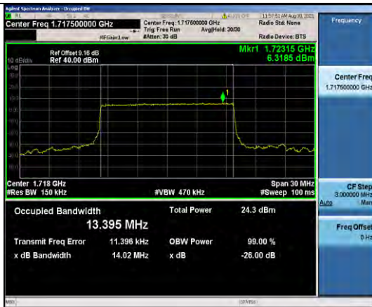
Band4-15MHz-QPSK-20025-75RB#0
