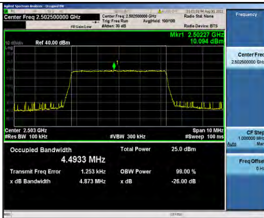
Band7-5MHz-QPSK-20775-25RB#0
