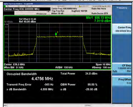
Band5-5MHz-16QAM-20525-25RB#0
