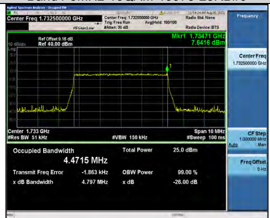
Band4-5MHz-16QAM-20175-25RB#0
