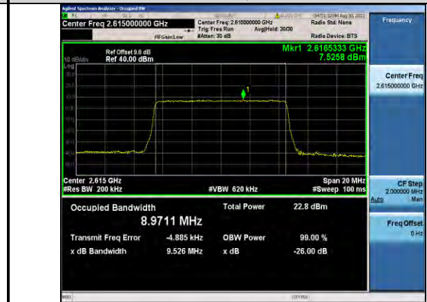
Band38-10MHz-16QAM-38200-50RB#0
