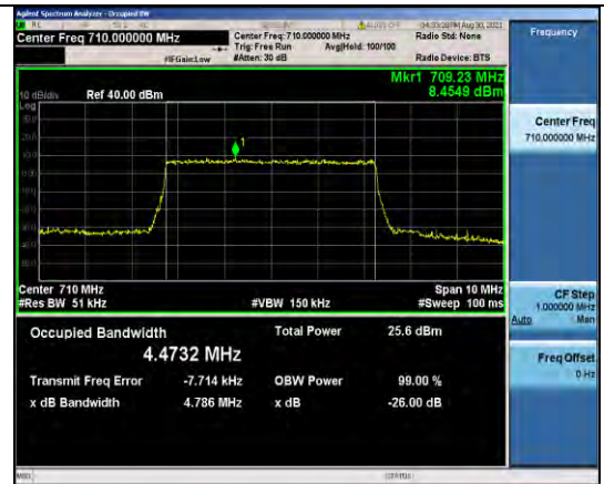
Band17-5MHz-QPSK-23790-25RB#0
