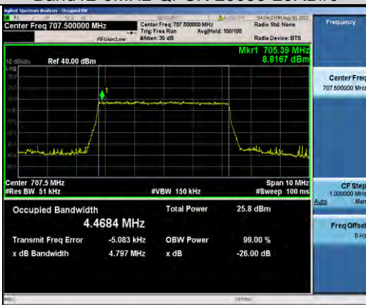
Band12-5MHz-QPSK-23095-25RB#0
