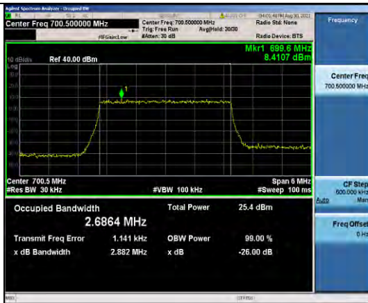
Band12-3MHz-QPSK-23025-15RB#0
