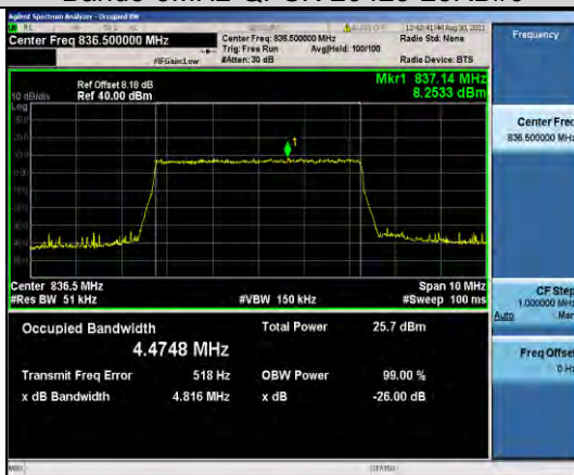
Band5-5MHz-QPSK-20525-25RB#0
