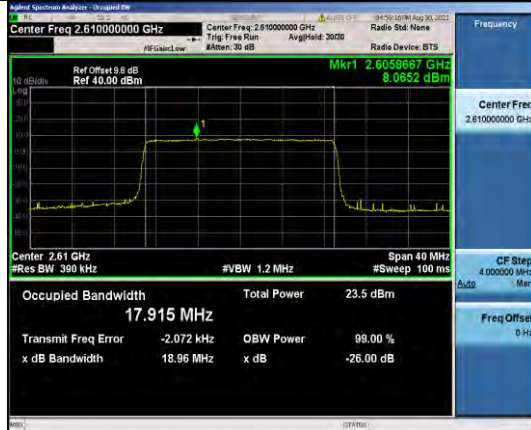
Band38-20MHz-QPSK-38150-100RB#0
