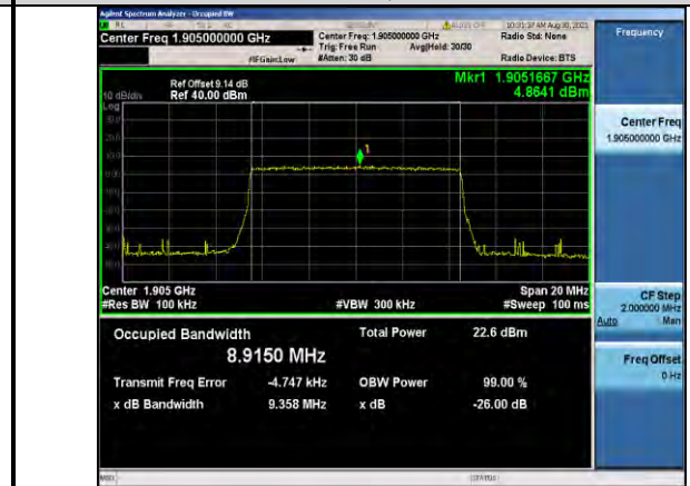
Band2-10MHz-16QAM-19150-50RB#0
