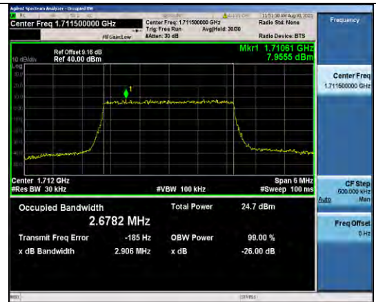
Band4-3MHz-16QAM-19965-15RB#0
