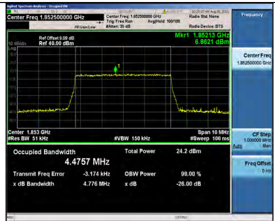
Band2-5MHz-16QAM-18625-25RB#0
