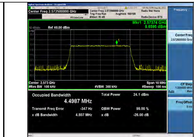
Band38-5MHz-16QAM-37775-25RB#0
