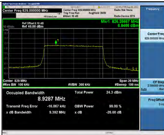
Band5-10MHz-QPSK-20450-50RB#0
