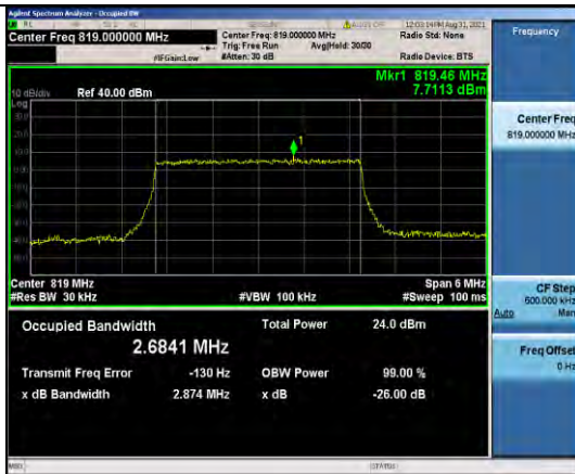
Band26-3MHz-16QAM-26740-15RB#0
