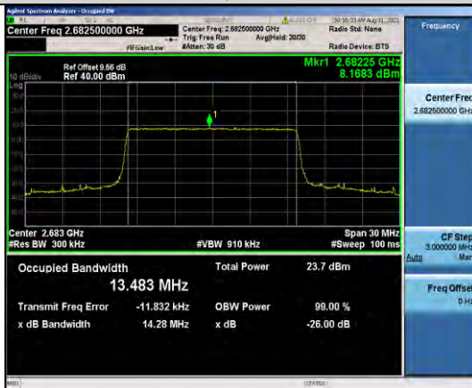
Band41-15MHz-QPSK-41515-75RB#0
