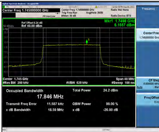
Band4-20MHz-QPSK-20300-100RB#0
