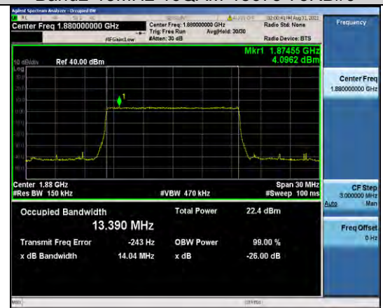
Band2-15MHz-16QAM-18900-75RB#0
