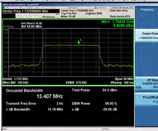
Band4-15MHz-QPSK-20175-75RB#0
