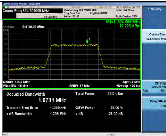
Band5-1.4MHz-QPSK-20407-6RB#0
