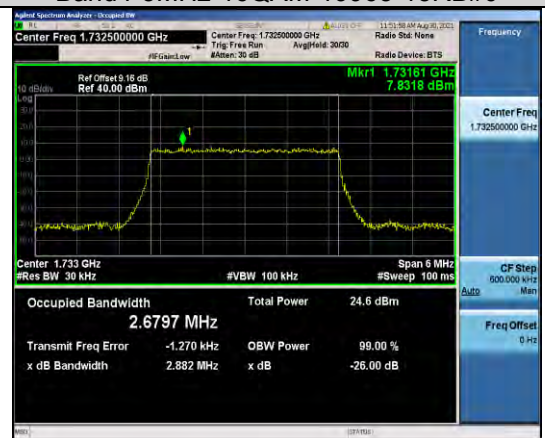
Band4-3MHz-16QAM-20175-15RB#0
