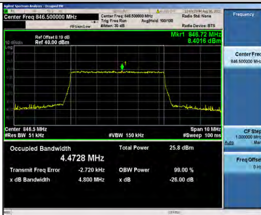
Band5-5MHz-QPSK-20625-25RB#0
