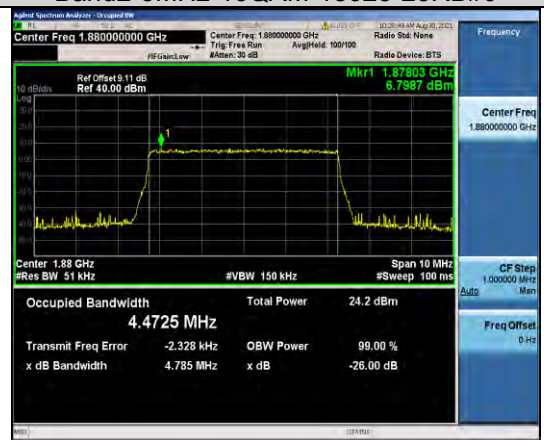
Band2-5MHz-16QAM-18900-25RB#0
