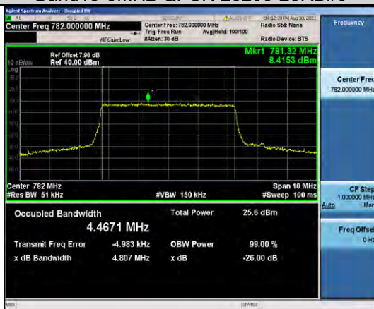
Band13-5MHz-QPSK-23230-25RB#0
