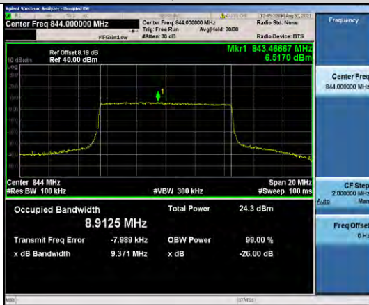
Band5-10MHz-QPSK-20600-50RB#0
