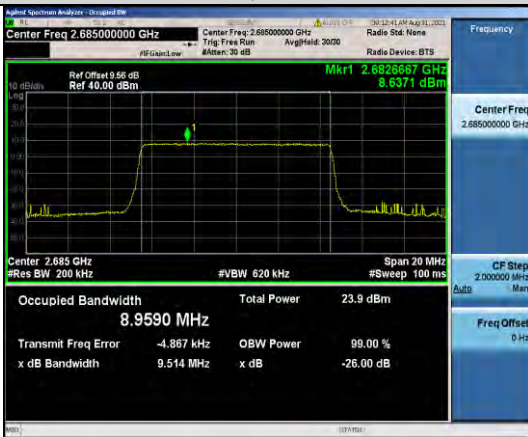
Band41-10MHz-QPSK-41540-50RB#0
