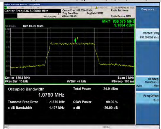
Band5-1.4MHz-16QAM-20525-6RB#0
