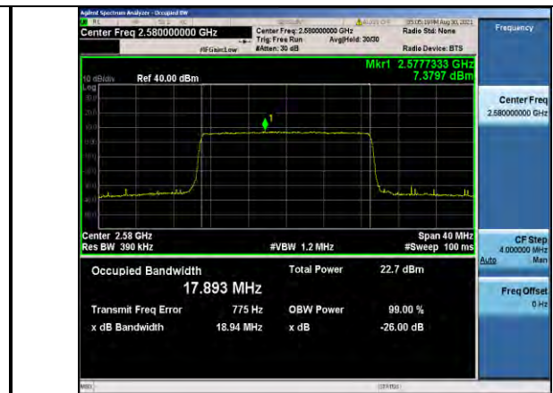
Band38-20MHz-16QAM-37850-100RB#0
