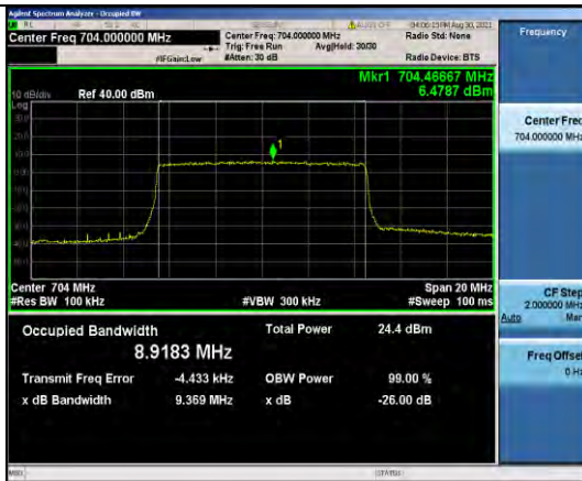
Band12-10MHz-QPSK-23060-50RB#0
