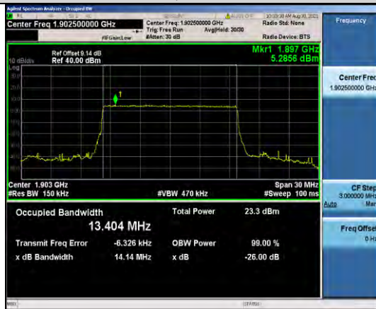
Band2-15MHz-QPSK-19125-75RB#0
