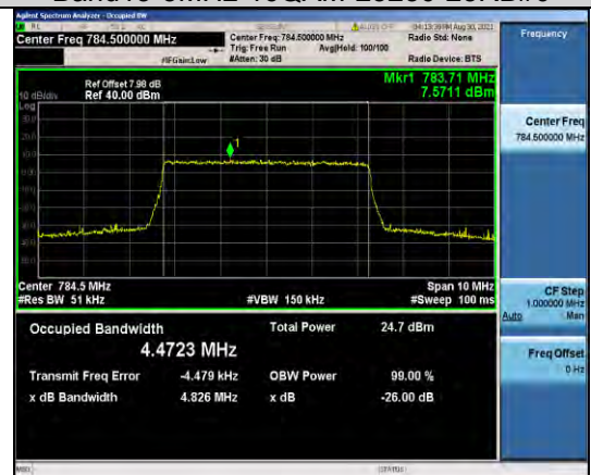
Band13-5MHz-16QAM-23255-25RB#0
