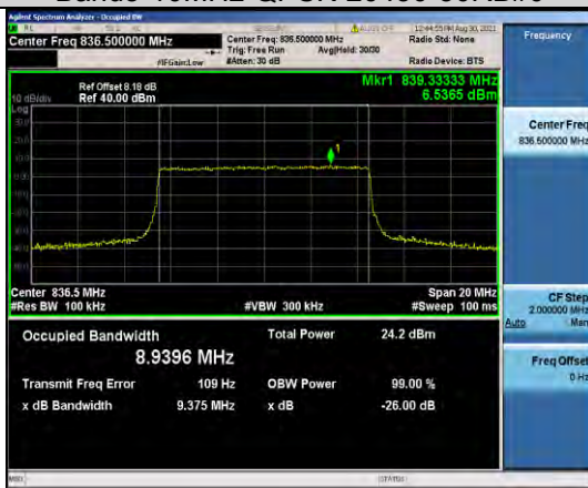
Band5-10MHz-QPSK-20525-50RB#0
