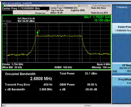
Band4-3MHz-QPSK-20385-15RB#0
