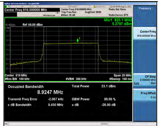
Band26-10MHz-16QAM-26740-50RB#0
