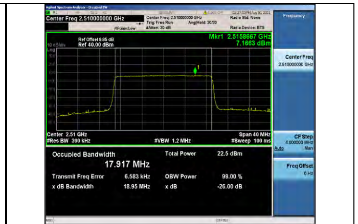
Band7-20MHz-16QAM-20850-100RB#0
