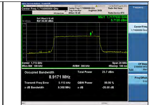
Band4-10MHz-16QAM-20000-50RB#0
