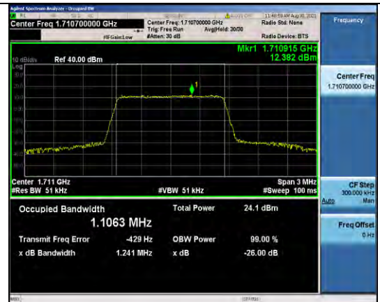
Band4-1.4MHz-16QAM-19957-6RB#0
