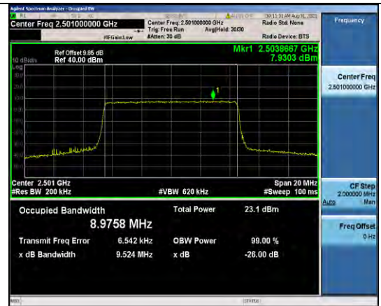
Band41-10MHz-16QAM-39700-50RB#0
