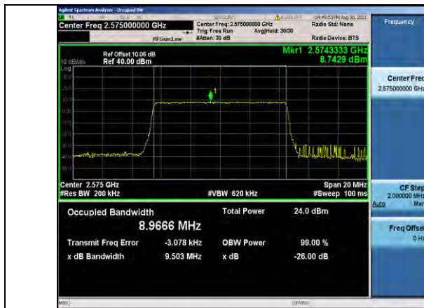
Band38-10MHz-QPSK-37800-50RB#0
