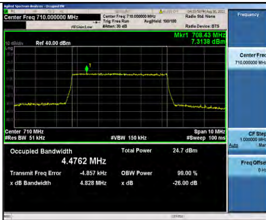
Band17-5MHz-16QAM-23790-25RB#0
