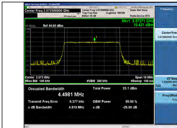
Band38-5MHz-QPSK-37775-25RB#0
