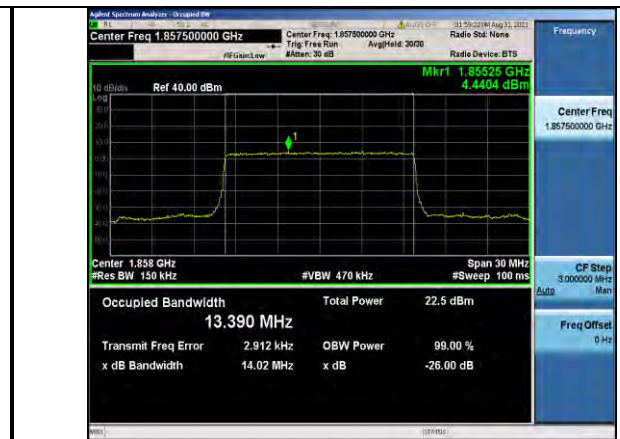
Band2-15MHz-16QAM-18675-75RB#0
