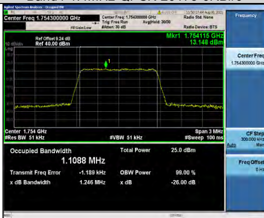
Band4-1.4MHz-QPSK-20393-6RB#0
