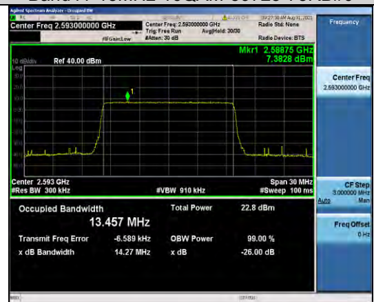
Band41-15MHz-16QAM-40620-75RB#0
