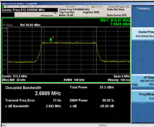
Band26-3MHz-QPSK-26705-15RB#0
