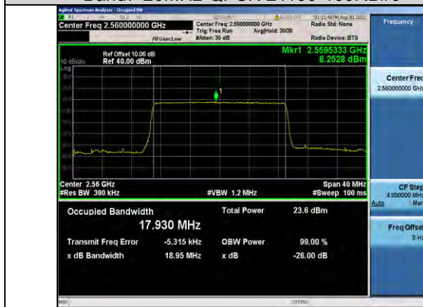
Band7-20MHz-QPSK-21350-100RB#0
