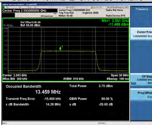
Band41-15MHz-QPSK-40620-75RB#0
