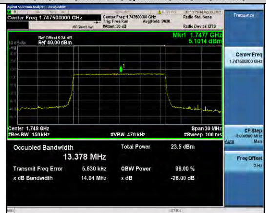
Band4-15MHz-16QAM-20325-75RB#0
