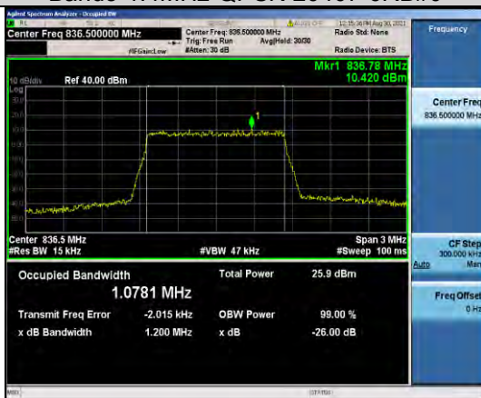
Band5-1.4MHz-QPSK-20525-6RB#0
