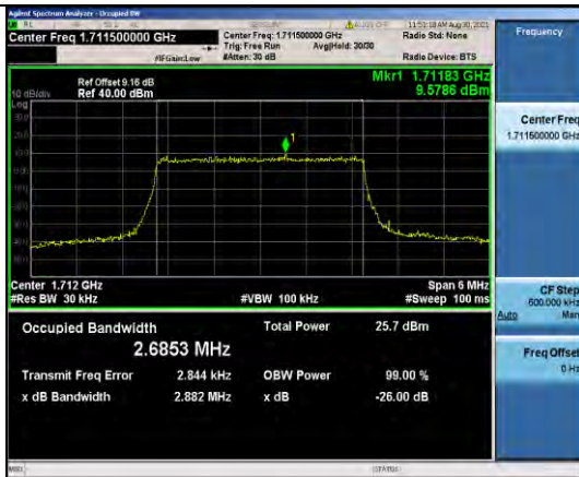
Band4-3MHz-QPSK-19965-15RB#0
