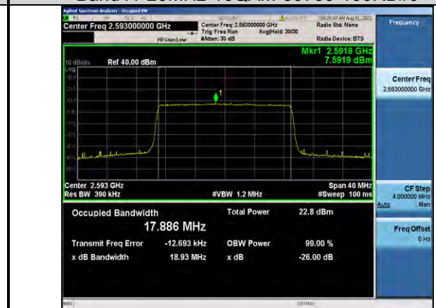
Band41-20MHz-16QAM-40620-100RB#0
