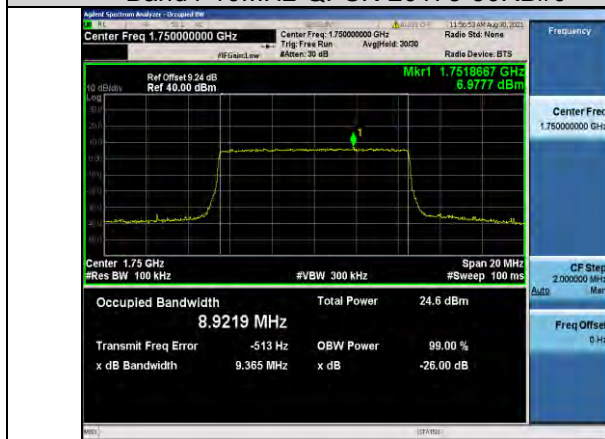
Band4-10MHz-QPSK-20350-50RB#0
