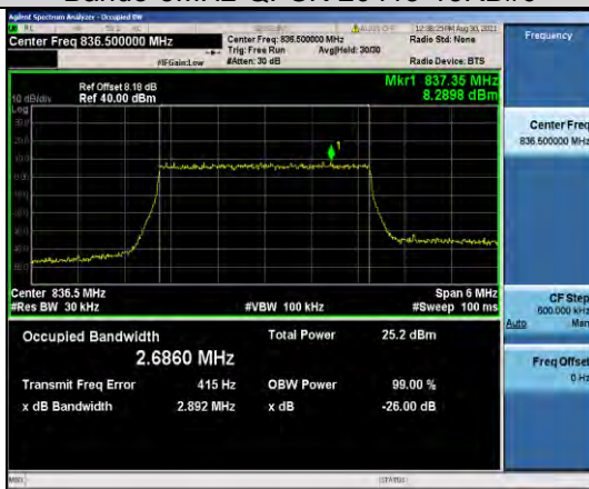
Band5-3MHz-QPSK-20525-15RB#0
