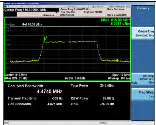
Band26-5MHz-QPSK-26740-25RB#0
