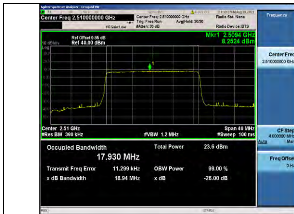
Band7-20MHz-QPSK-20850-100RB#0
