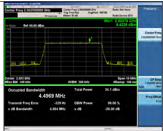
Band7-5MHz-16QAM-20775-25RB#0
