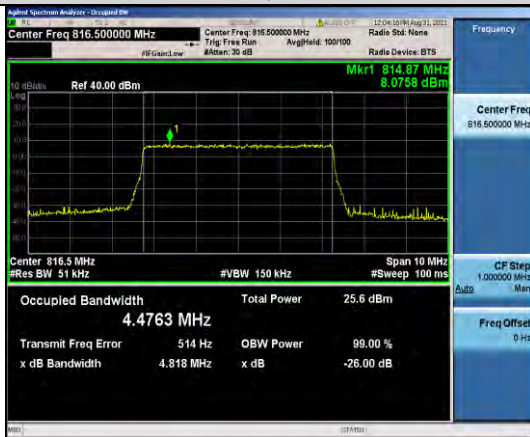
Band26-5MHz-QPSK-26715-25RB#0
