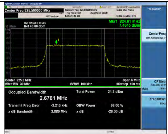
Band5-3MHz-16QAM-20415-15RB#0
