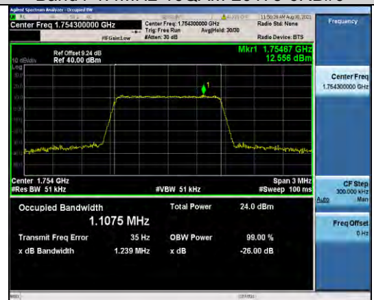
Band4-1.4MHz-16QAM-20393-6RB#0
