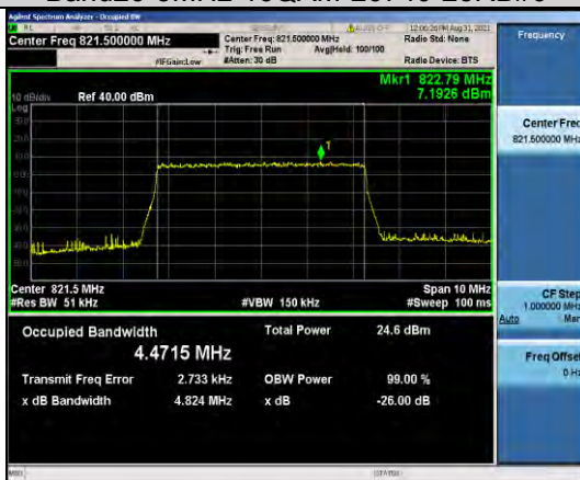
Band26-5MHz-16QAM-26765-25RB#0
