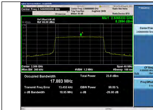
Band41-20MHz-QPSK-39750-100RB#0
