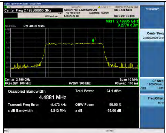
Band41-5MHz-16QAM-39675-25RB#0
