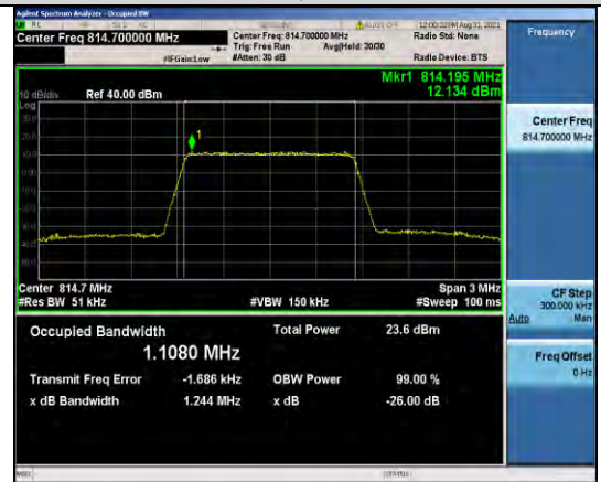
Band26-1.4MHz-16QAM-26697-6RB#0
