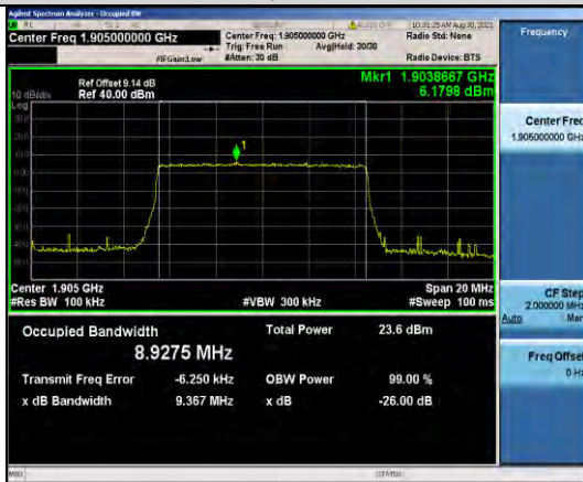
Band2-10MHz-QPSK-19150-50RB#0
