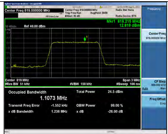
Band26-1.4MHz-QPSK-26740-6RB#0
