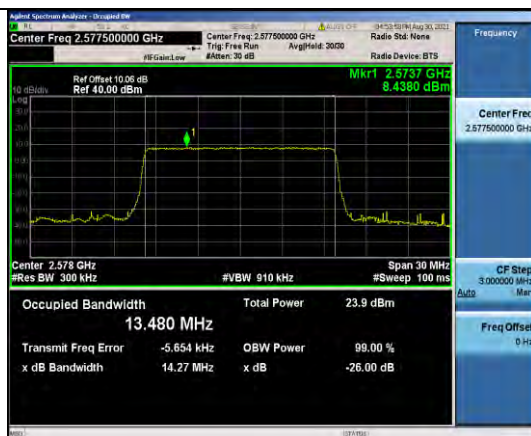
Band38-15MHz-QPSK-37825-75RB#0
