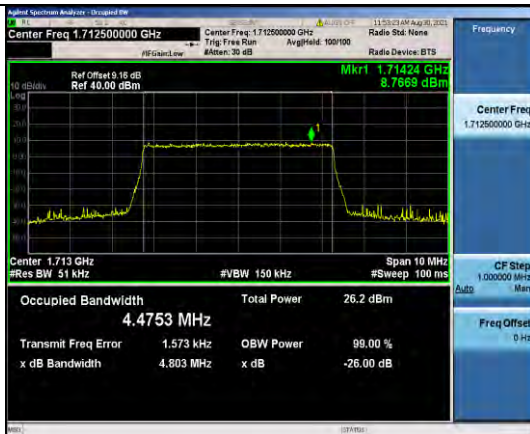
Band4-5MHz-QPSK-19975-25RB#0
