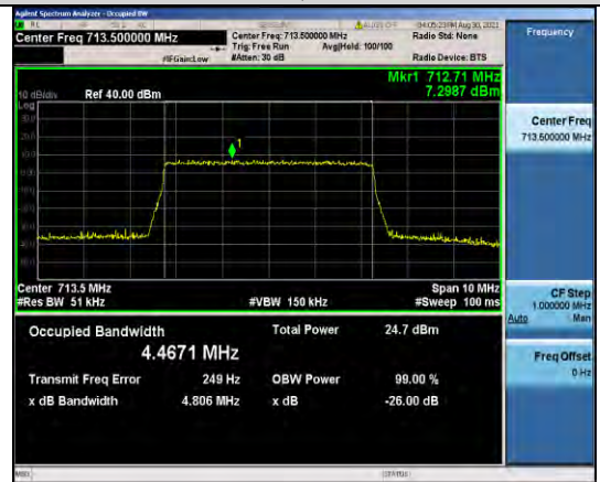
Band12-5MHz-16QAM-23155-25RB#0
