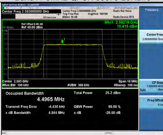
Band41-5MHz-QPSK-40620-25RB#0
