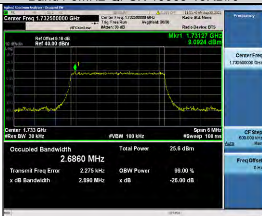
Band4-3MHz-QPSK-20175-15RB#0
