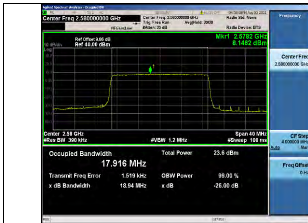
Band38-20MHz-QPSK-37850-100RB#0
