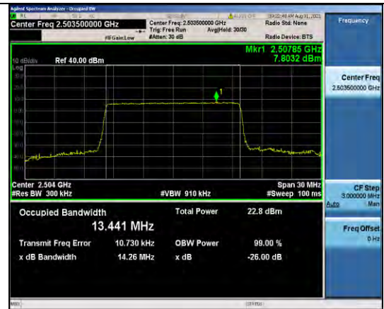
Band41-15MHz-16QAM-39725-75RB#0
