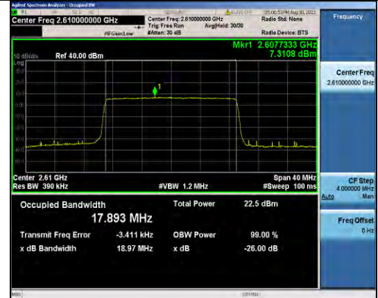
Band38-20MHz-16QAM-38150-100RB#0
