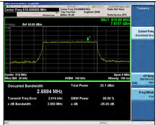
Band26-3MHz-QPSK-26740-15RB#0
