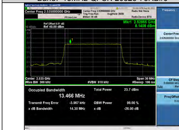
Band7-15MHz-QPSK-21100-75RB#0
