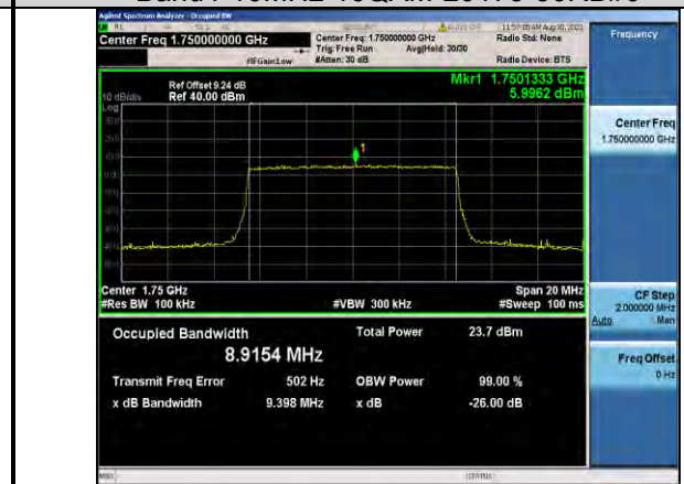
Band4-10MHz-16QAM-20350-50RB#0
