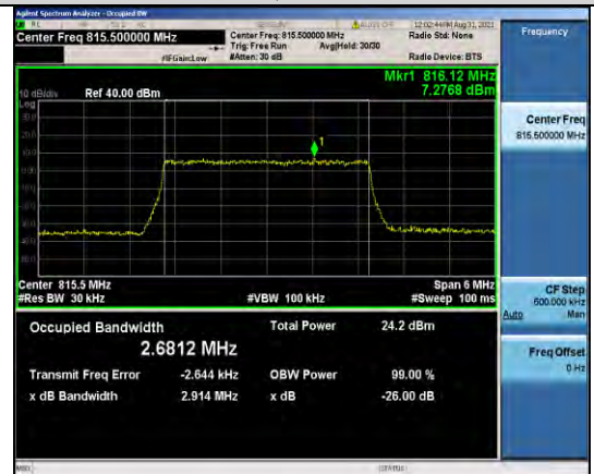
Band26-3MHz-16QAM-26705-15RB#0
