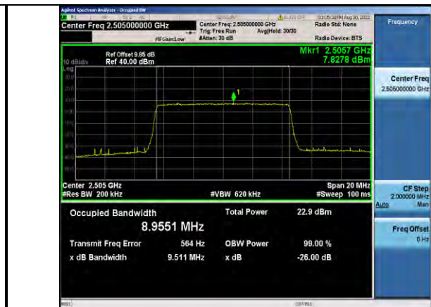
Band7-10MHz-16QAM-20800-50RB#0
