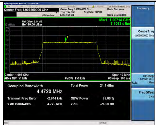
Band2-5MHz-16QAM-19175-25RB#0
