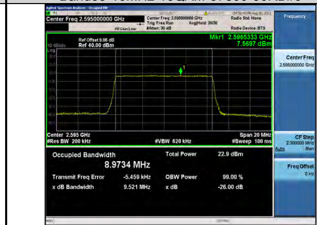
Band38-10MHz-16QAM-38000-50RB#0
