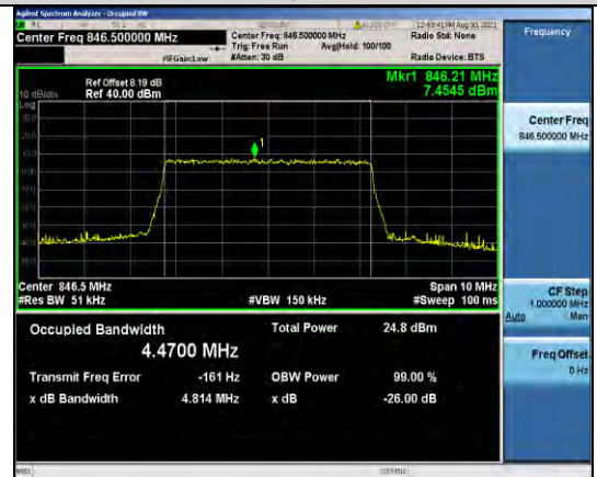
Band5-5MHz-16QAM-20625-25RB#0
