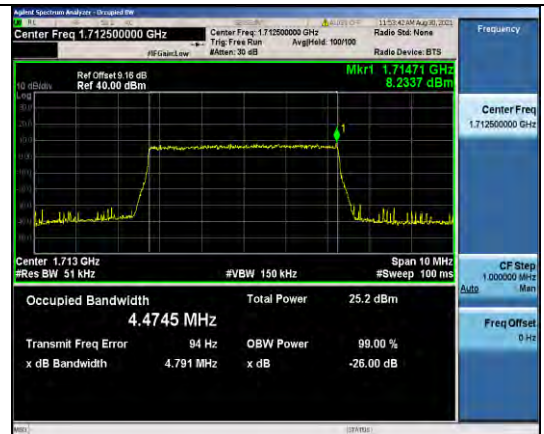
Band4-5MHz-16QAM-19975-25RB#0
