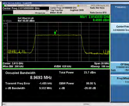
Band38-10MHz-QPSK-38200-50RB#0
