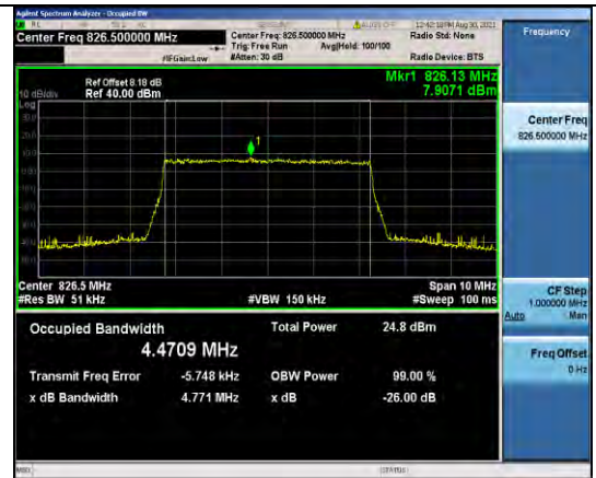
Band5-5MHz-16QAM-20425-25RB#0
