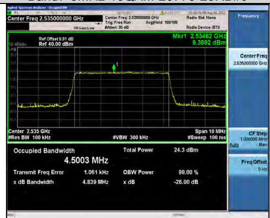
Band7-5MHz-16QAM-21100-25RB#0
