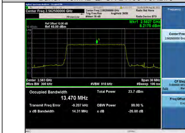
Band7-15MHz-QPSK-21375-75RB#0
