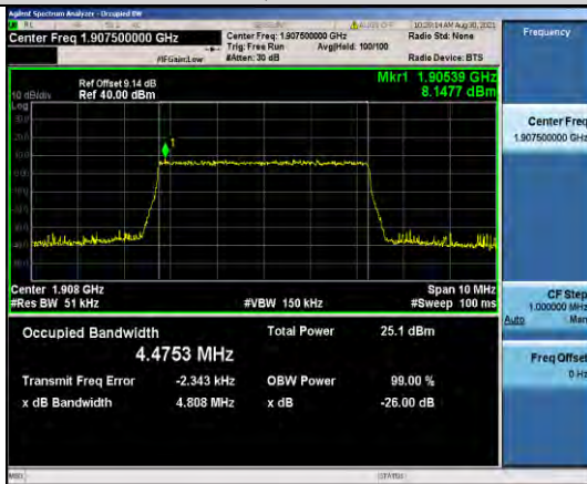
Band2-5MHz-QPSK-19175-25RB#0
