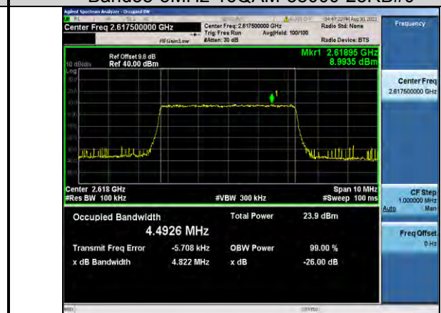
Band38-5MHz-16QAM-38225-25RB#0
