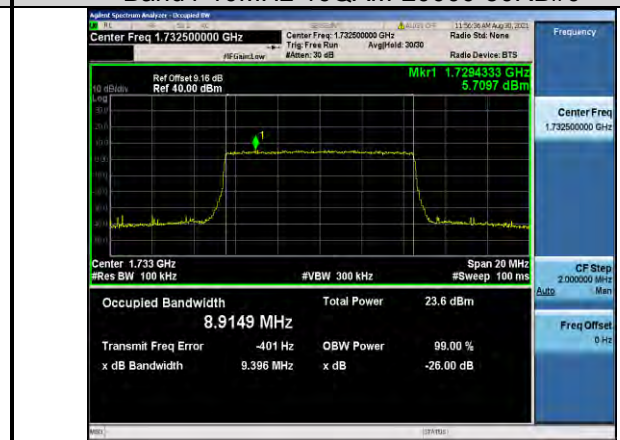
Band4-10MHz-16QAM-20175-50RB#0
