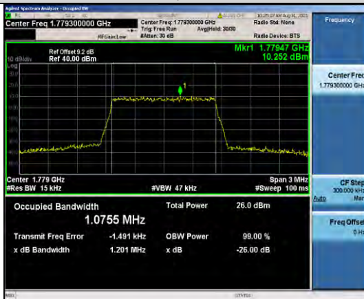
Band66-1.4MHz-QPSK-132665-6RB#0
