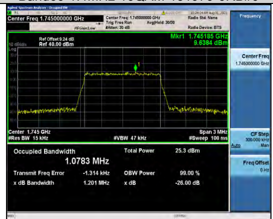
Band66-1.4MHz-16QAM-132322-6RB#0
