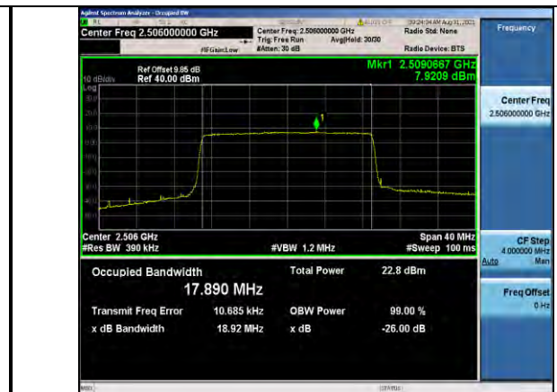
Band41-20MHz-16QAM-39750-100RB#0
