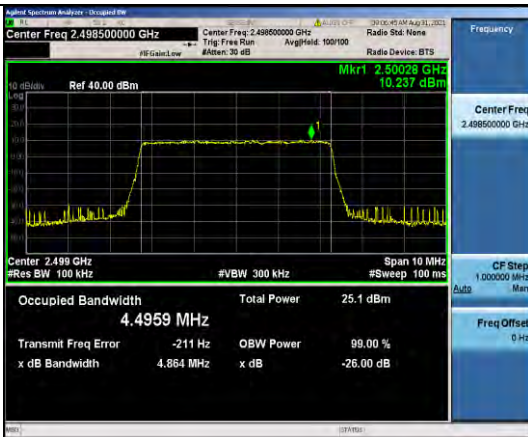
Band41-5MHz-QPSK-39675-25RB#0
