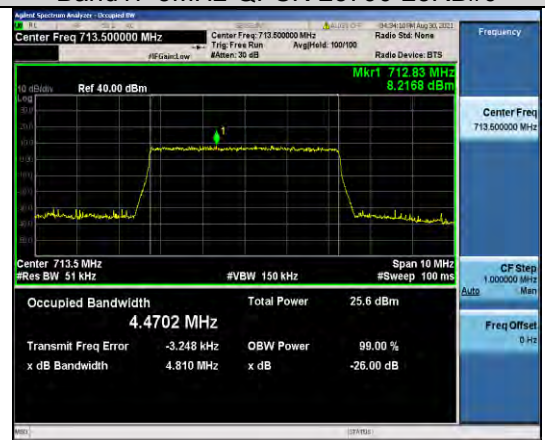
Band17-5MHz-QPSK-23825-25RB#0
