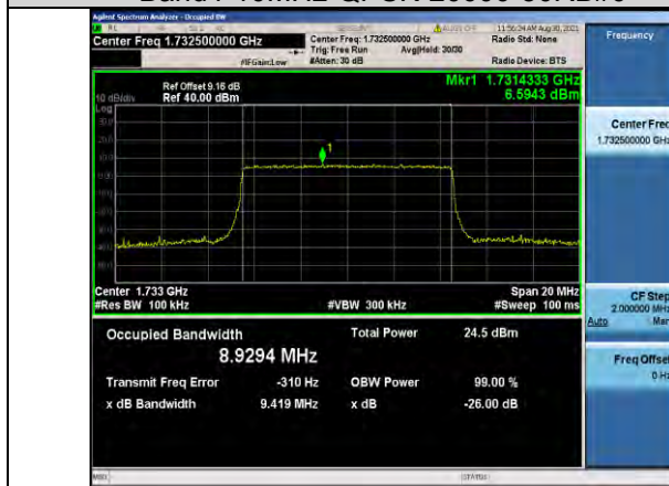
Band4-10MHz-QPSK-20175-50RB#0
