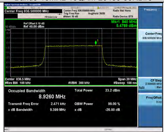
Band5-10MHz-16QAM-20525-50RB#0
