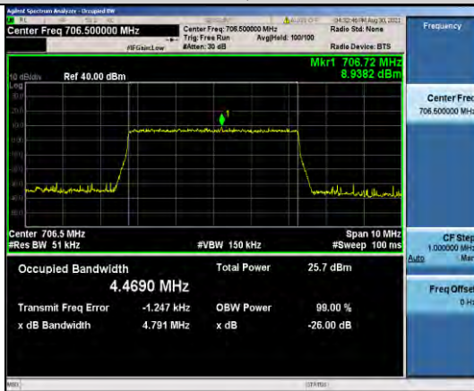
Band17-5MHz-QPSK-23755-25RB#0
