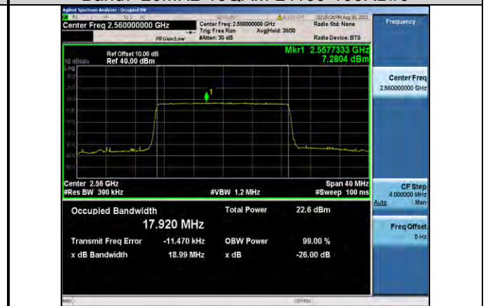
Band7-20MHz-16QAM-21350-100RB#0
