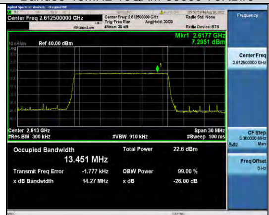
Band38-15MHz-16QAM-38175-75RB#0
