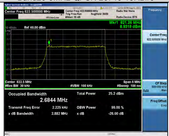
Band26-3MHz-QPSK-26775-15RB#0
