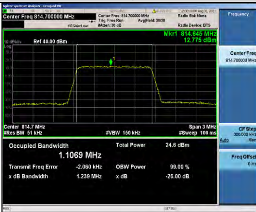
Band26-1.4MHz-QPSK-26697-6RB#0
