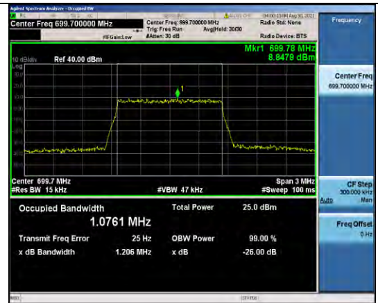
Band12-1.4MHz-16QAM-23017-6RB#0
