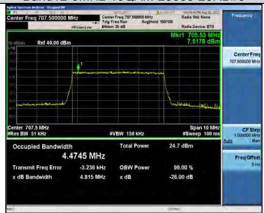
Band12-5MHz-16QAM-23095-25RB#0
