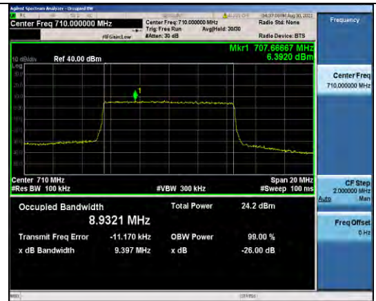
Band17-10MHz-QPSK-23790-50RB#0
