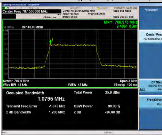
Band12-1.4MHz-QPSK-23095-6RB#0
