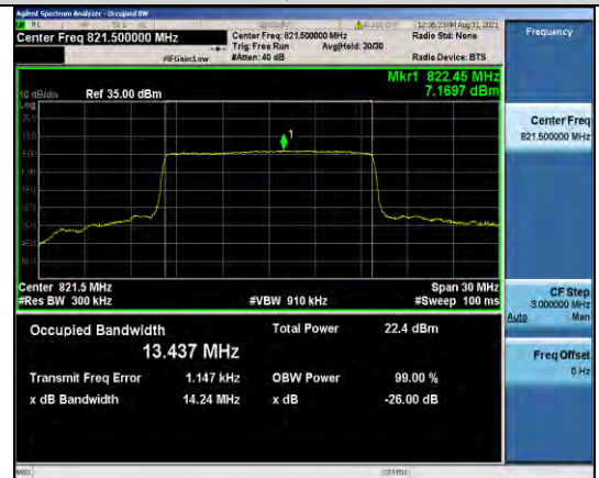
Band26-15MHz-16QAM-26765-75RB#0
