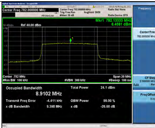
Band13-10MHz-QPSK-23230-50RB#0
