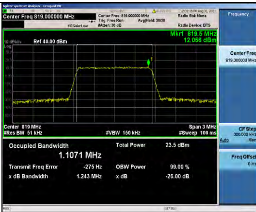
Band26-1.4MHz-16QAM-26740-6RB#0
