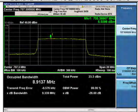
Band12-10MHz-16QAM-23095-50RB#0
