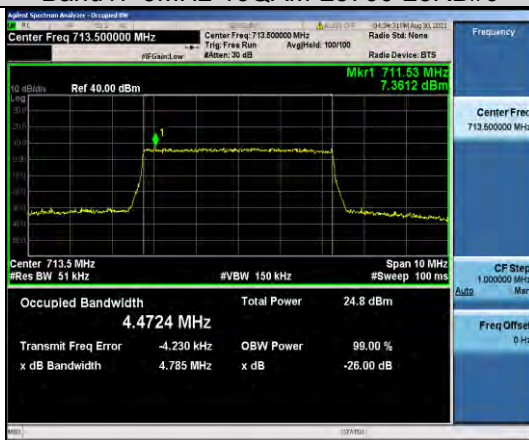
Band17-5MHz-16QAM-23825-25RB#0
