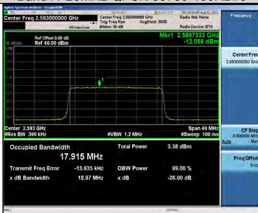
Band41-20MHz-QPSK-40620-100RB#0
