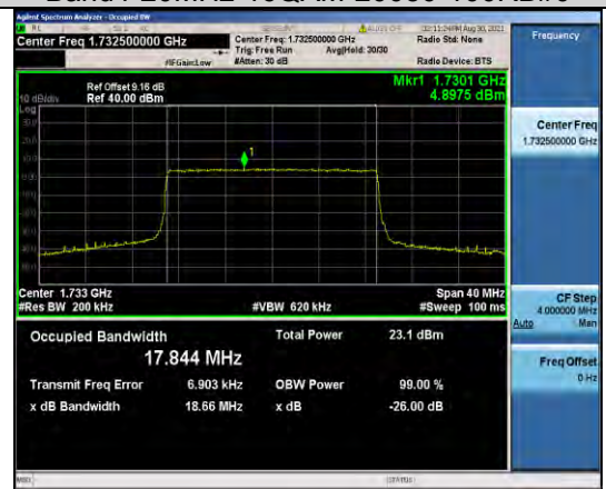
Band4-20MHz-16QAM-20175-100RB#0
