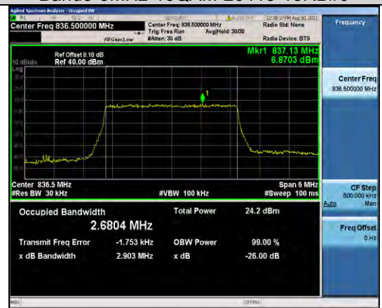
Band5-3MHz-16QAM-20525-15RB#0
