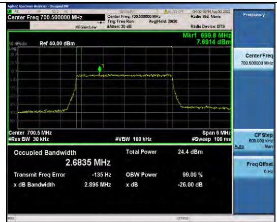
Band12-3MHz-16QAM-23025-15RB#0
