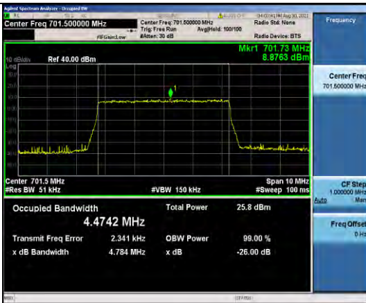
Band12-5MHz-QPSK-23035-25RB#0
