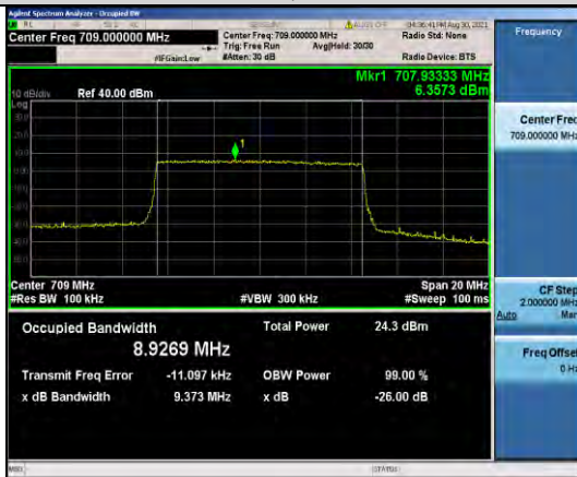
Band17-10MHz-QPSK-23780-50RB#0
