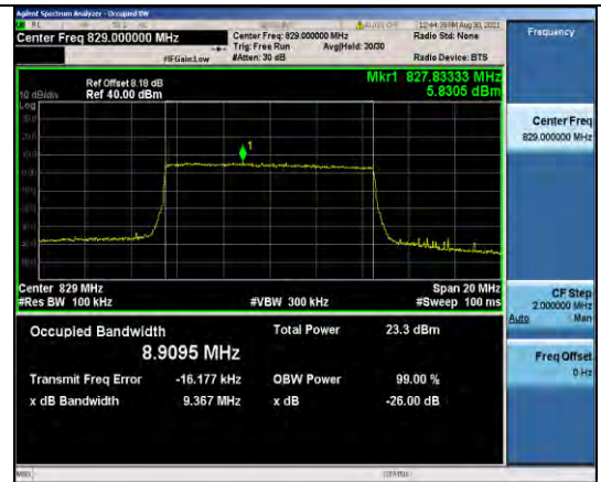
Band5-10MHz-16QAM-20450-50RB#0
