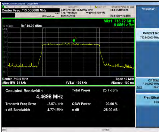
Band12-5MHz-QPSK-23155-25RB#0
