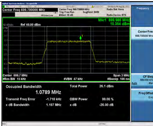
Band12-1.4MHz-QPSK-23017-6RB#0
