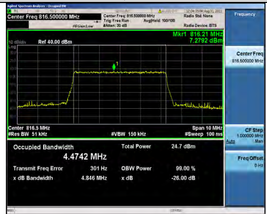
Band26-5MHz-16QAM-26715-25RB#0
