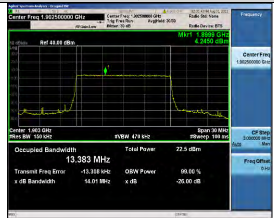
Band2-15MHz-16QAM-19125-75RB#0
