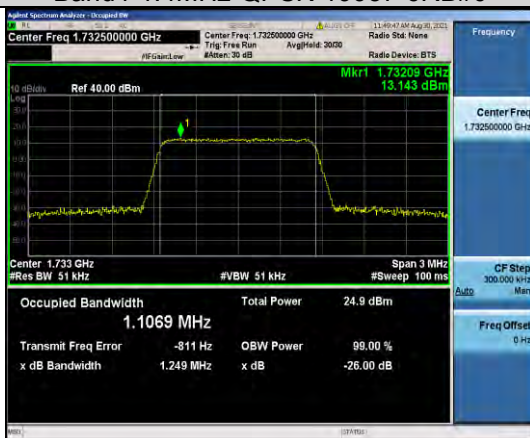
Band4-1.4MHz-QPSK-20175-6RB#0
