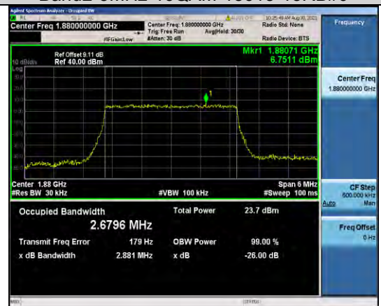
Band2-3MHz-16QAM-18900-15RB#0
