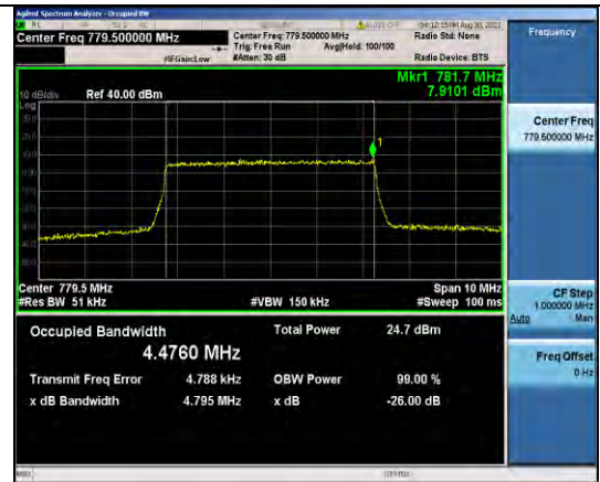
Band13-5MHz-16QAM-23205-25RB#0
