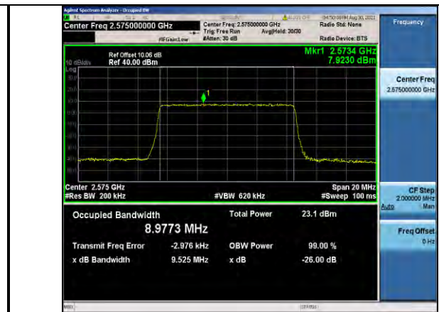
Band38-10MHz-16QAM-37800-50RB#0
