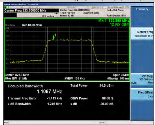
Band26-1.4MHz-QPSK-26783-6RB#0
