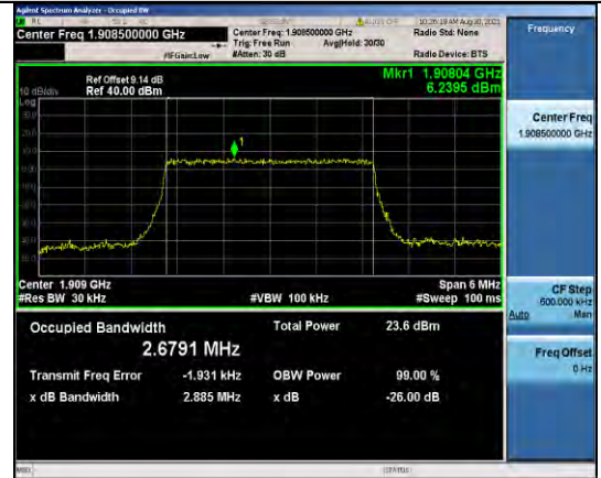
Band2-3MHz-16QAM-19185-15RB#0
