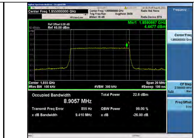
Band2-10MHz-16QAM-18650-50RB#0
