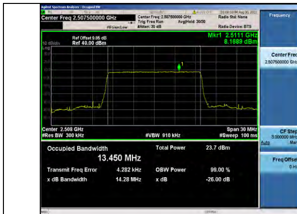
Band7-15MHz-QPSK-20825-75RB#0
