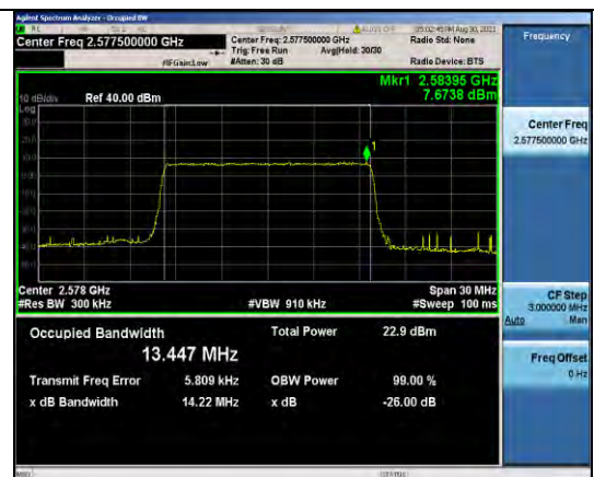
Band38-15MHz-16QAM-37825-75RB#0
