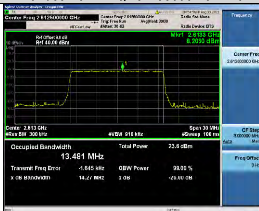
Band38-15MHz-QPSK-38175-75RB#0
