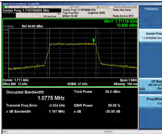
Band66-1.4MHz-QPSK-131979-6RB#0
