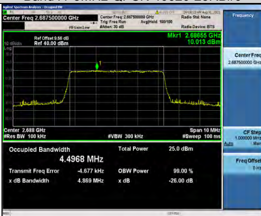
Band41-5MHz-QPSK-41565-25RB#0
