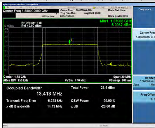
Band2-15MHz-QPSK-18900-75RB#0
