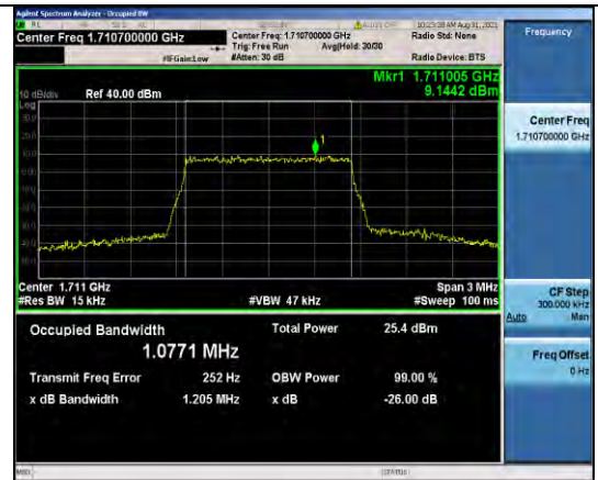
Band66-1.4MHz-16QAM-131979-6RB#0
