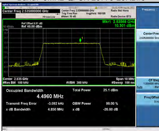
Band7-5MHz-QPSK-21100-25RB#0
