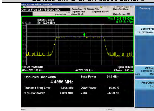
Band38-5MHz-QPSK-38225-25RB#0
