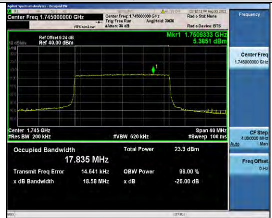
Band4-20MHz-16QAM-20300-100RB#0
