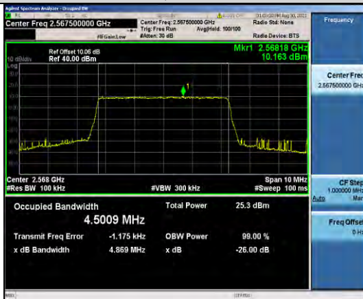
Band7-5MHz-QPSK-21425-25RB#0
