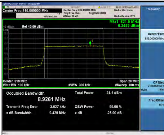
Band26-10MHz-QPSK-26740-50RB#0
