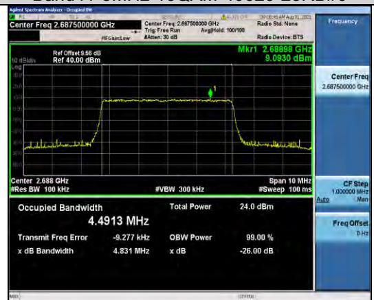
Band41-5MHz-16QAM-41565-25RB#0
