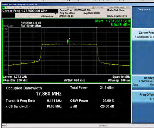
Band4-20MHz-QPSK-20175-100RB#0
