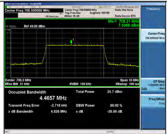
Band17-5MHz-16QAM-23755-25RB#0
