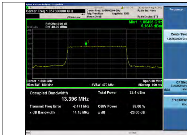
Band2-15MHz-QPSK-18675-75RB#0
