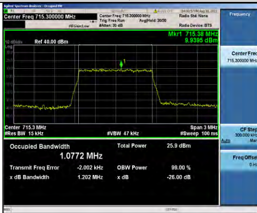
Band12-1.4MHz-QPSK-23173-6RB#0
