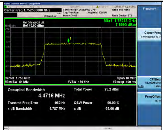
Band4-5MHz-16QAM-20375-25RB#0
