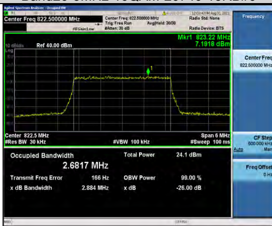
Band26-3MHz-16QAM-26775-15RB#0
