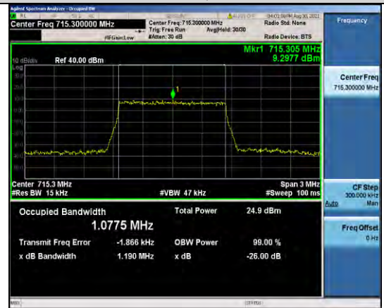
Band12-1.4MHz-16QAM-23173-6RB#0
