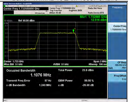
Band4-1.4MHz-16QAM-20175-6RB#0
