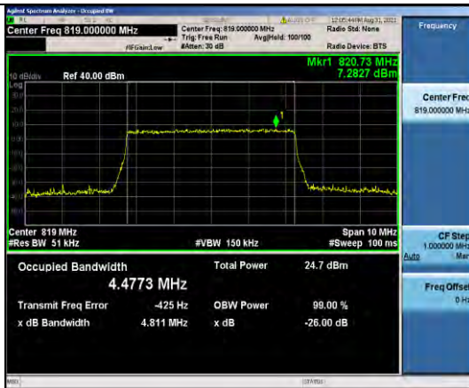
Band26-5MHz-16QAM-26740-25RB#0
