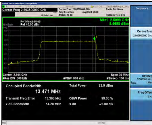
Band41-15MHz-QPSK-39725-75RB#0
