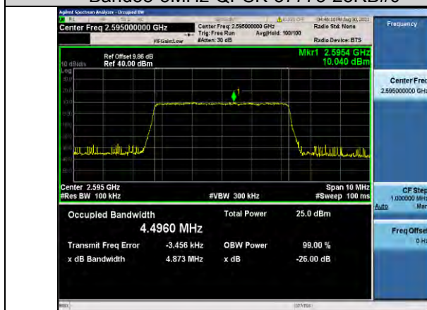
Band38-5MHz-QPSK-38000-25RB#0
