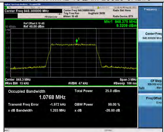
Band5-1.4MHz-16QAM-20643-6RB#0
