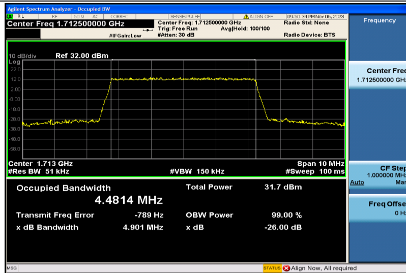
Band4-5MHz-QPSK-19975-25RB#0-4.4814
