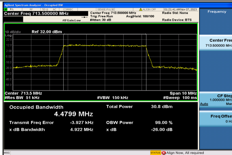
Band17-5MHz-16QAM-23825-25RB#0-4.4799
