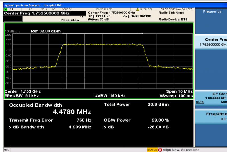
Band4-5MHz-16QAM-20375-25RB#0-4.4780
