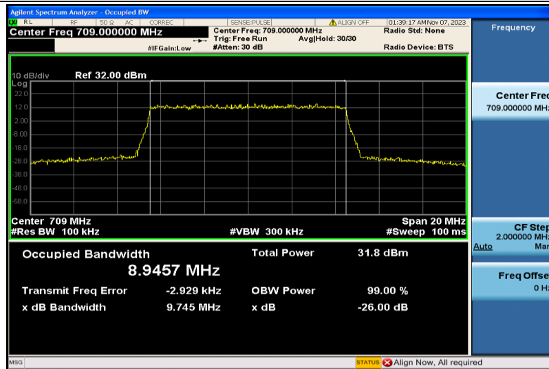
Band17-10MHz-QPSK-23780-50RB#0-8.9457
