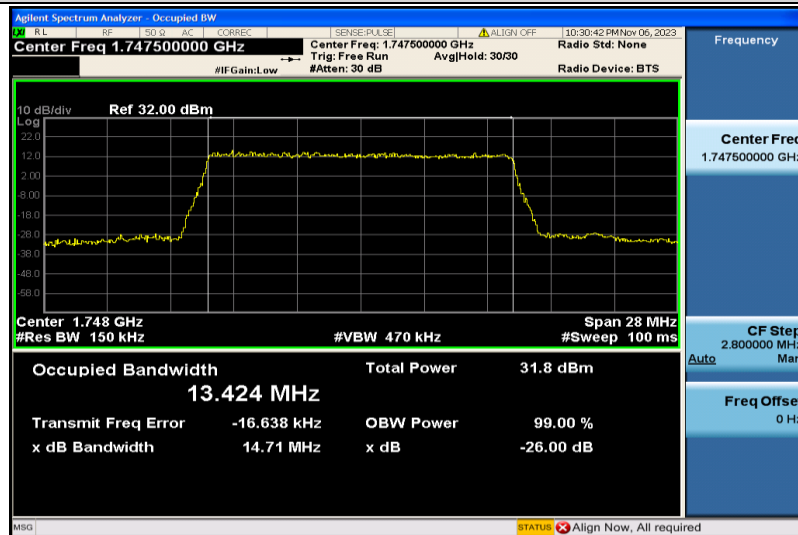
Band4-15MHz-QPSK-20325-75RB#0-13.424
