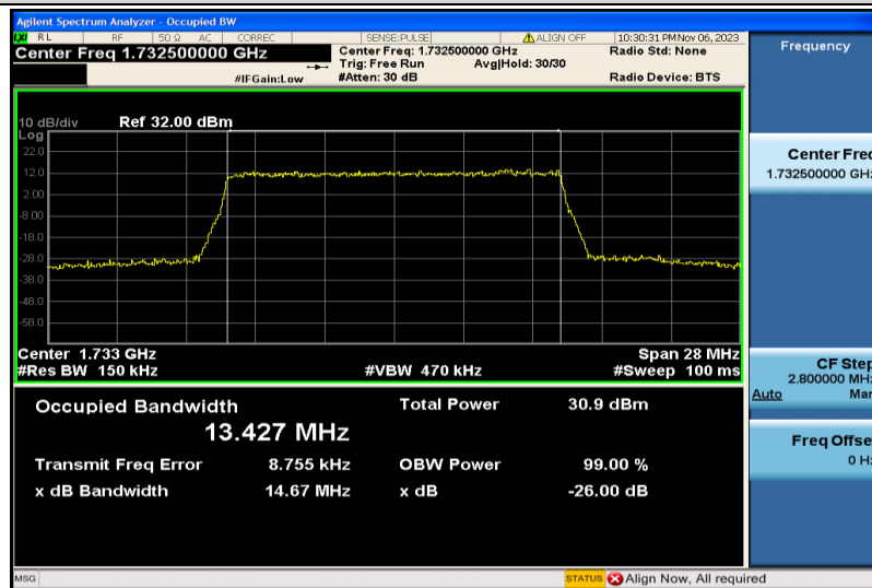
Band4-15MHz-16QAM-20175-75RB#0-13.427
