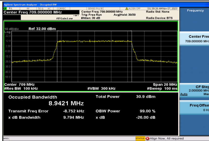
Band17-10MHz-16QAM-23780-50RB#0-8.9421
