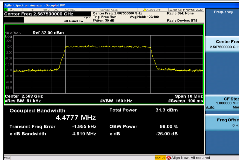
Band7-5MHz-QPSK-21425-25RB#0-4.4777
