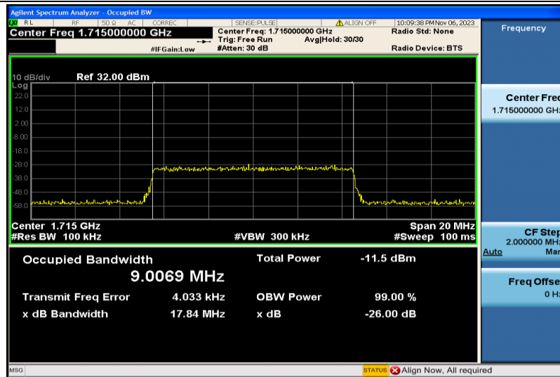
Band4-10MHz-QPSK-20000-50RB#0-9.0069
