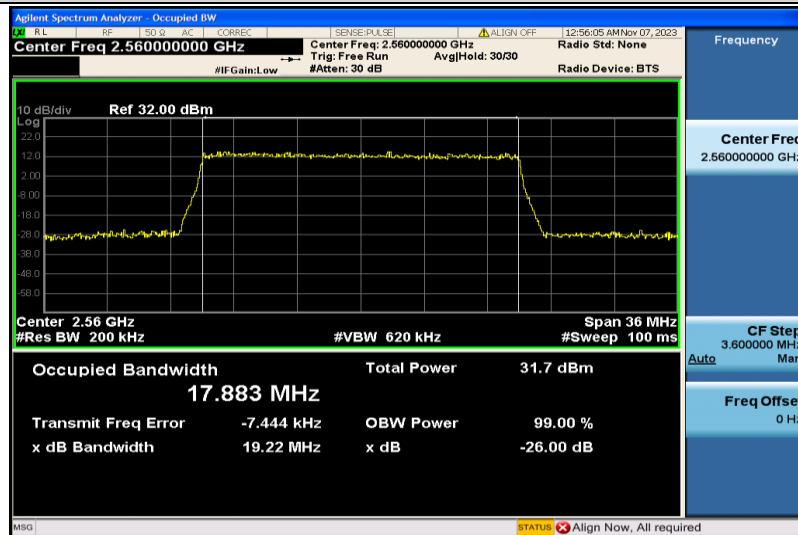
Band7-20MHz-QPSK-21350-100RB#0-17.883
