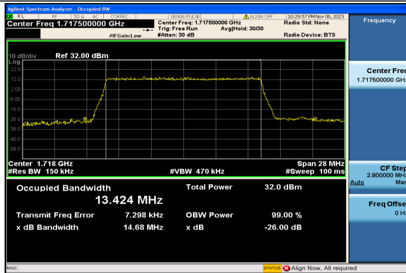
Band4-15MHz-QPSK-20025-75RB#0-13.424
