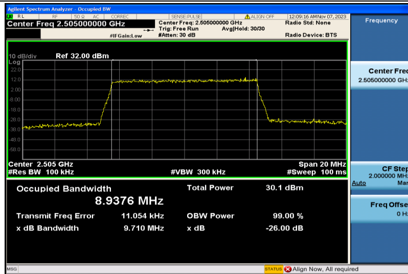
Band7-10MHz-16QAM-20800-50RB#0-8.9376
