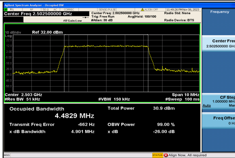
Band7-5MHz-QPSK-20775-25RB#0-4.4829
