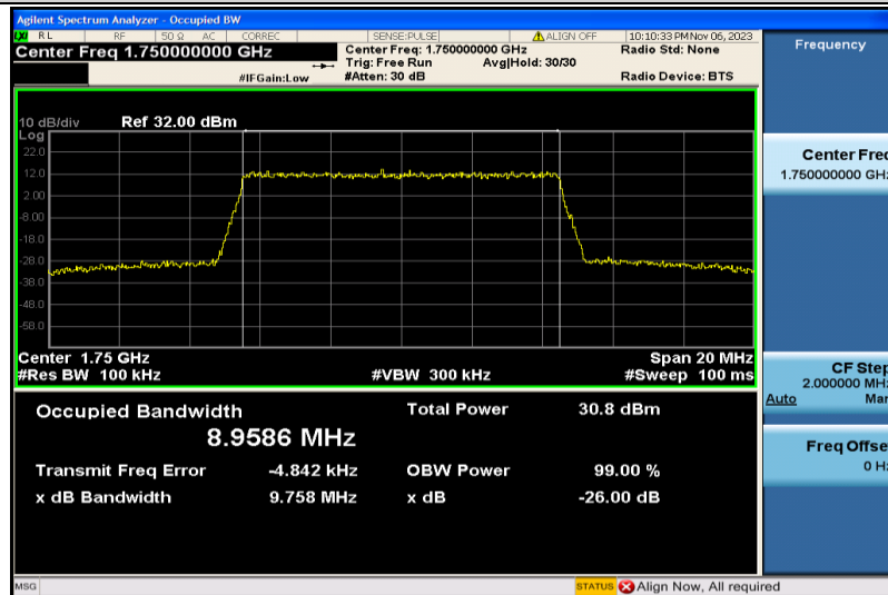
Band4-10MHz-16QAM-20350-50RB#0-8.9586
