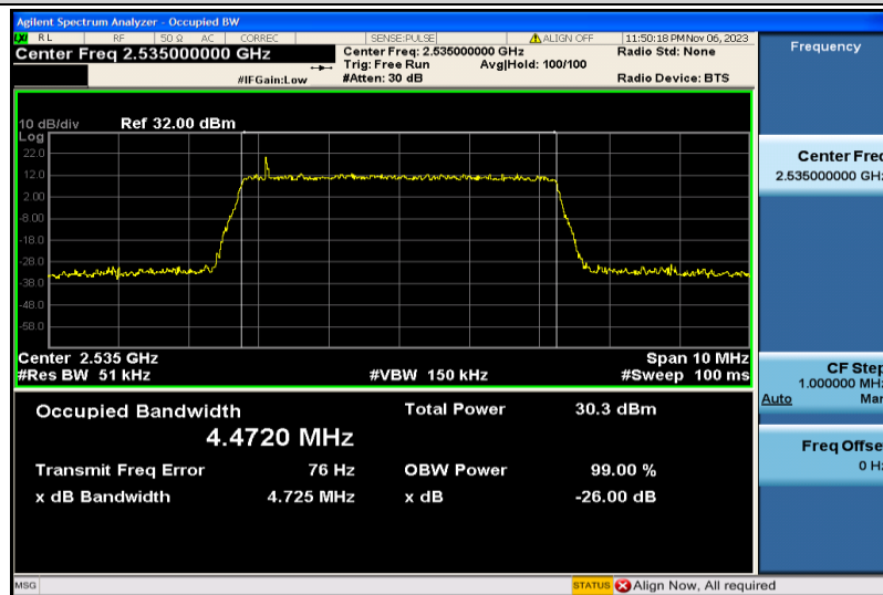
Band7-5MHz-16QAM-21100-25RB#0-4.4720
