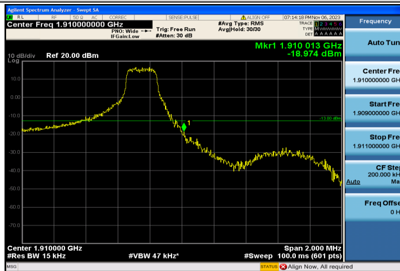
Band2-1.4MHz-16QAM-1913-1RB#5
