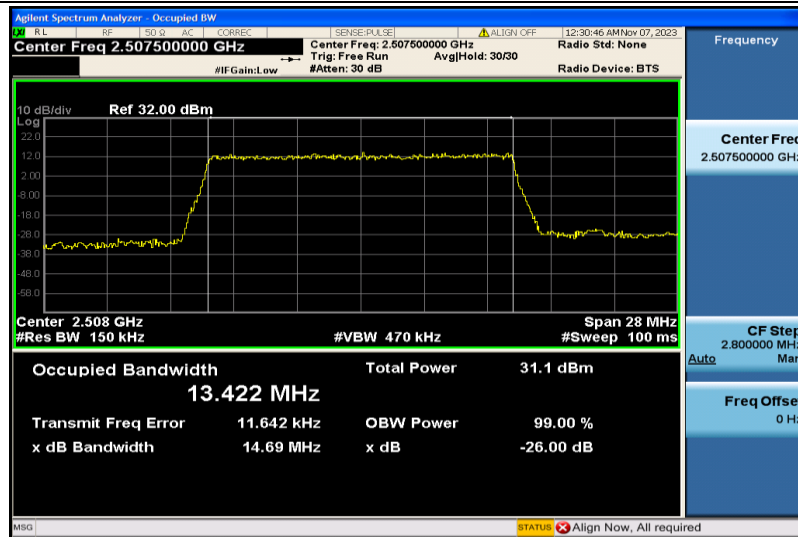
Band7-15MHz-QPSK-20825-75RB#0-13.422
