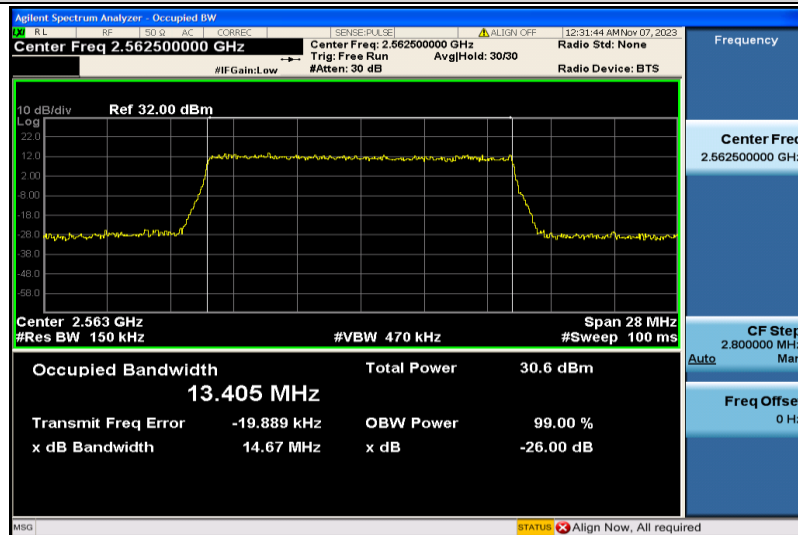
Band7-15MHz-16QAM-21375-75RB#0-13.405
