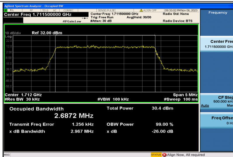
Band4-3MHz-16QAM-19965-15RB#0-2.6872
