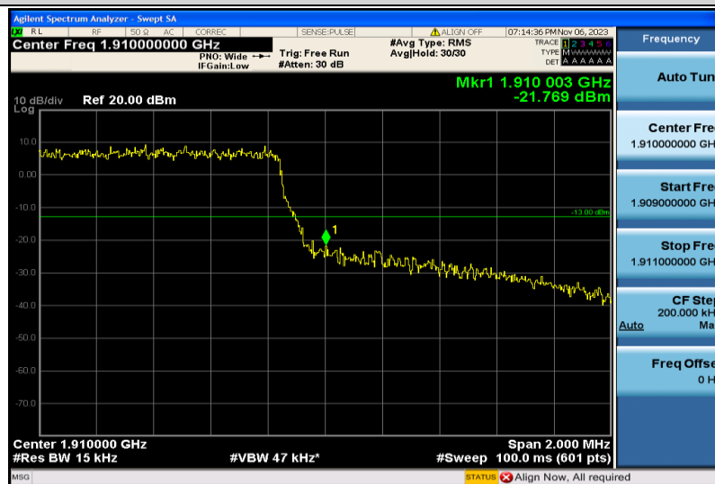
Band2-1.4MHz-16QAM-1913-6RB#0
