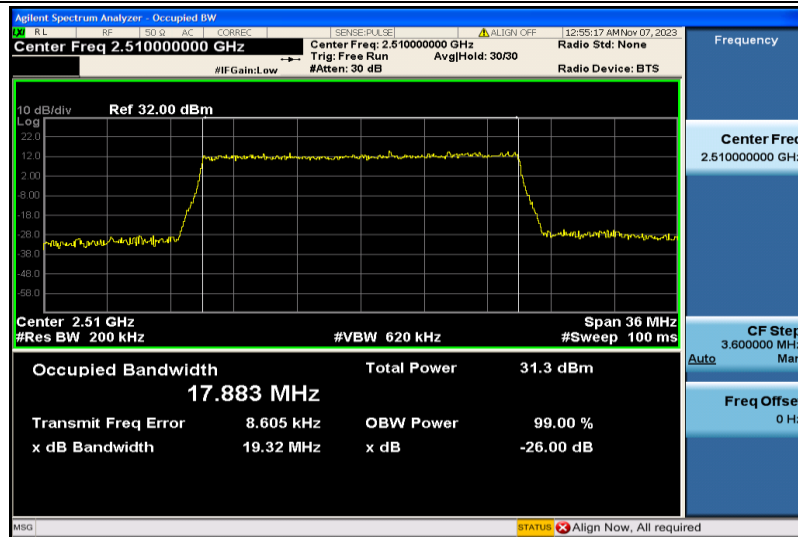
Band7-20MHz-QPSK-20850-100RB#0-17.883
