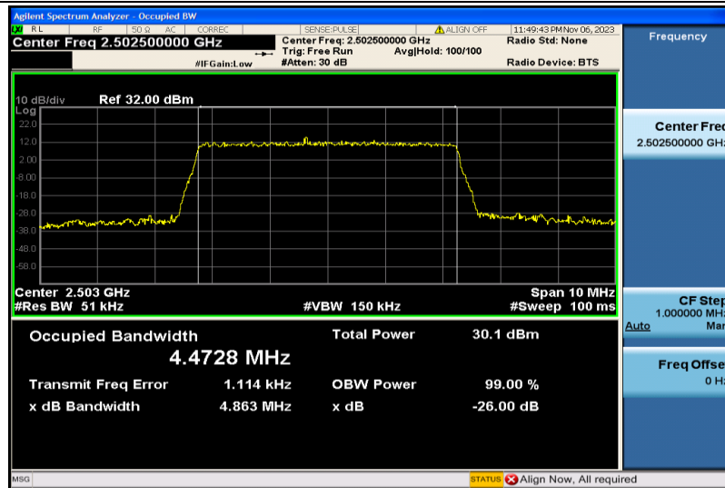
Band7-5MHz-16QAM-20775-25RB#0-4.4728
