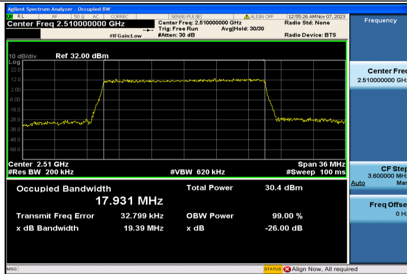
Band7-20MHz-16QAM-20850-100RB#0-17.931
