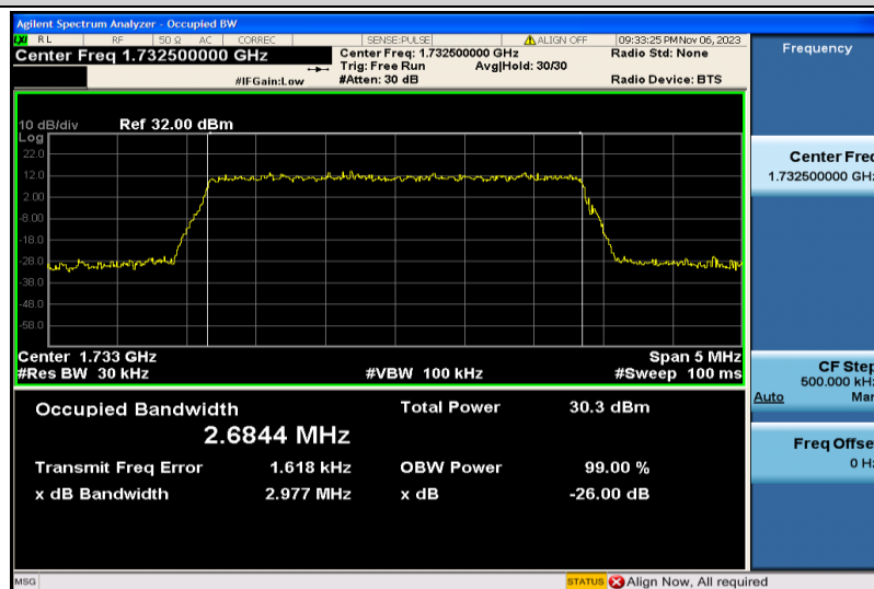
Band4-3MHz-16QAM-20175-15RB#0-2.6844
