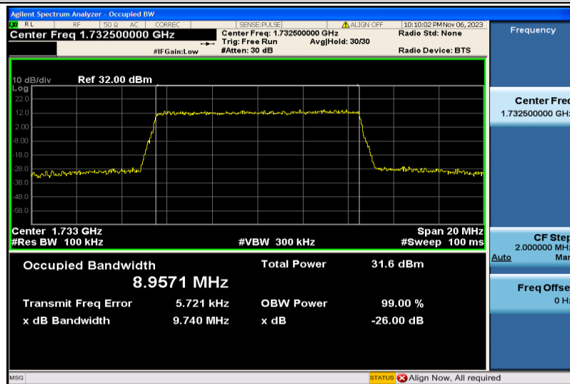
Band4-10MHz-QPSK-20175-50RB#0-8.9571
