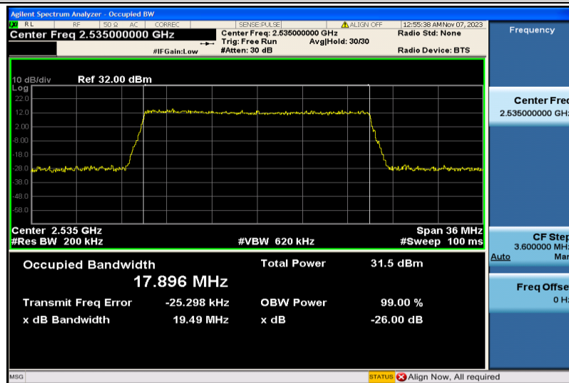
Band7-20MHz-QPSK-21100-100RB#0-17.896
