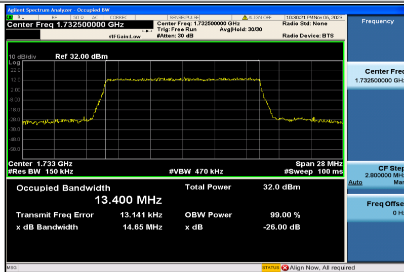
Band4-15MHz-QPSK-20175-75RB#0-13.400
