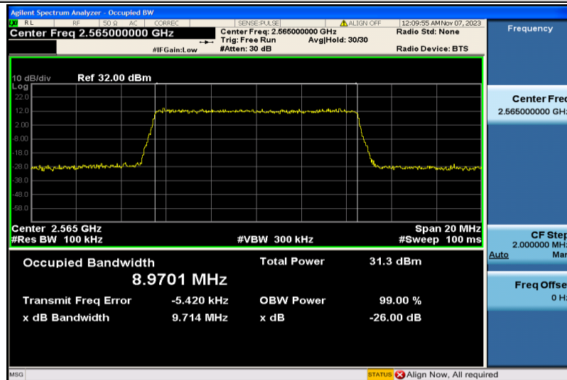
Band7-10MHz-QPSK-21400-50RB#0-8.9701
