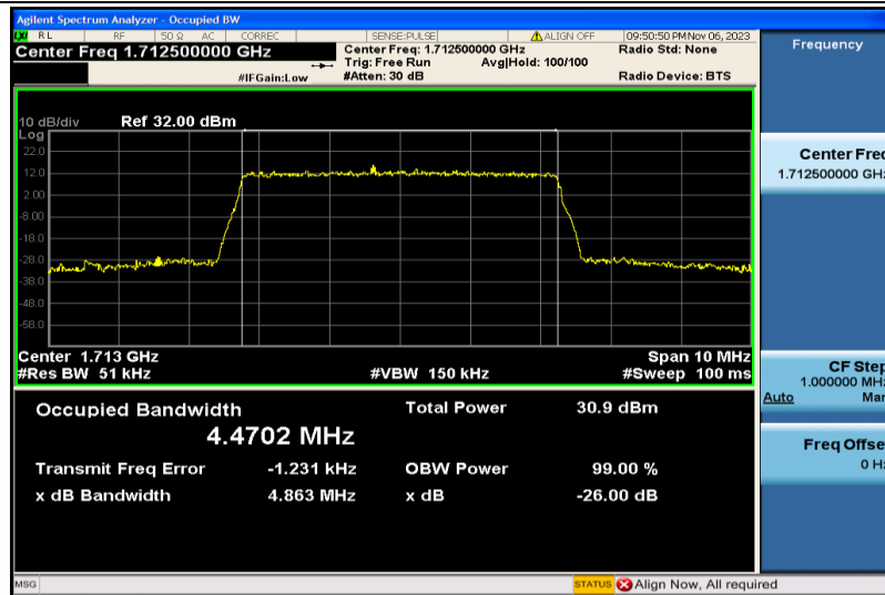
Band4-5MHz-16QAM-19975-25RB#0-4.4702
