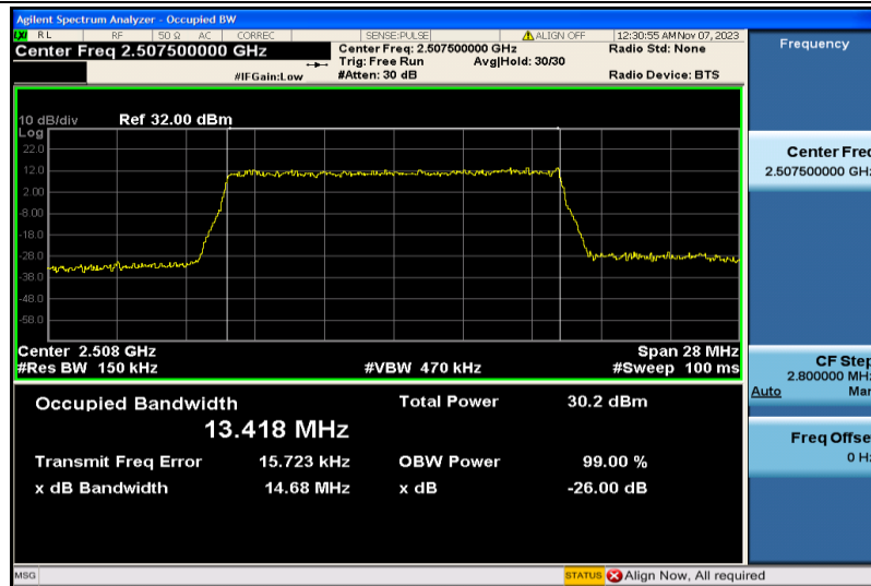
Band7-15MHz-16QAM-20825-75RB#0-13.418
