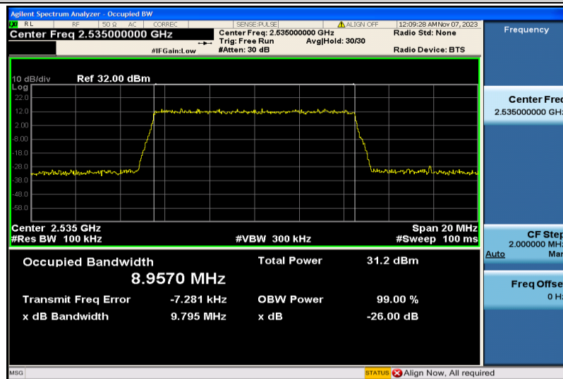
Band7-10MHz-QPSK-21100-50RB#0-8.9570
