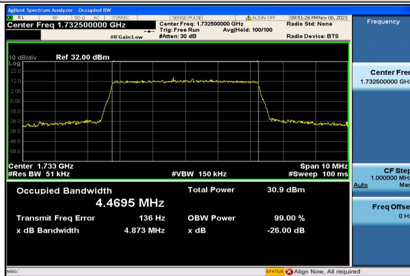
Band4-5MHz-16QAM-20175-25RB#0-4.4695
