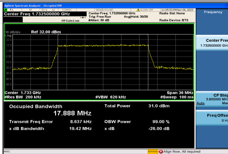
Band4-20MHz-16QAM-20175-100RB#0-17.888
