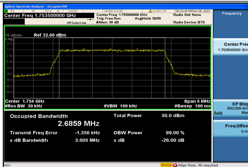
Band4-3MHz-16QAM-20385-15RB#0-2.6859
