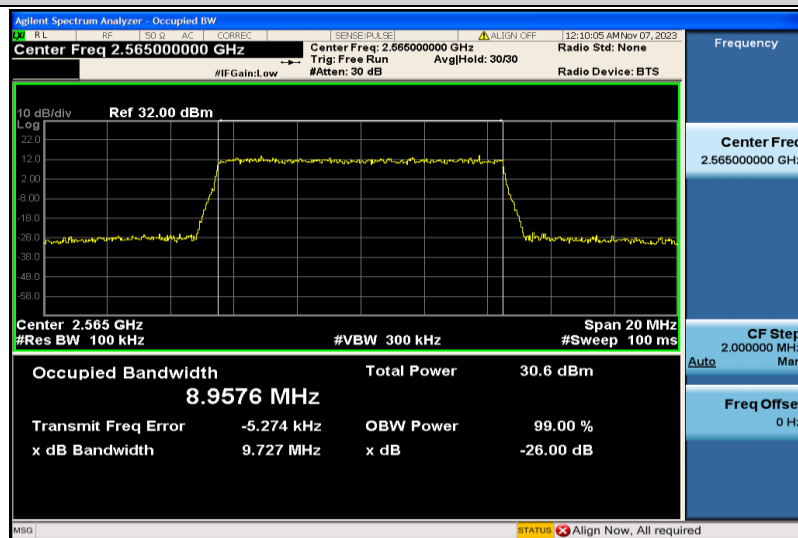
Band7-10MHz-16QAM-21400-50RB#0-8.9576
