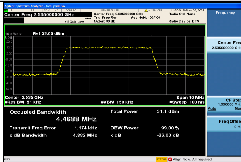
Band7-5MHz-QPSK-21100-25RB#0-4.4688
