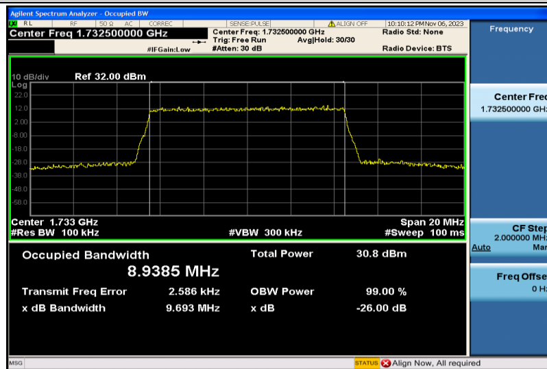
Band4-10MHz-16QAM-20175-50RB#0-8.9385
