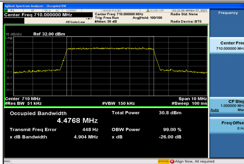
Band17-5MHz-16QAM-23790-25RB#0-4.4768
