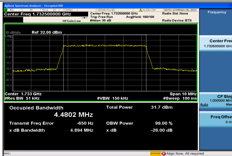
Band4-5MHz-QPSK-20175-25RB#0-4.4802
