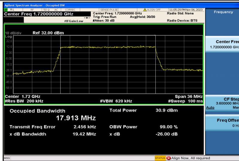
Band4-20MHz-16QAM-20050-100RB#0-17.913
