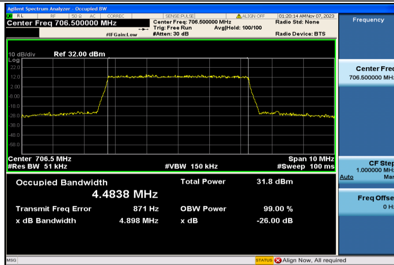
Band17-5MHz-QPSK-23755-25RB#0-4.4838
