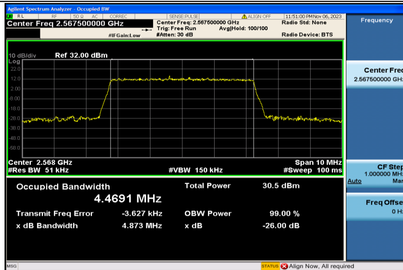
Band7-5MHz-16QAM-21425-25RB#0-4.4691
