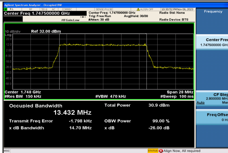
Band4-15MHz-16QAM-20325-75RB#0-13.432
