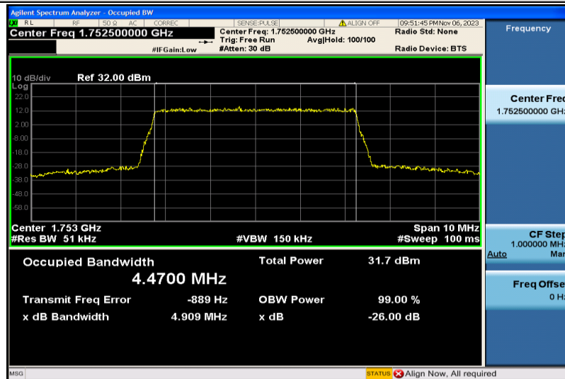
Band4-5MHz-QPSK-20375-25RB#0-4.4700
