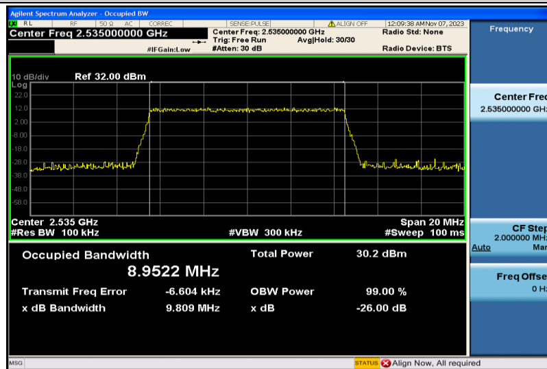
Band7-10MHz-16QAM-21100-50RB#0-8.9522
