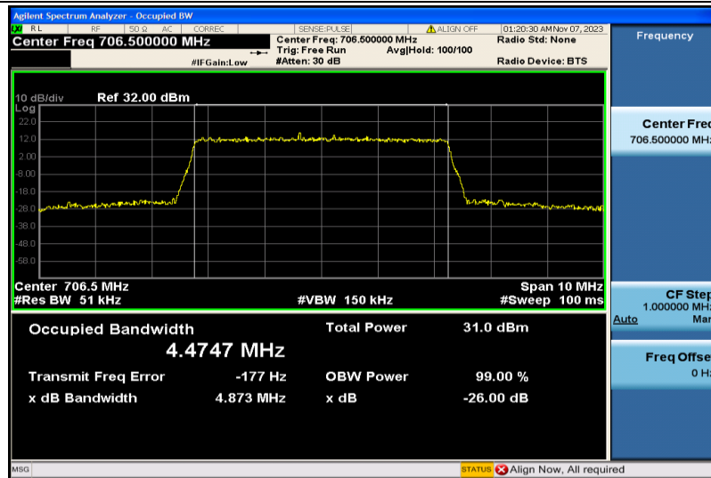
Band17-5MHz-16QAM-23755-25RB#0-4.4747
