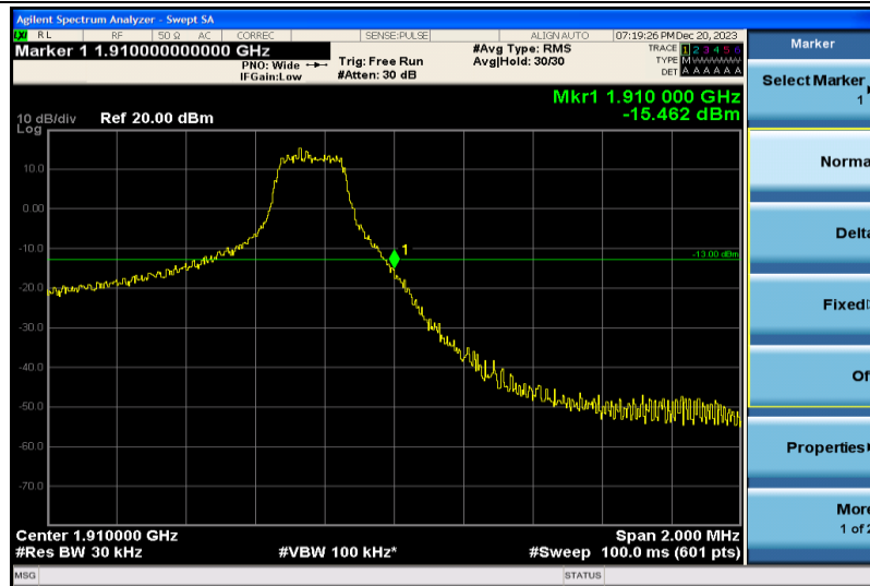
Band2-3MHz-16QAM-19185-1RB#14
