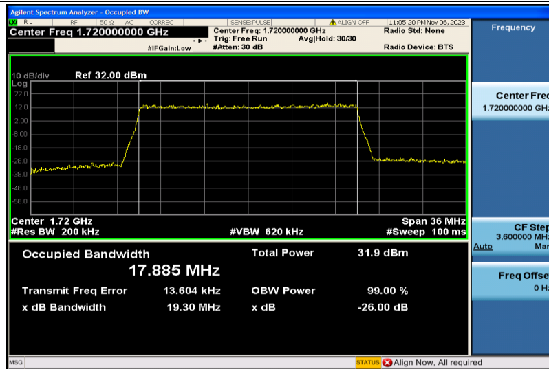
Band4-20MHz-QPSK-20050-100RB#0-17.885
