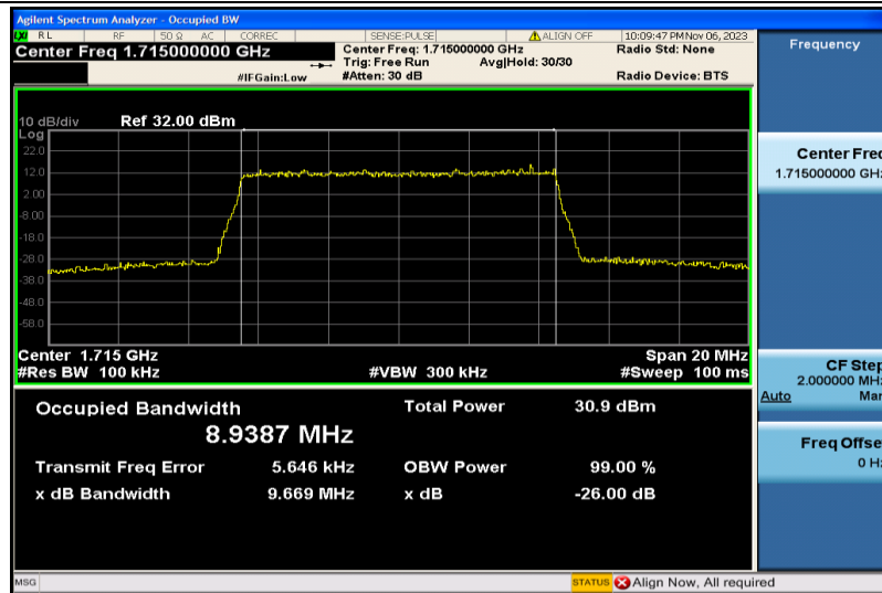
Band4-10MHz-16QAM-20000-50RB#0-8.9387
