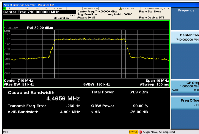
Band17-5MHz-QPSK-23790-25RB#0-4.4656
