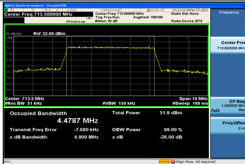
Band17-5MHz-QPSK-23825-25RB#0-4.4787
