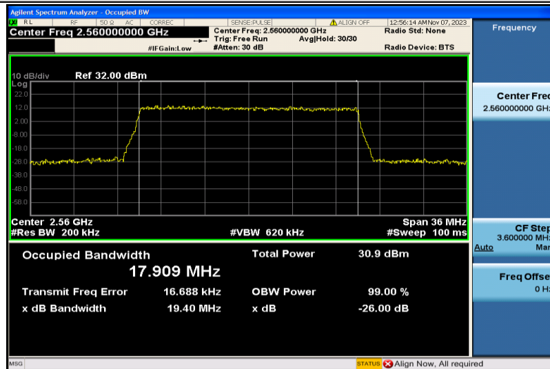
Band7-20MHz-16QAM-21350-100RB#0-17.909
