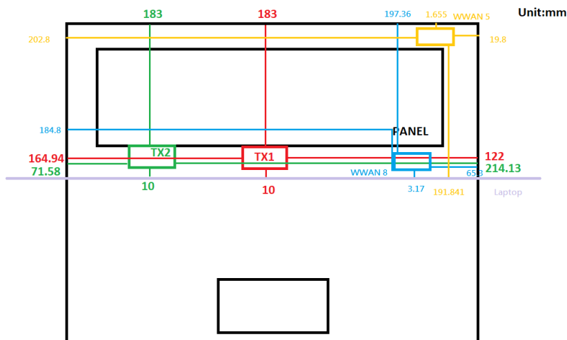
Fig.6 WWAN Antenna location
