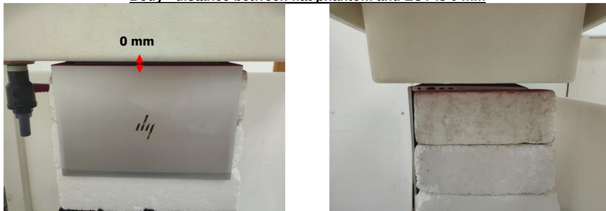
Fig.3 EUT Bottom side to flat phantom
