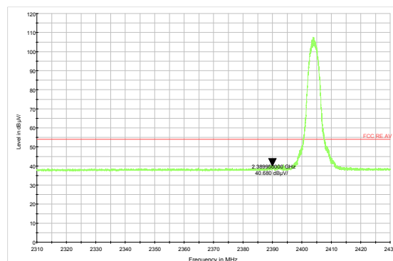
BT UHD 2M 8DPSK_2404MHz: Average
