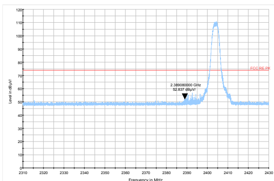
BT UHD 2M 8DPSK_2404MHz: Peak
