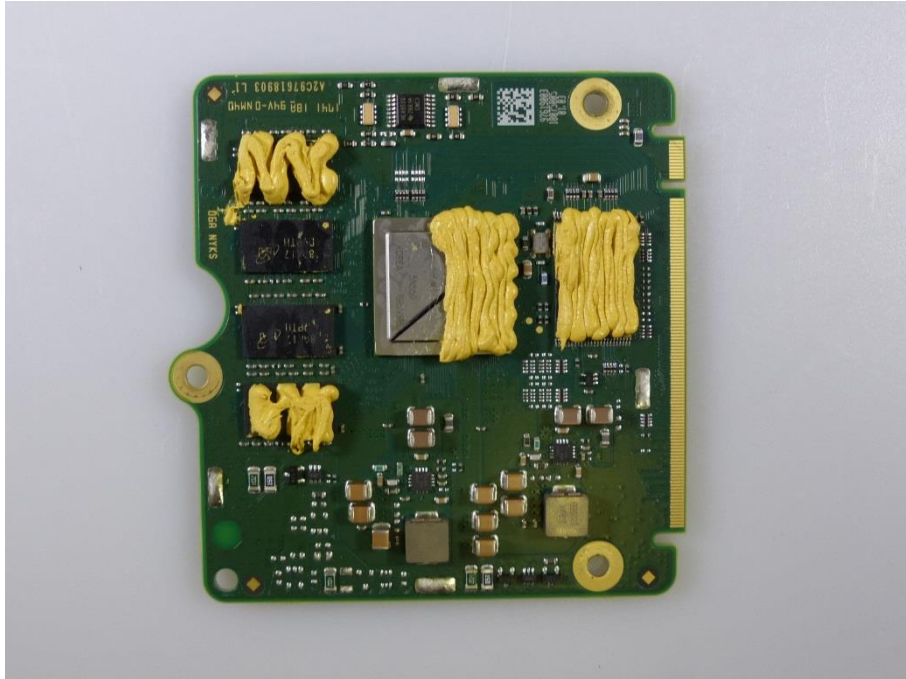
Photo 7: PCB 2 front side view
