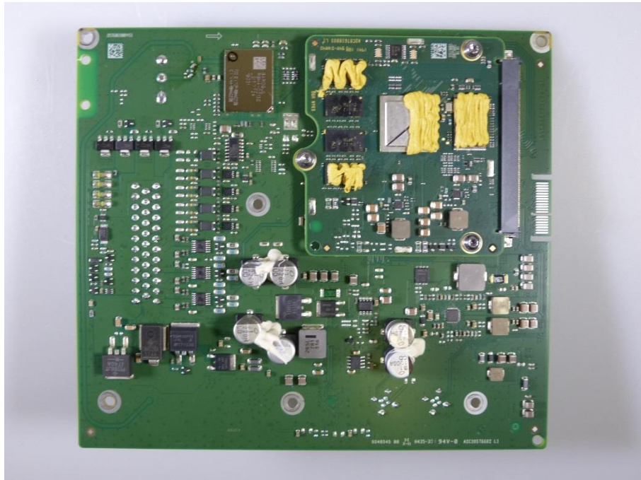
Photo 5: PCB 1 front side view with PCB 2 on it
