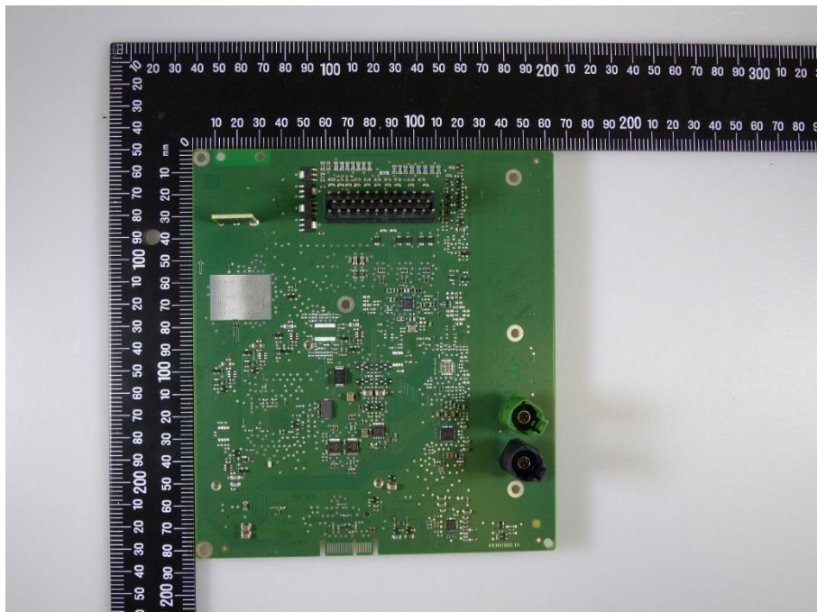
Photo 4: PCB 1 back side view
