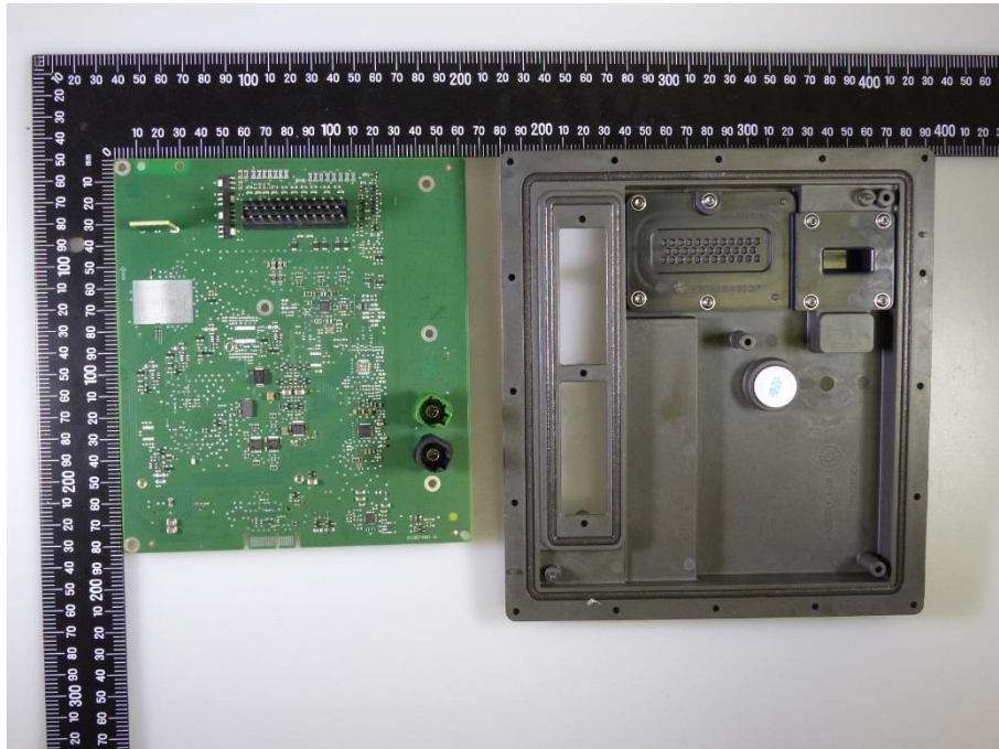
Photo 3: PCB 1 back side view
