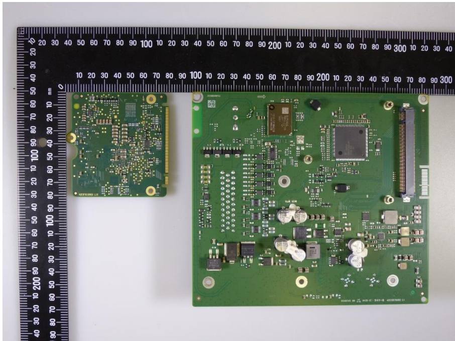
Photo 8: PCB 2 back side view and PCB 1 front side view
