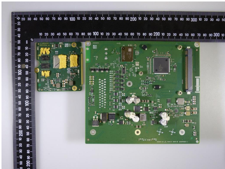
Photo 6: PCB 1 front side view and PCB 2 front side view
