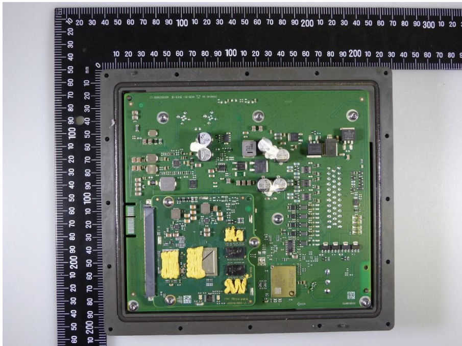
Photo 2: EUT opened
