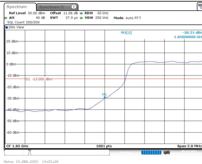
Band2-5MHz-16QAM-19175-1RB#24
