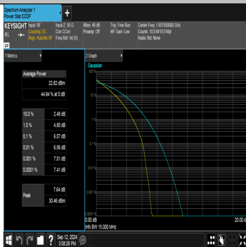
Band2-15MHz-QPSK-18675-75RB#0-PASS
