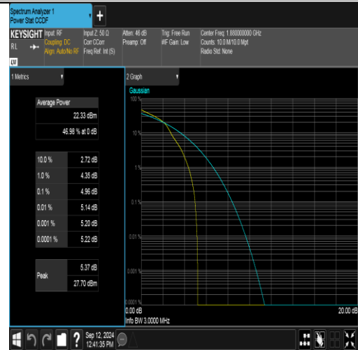
Band2-3MHz-16QAM-18900-1RB#0-PASS
