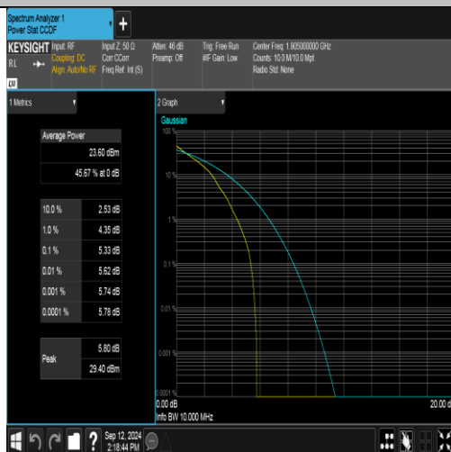
Band2-10MHz-QPSK-19150-1RB#0-PASS
