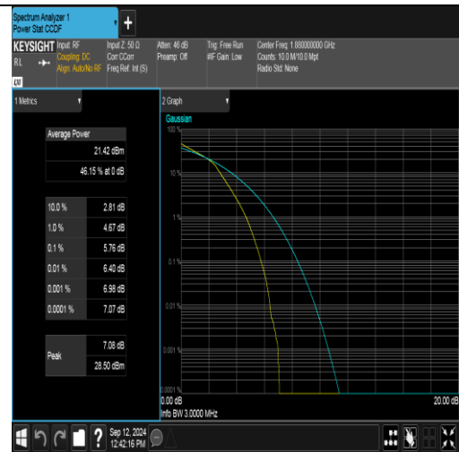
Band2-3MHz-16QAM-18900-15RB#0-PASS
