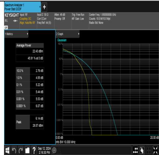
Band2-10MHz-16QAM-18900-1RB#0-PASS
