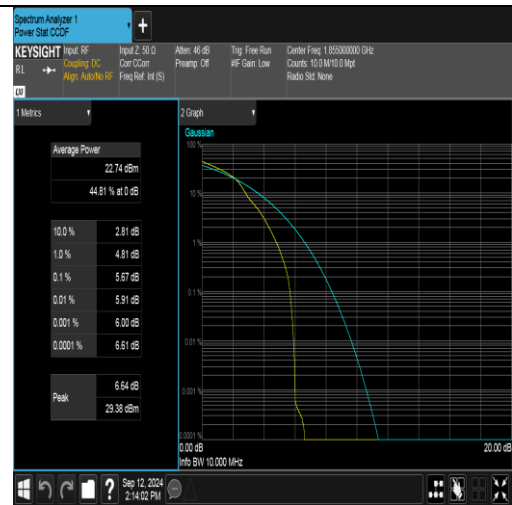
Band2-10MHz-16QAM-18650-1RB#0-PASS
