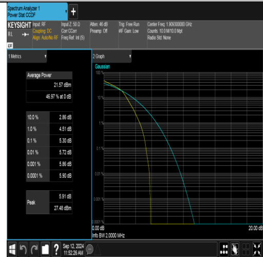
Band2-1.4MHz-16QAM-19193-6RB#0-PASS
