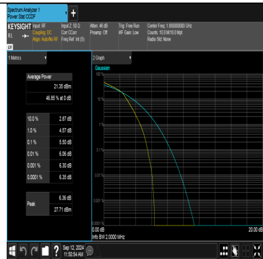
Band2-1.4MHz-16QAM-18900-6RB#0-PASS
