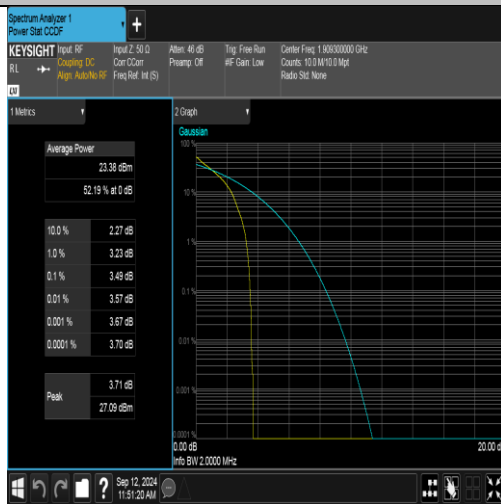
Band2-1.4MHz-QPSK-19193-1RB#0-PASS
