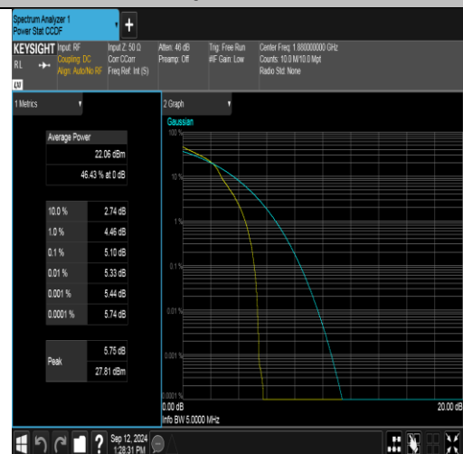
Band2-5MHz-16QAM-18900-1RB#0-PASS
