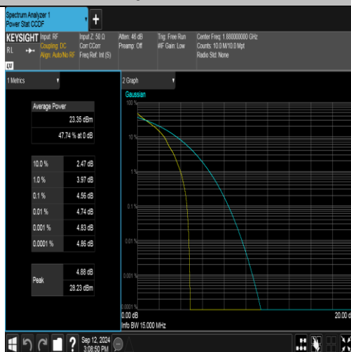
Band2-15MHz-QPSK-18900-1RB#0-PASS
