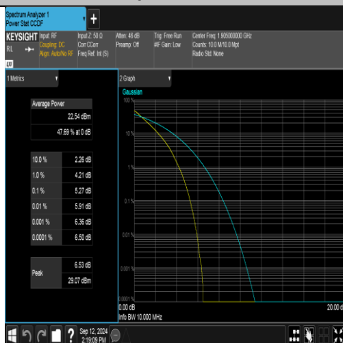
Band2-10MHz-QPSK-19150-50RB#0-PASS
