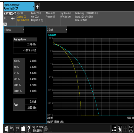
Band2-15MHz-16QAM-18900-75RB#0-PASS
