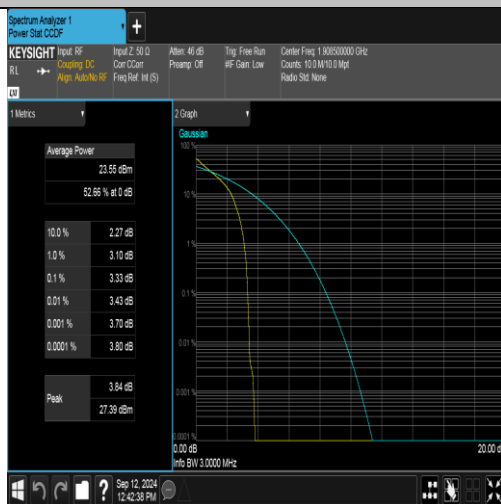
Band2-3MHz-QPSK-19185-1RB#0-PASS
