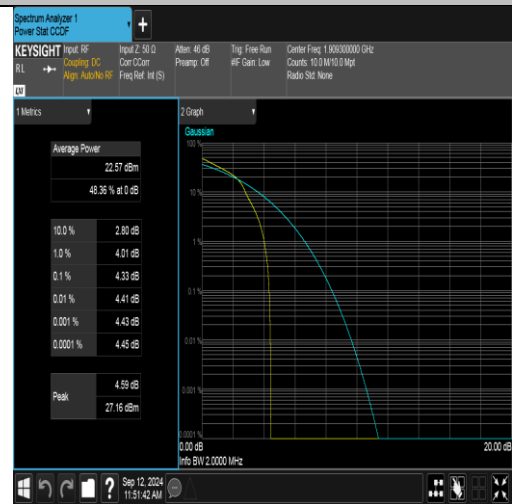
Band2-1.4MHz-16QAM-19193-1RB#0-PASS
