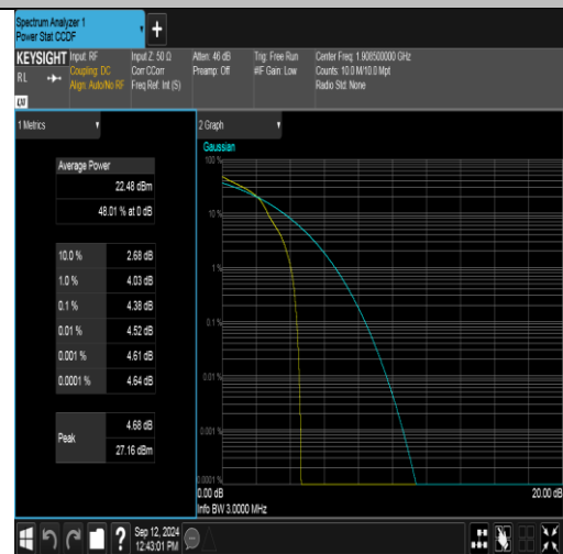
Band2-3MHz-16QAM-19185-1RB#0-PASS
