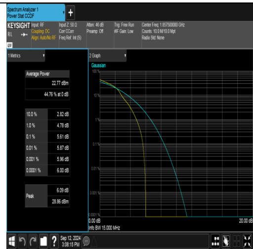
Band2-15MHz-16QAM-18675-1RB#0-PASS
