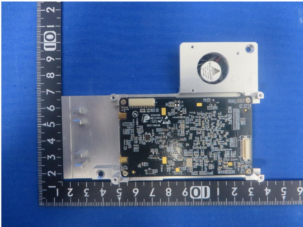
(18) EUT Photo (Model: WLN210-BM-d)
