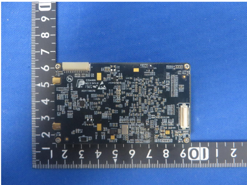
(6) EUT Photo (Model: WLN210-BM-a)
