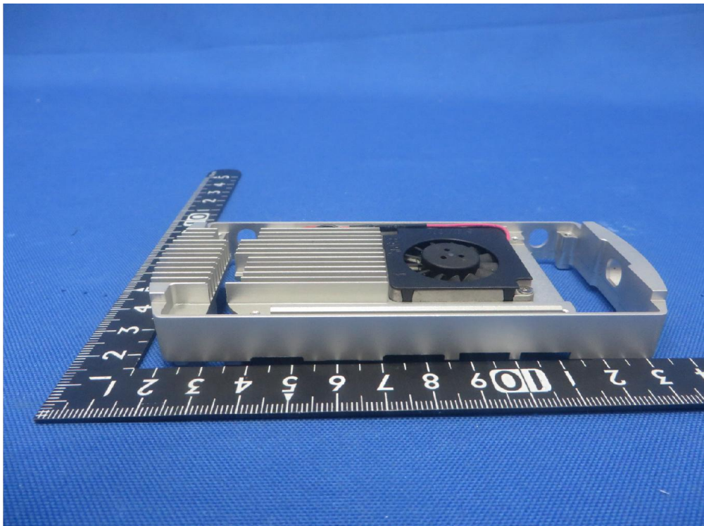
(22) EUT Photo (Model: WLN210-BM-a)
