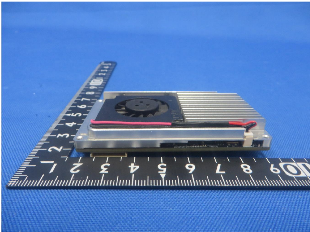
(2) EUT Photo (Model: WLN210-BM-a)
