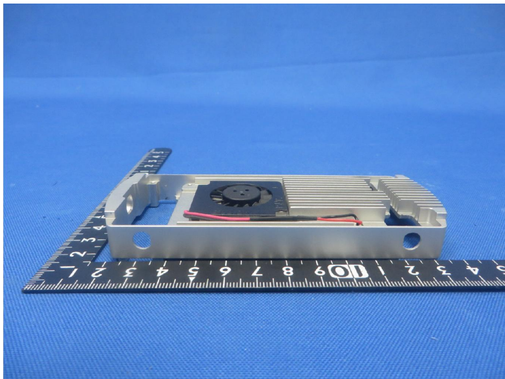
(20) EUT Photo (Model: WLN210-BM-d)
