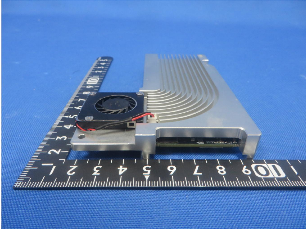
(17) EUT Photo (Model: WLN210-BM-c)
