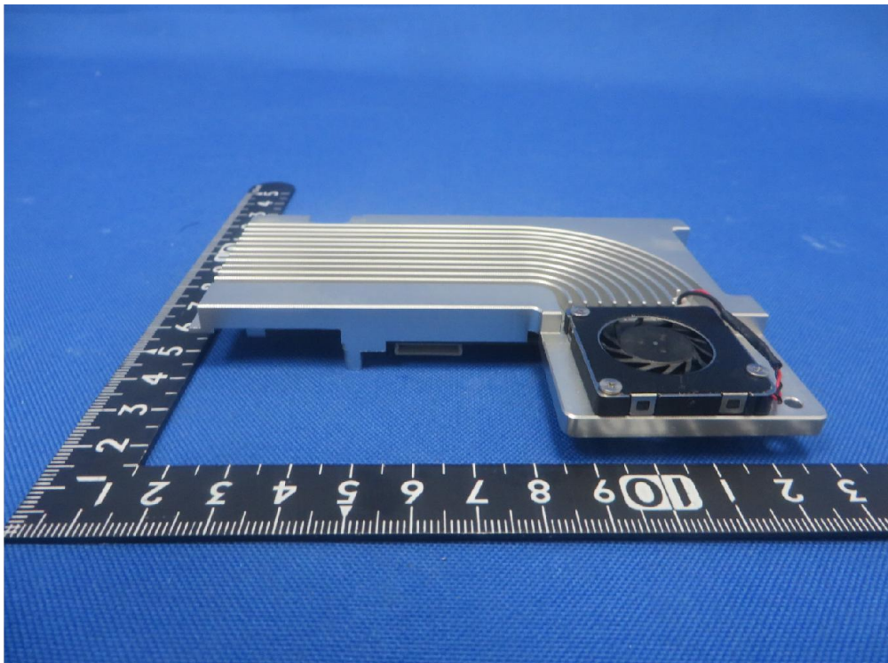
(16) EUT Photo (Model: WLN210-BM-c)
