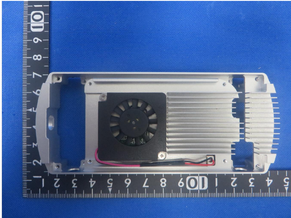
(19) EUT Photo (Model: WLN210-BM-d)
