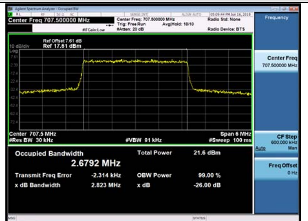
MCH_16QAM_15RB#0
