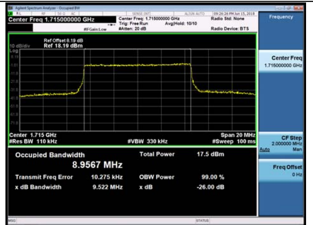
LCH_16QAM_50RB#0
