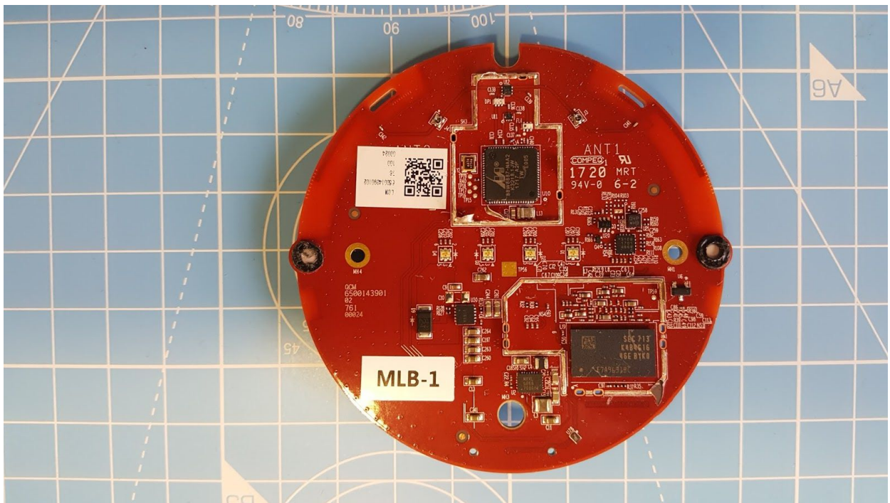
Bottom View PCB, Shield Cans Removed
