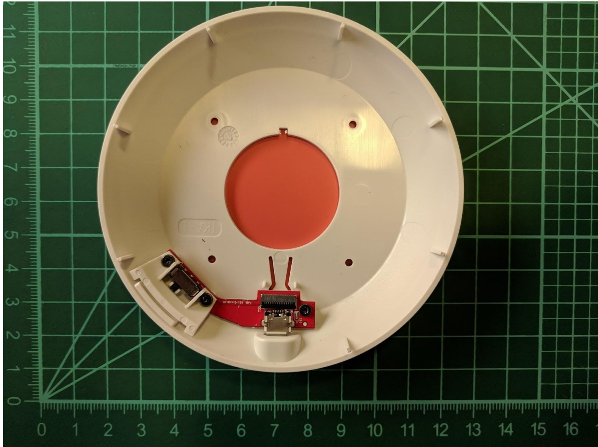
Speaker Connection Close-Up
