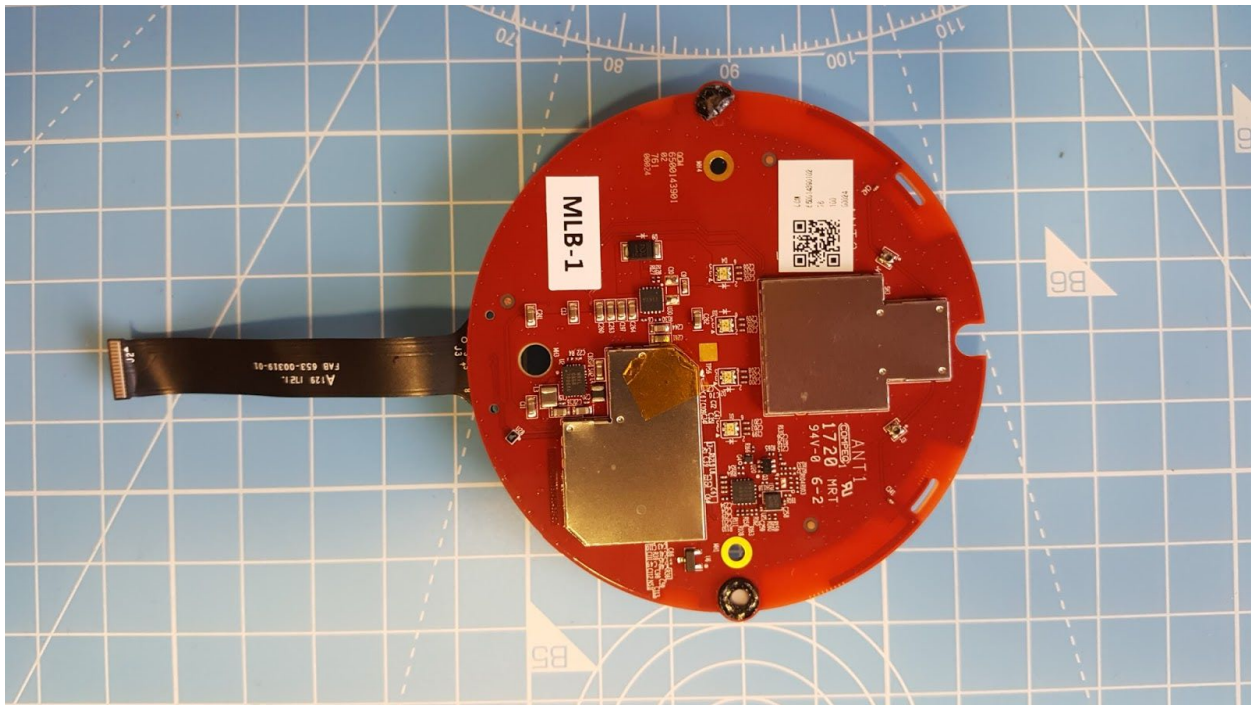
Top View PCB, Shield Cans Removed
