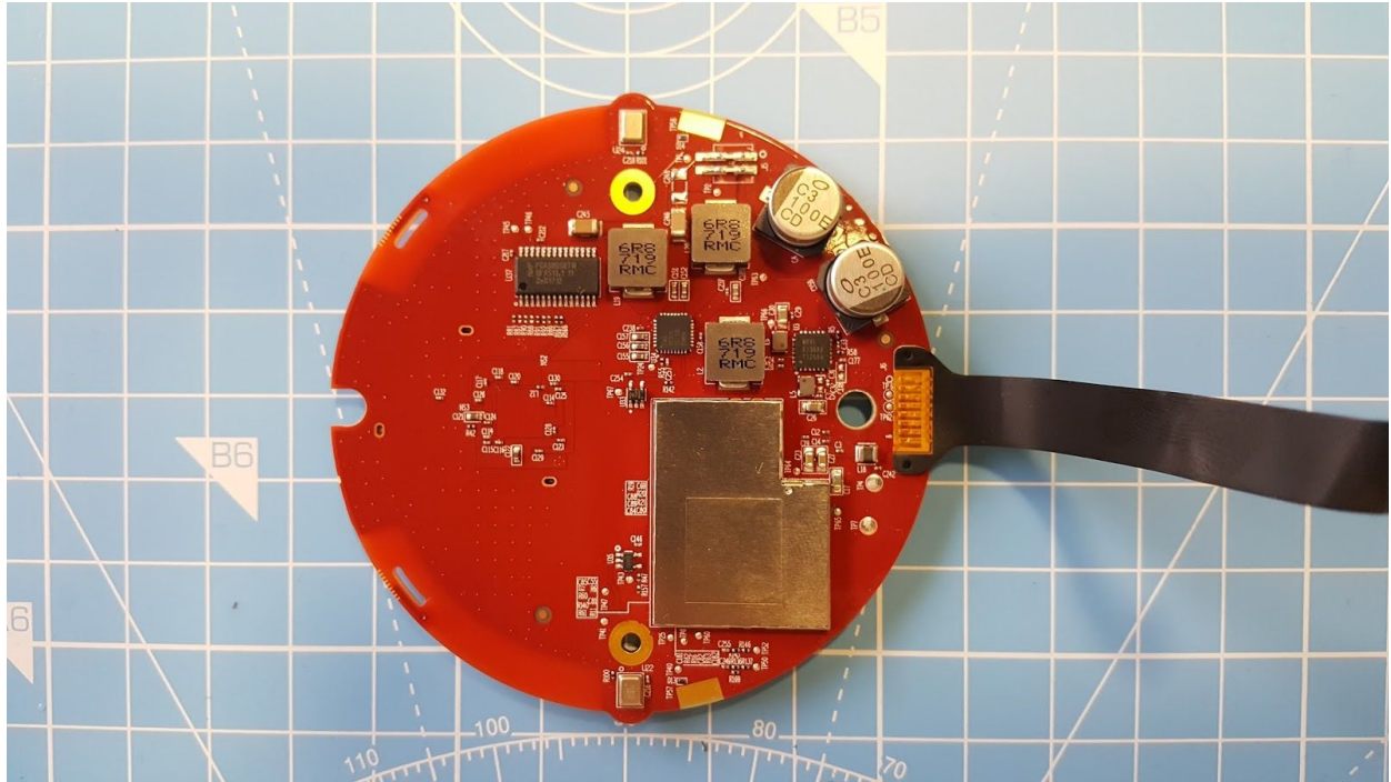
Bottom View PCB
