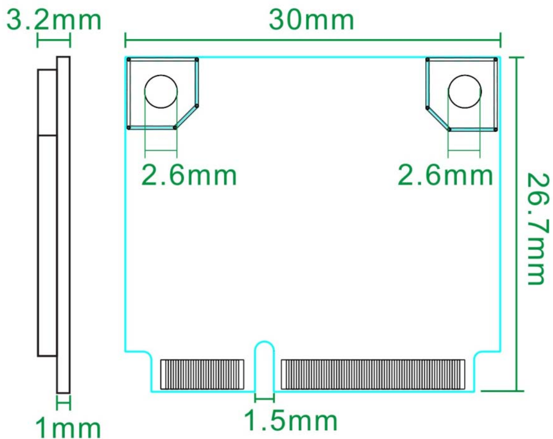
Figure 5 Top View
