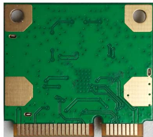
Figure 2 Bottom View
