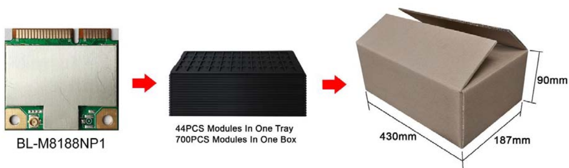
Figure 6 Package Information
