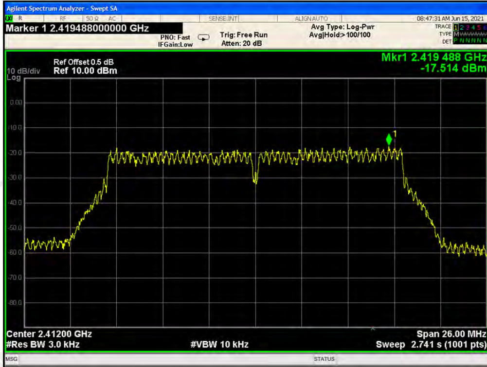
CH1: 2412MHz
