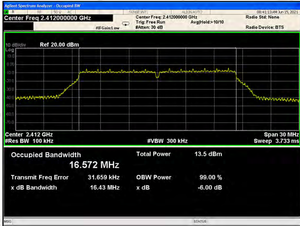
CH1: 2412MHz
