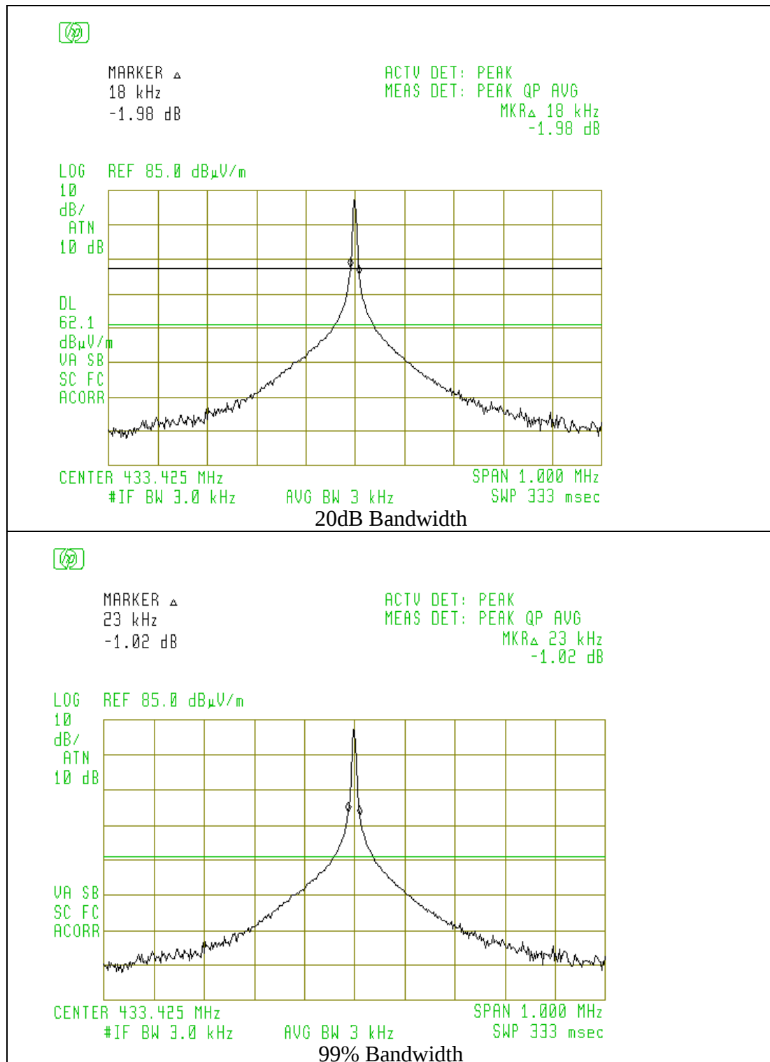
Figure 6.1 Occupied Bandwidth
