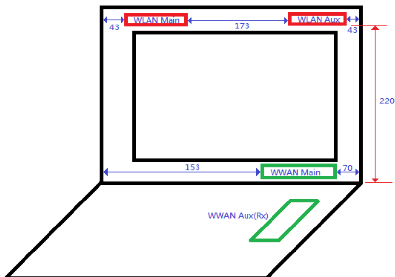
Photograph 5. Antenna position of EUT
