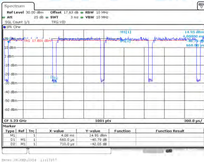
NTNV-11AC40-CDD-Ant3-5230
