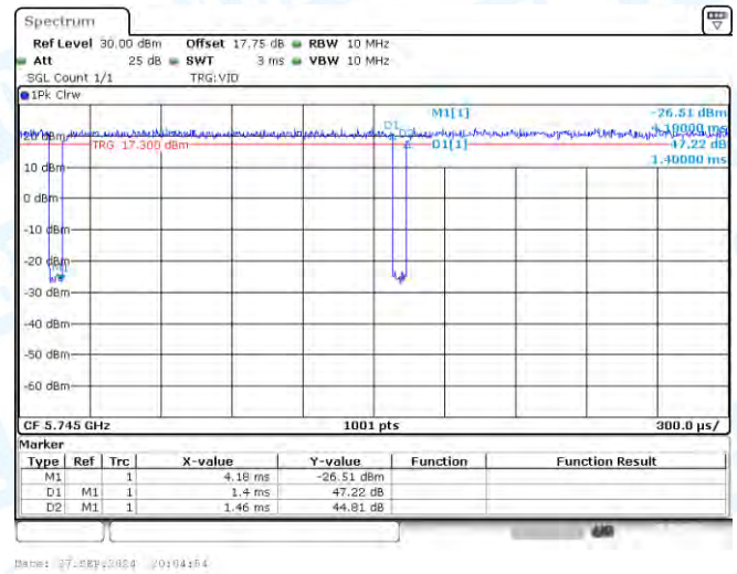
NTNV-11A-CDD-Ant1-5745
