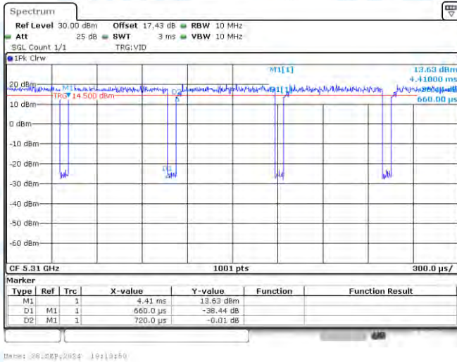
NTNV-11AC40-CDD-Ant1-5310
