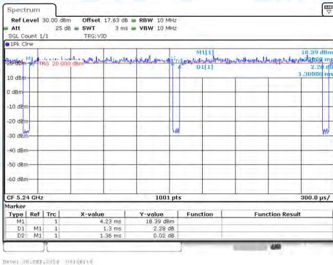
NTNV-11N20-CDD-Ant3-5240
