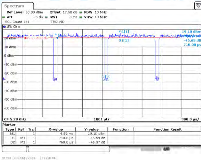
NTVN-11A-Ant3-5280
