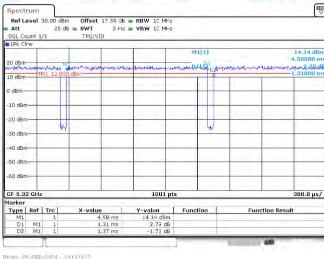
NTNV-11AC20-CDD-Ant3-5320
