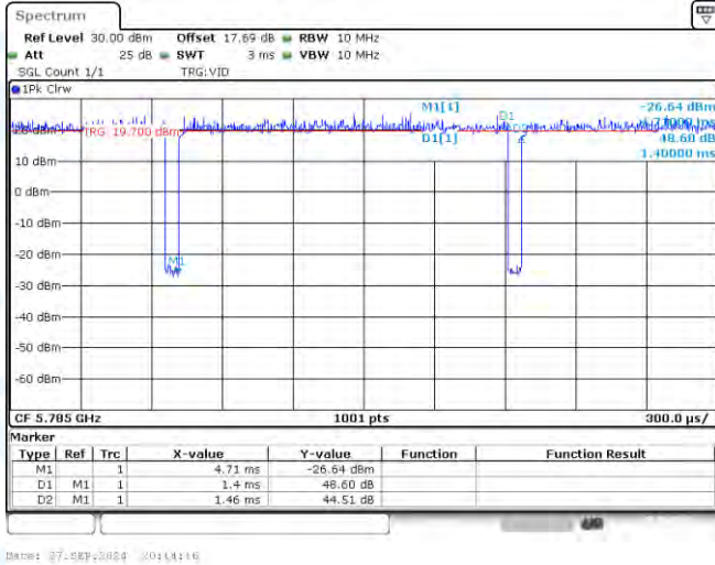
NTNV-11A-CDD-Ant1-5785
