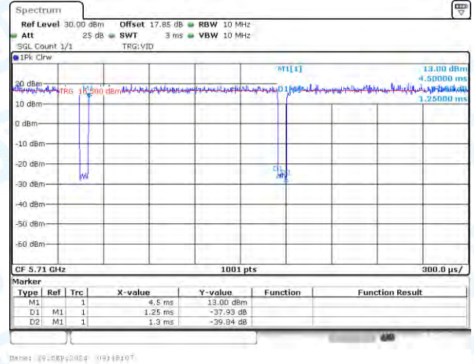
NTNV-11N40-CDD-Ant2-5710
