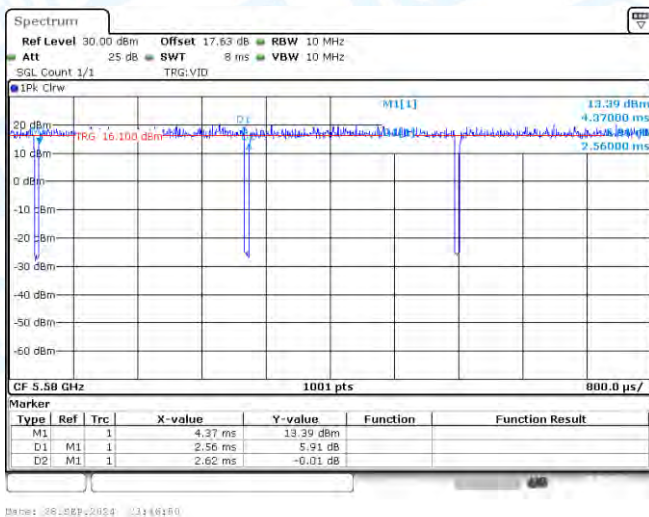
NTNV-11N20-CDD-Ant2-5580
