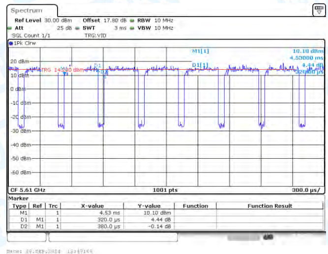
NTNV-11AC80-CDD-Ant3-5610
