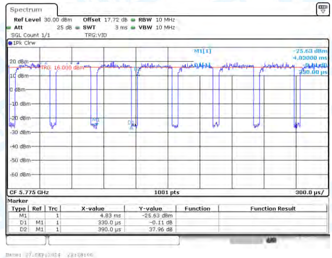
NTNV-11AC80-CDD-Ant1-5775
