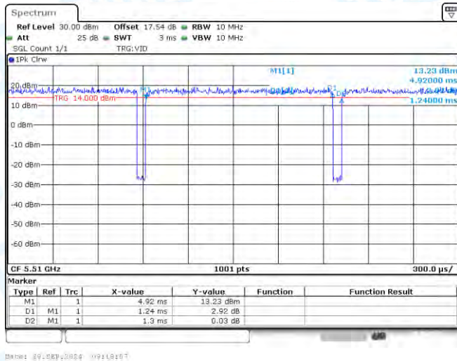
NTNV-11N40-CDD-Ant1-5510
