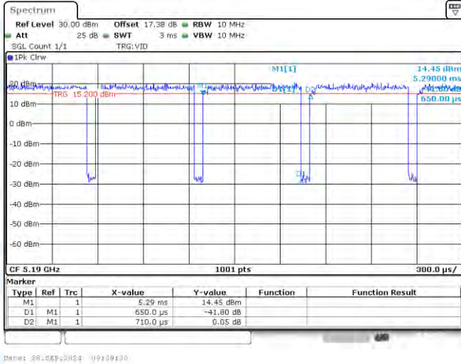
NTNV-11N40-CDD-Ant1-5190
