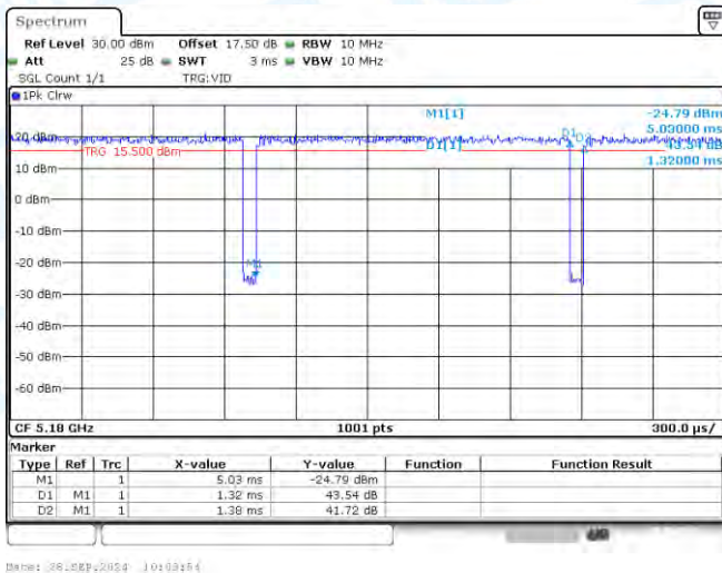
NTNV-11AC20-CDD-Ant2-5180
