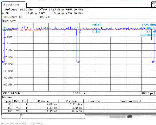
NTNV-11A-CDD-Ant3-5240
