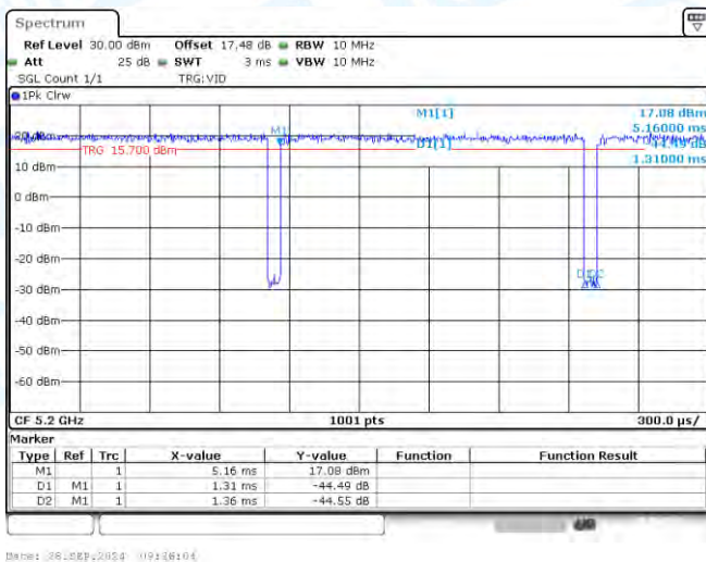
NTNV-11N20-CDD-Ant2-5200
