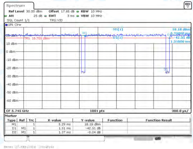
NTNV-11N20-CDD-Ant3-5745
