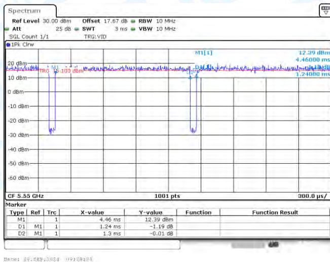
NTNV-11N40-CDD-Ant2-5550
