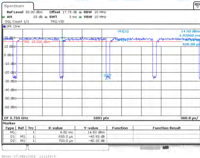
NTNV-11N40-CDD-Ant2-5755
