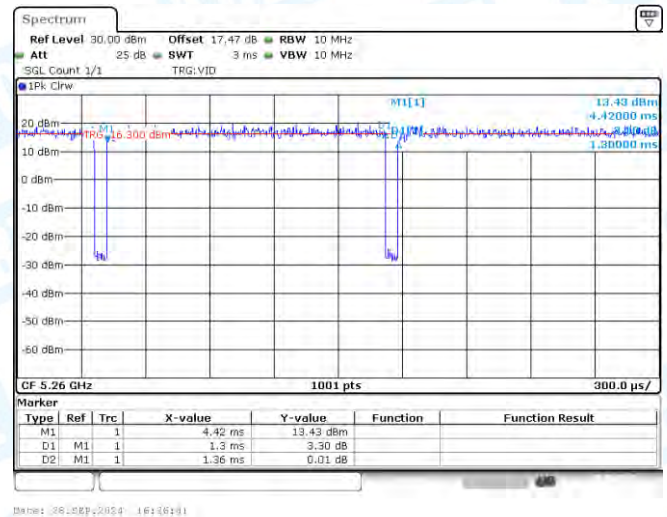
NTNV-11N20-CDD-Ant1-5260
