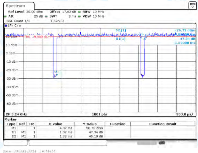
NTNV-11AC20-CDD-Ant3-5240
