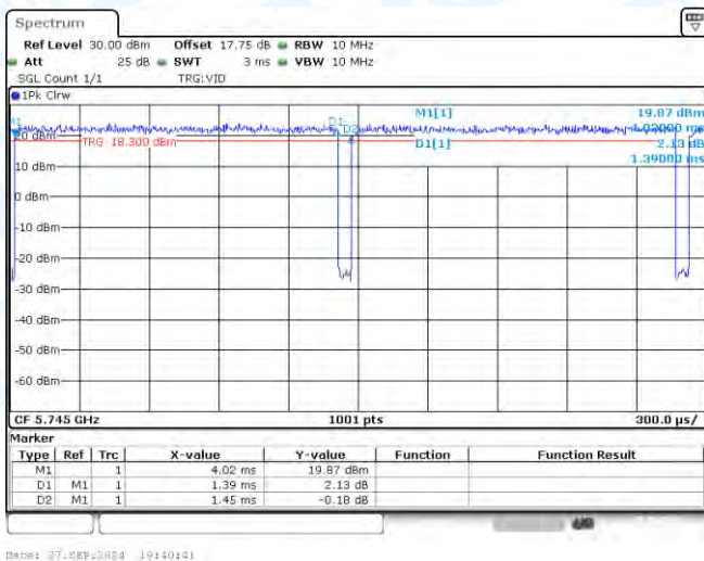
NTVN-11A-Ant2-5745
