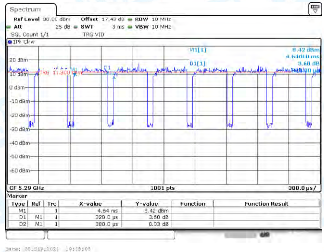
NTNV-11AC80-CDD-Ant1-5290
