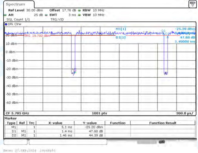
NTNV-11A-Ant2-5785
