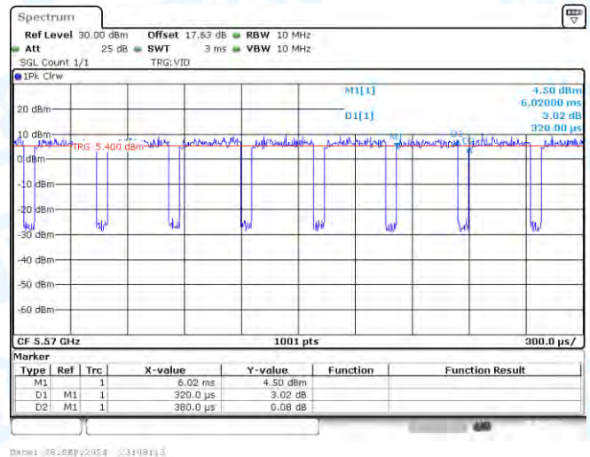
NTNV-11AC160-CDD-Ant2-5570
