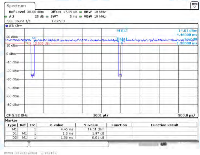
NTNV-11N20-CDD-Ant3-5320
