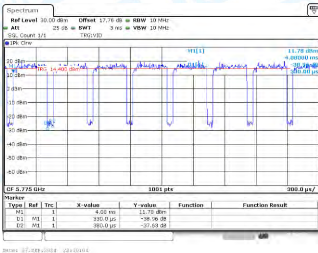
NTNV-11AC80-CDD-Ant2-5775
