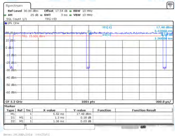
NTNV-11N20-CDD-Ant3-5200
