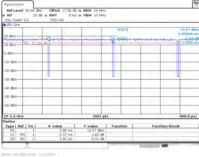
NTNV-11N20-CDD-Ant1-5500
