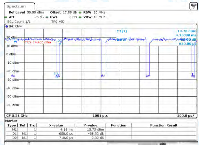
NTNV-11N40-CDD-Ant1-5310
