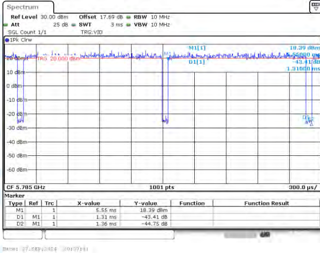
NTNV-11N20-CDD-Ant1-5785
