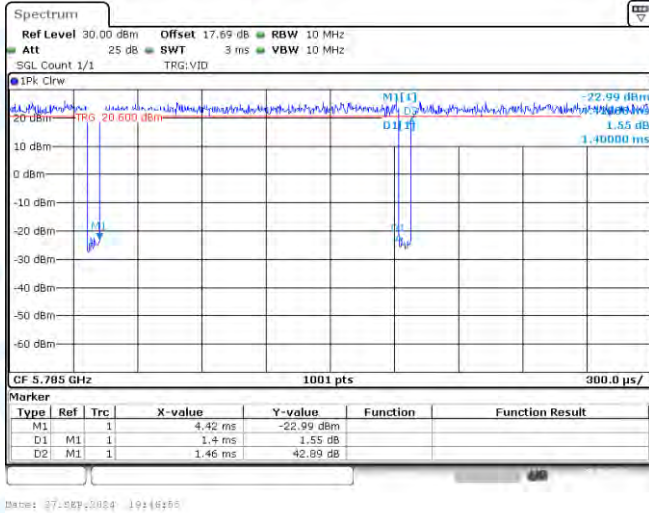
NTNV-11A-Ant1-5785
