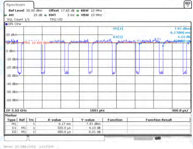
NTNV-11AC80-CDD-Ant2-5530
