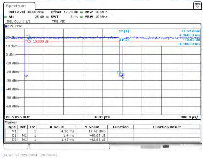
NTNV-11A-CDD-Ant1-5825
