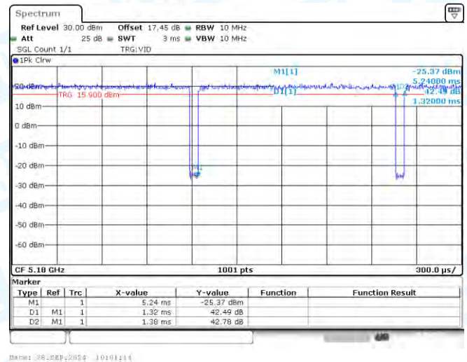
NTNV-11AC20-CDD-Ant1-5180
