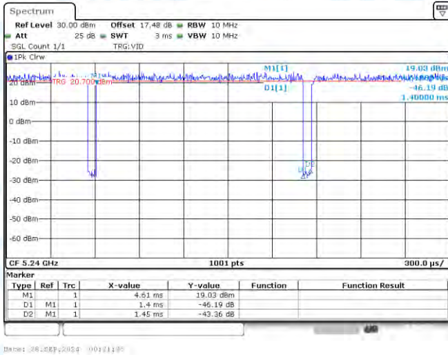
NTVN-11A-Ant1-5240
