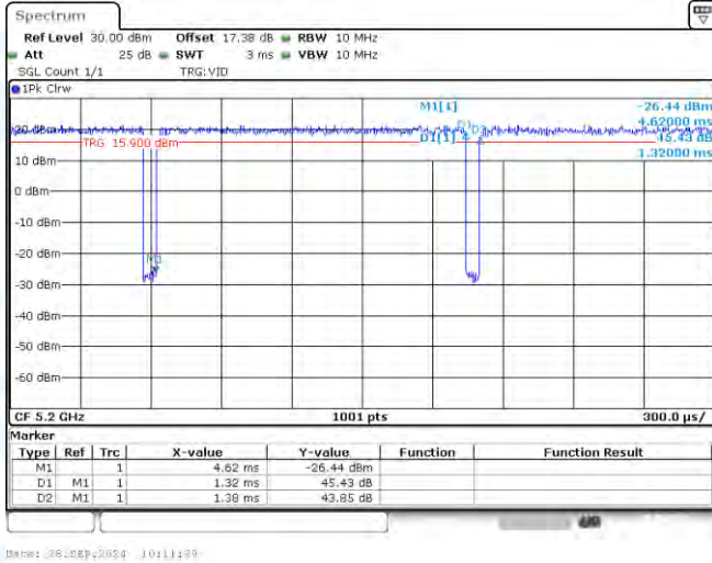
NTNV-11AC20-CDD-Ant1-5200
