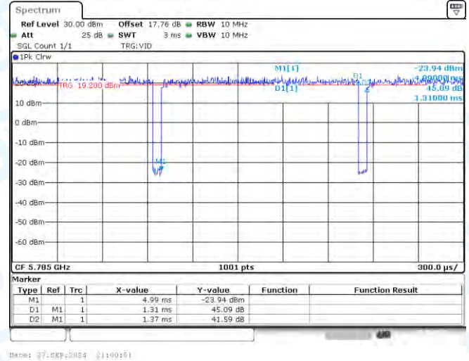
NTNV-11N20-CDD-Ant2-5785
