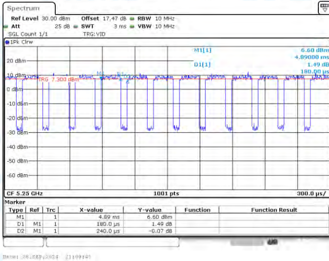
NTNV-11AC160-CDD-Ant1-5250
