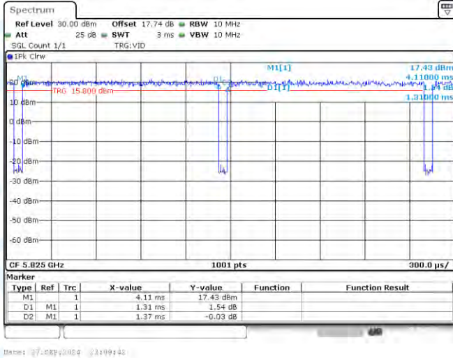
NTNV-11AC20-CDD-Ant1-5825
