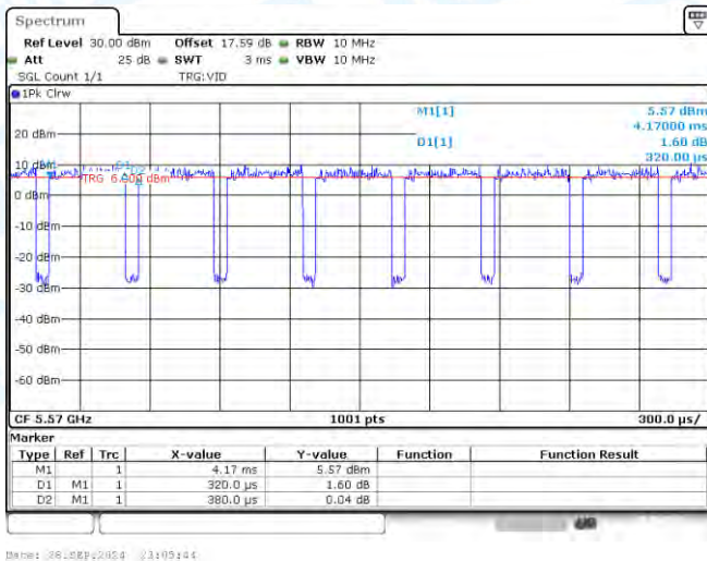
NTNV-11AC160-CDD-Ant1-5570
