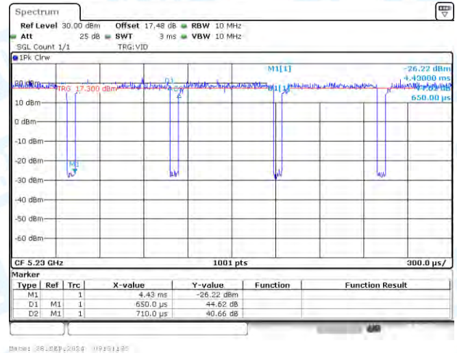
NTNV-11N40-CDD-Ant1-5230
