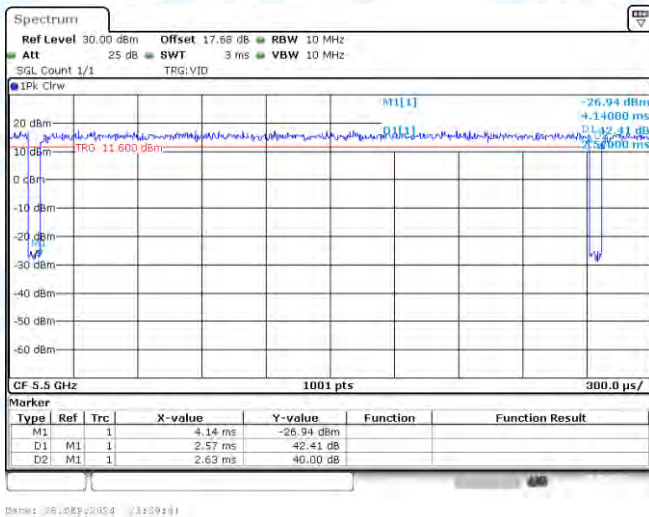
NTNV-11N20-CDD-Ant3-5500
