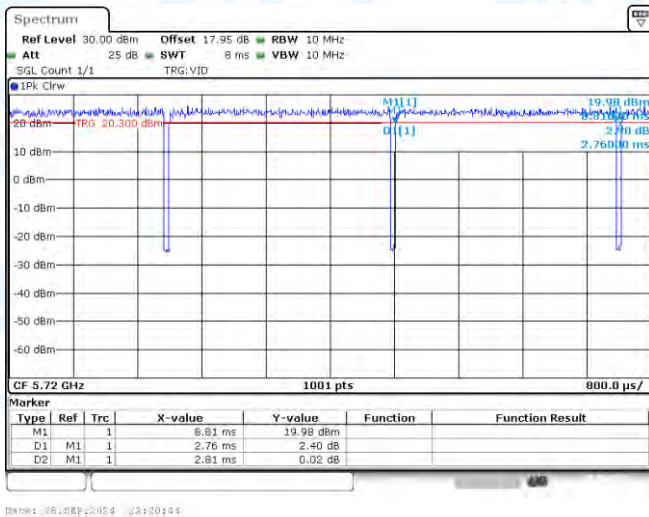
NTVN-11A-Ant3-5720
