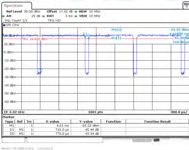
NTVN-11A-Ant2-5320
