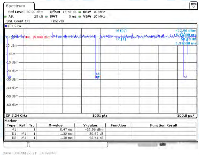
NTNV-11AC20-CDD-Ant1-5240
