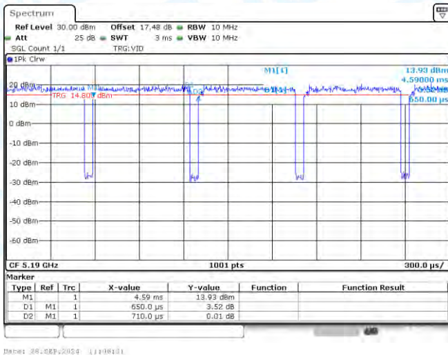
NTNV-11AC40-CDD-Ant2-5190
