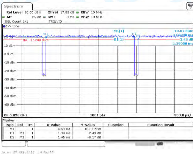
NTNV-11A-Ant2-5825
