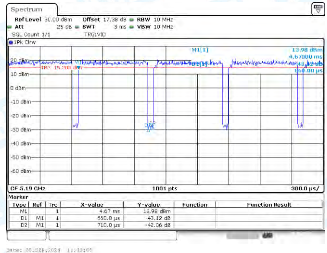
NTNV-11AC40-CDD-Ant1-5190
