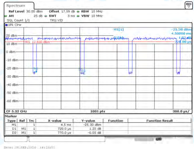
NTNV-11A-CDD-Ant3-5320
