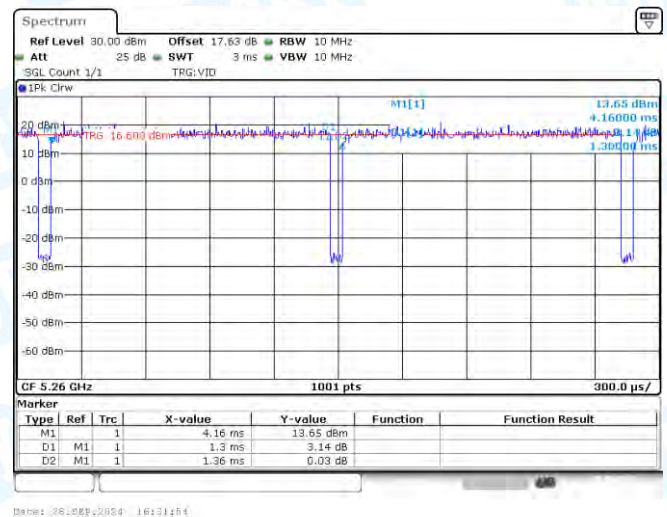
NTNV-11N20-CDD-Ant3-5260
