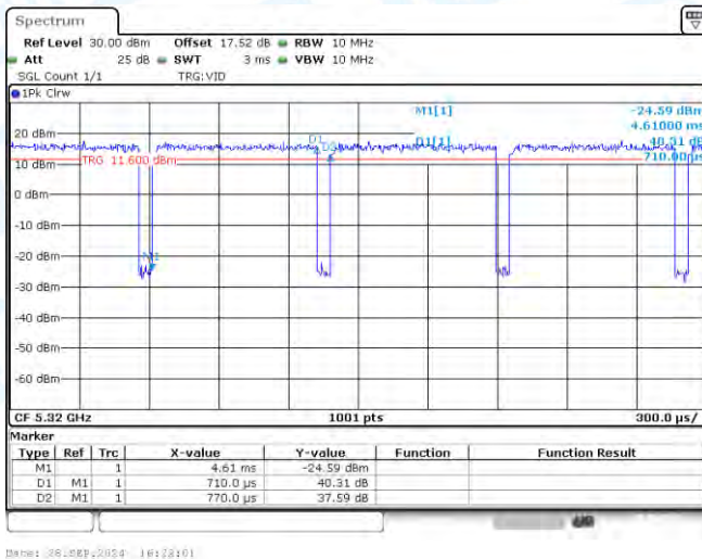
NTNV-11A-CDD-Ant2-5320
