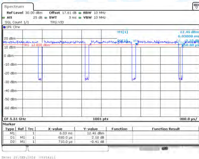
NTNV-11AC40-CDD-Ant2-5510
