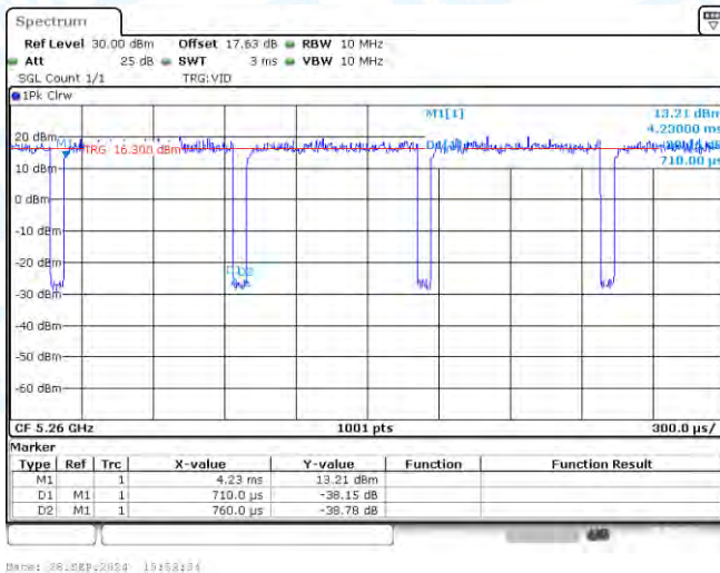
NTNV-11A-CDD-Ant3-5260
