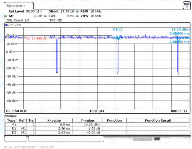
NTNV-11N20-CDD-Ant1-5580
