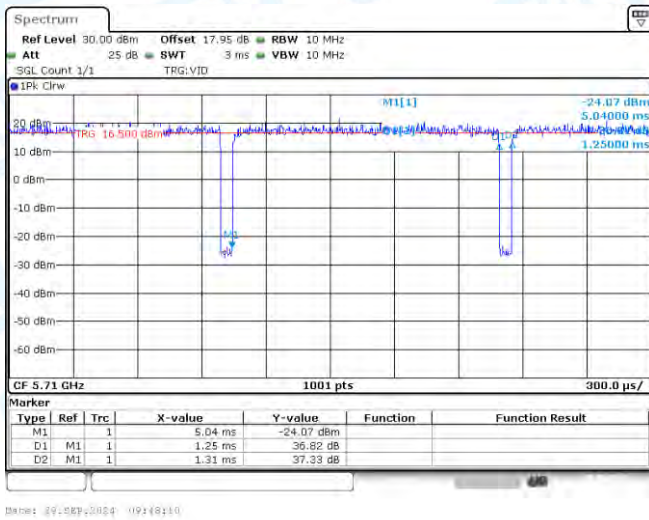
NTNV-11N40-CDD-Ant3-5710
