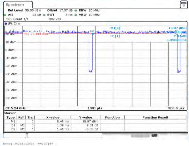
NTVN-11A-Ant2-5240
