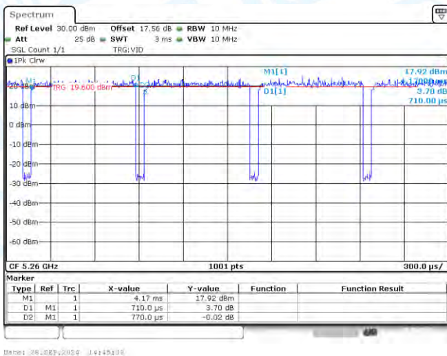
NTVN-11A-Ant2-5260
