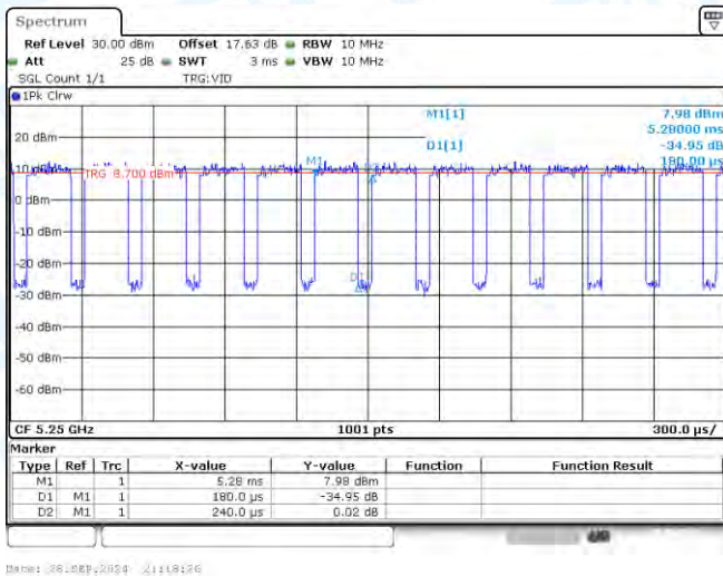
NTNV-11AC160-CDD-Ant3-5250
