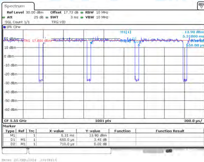
NTNV-11AC40-CDD-Ant3-5550
