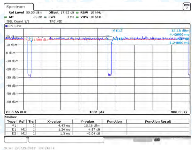
NTNV-11N40-CDD-Ant1-5550
