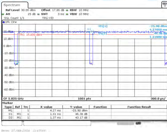
NTNV-11N20-CDD-Ant2-5825
