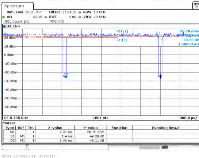
NTNV-11A-Ant3-5785
