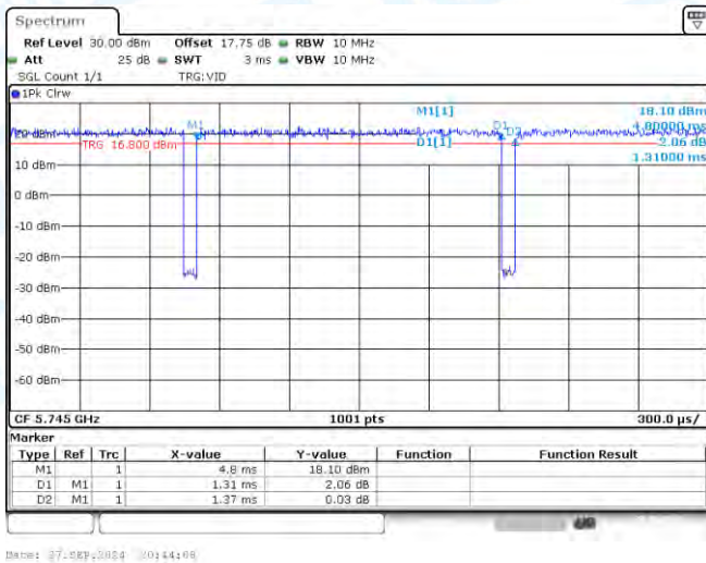
NTNV-11N20-CDD-Ant2-5745
