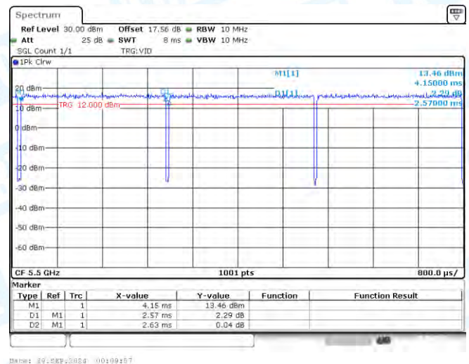
NTNV-11AC20-CDD-Ant1-5500
