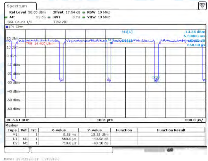
NTNV-11AC40-CDD-Ant1-5510
