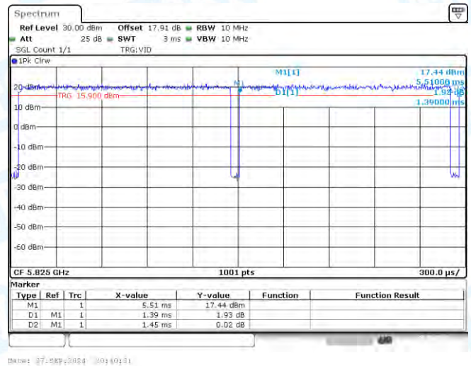
NTNV-11A-CDD-Ant3-5825
