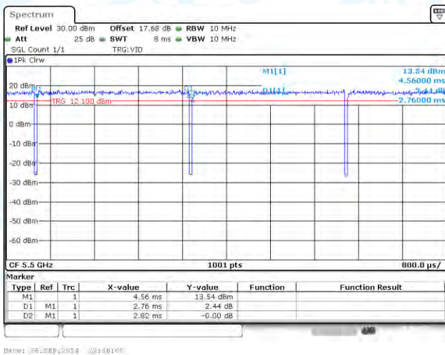
NTNV-11A-CDD-Ant3-5500
