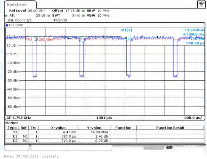
NTNV-11N40-CDD-Ant2-5795
