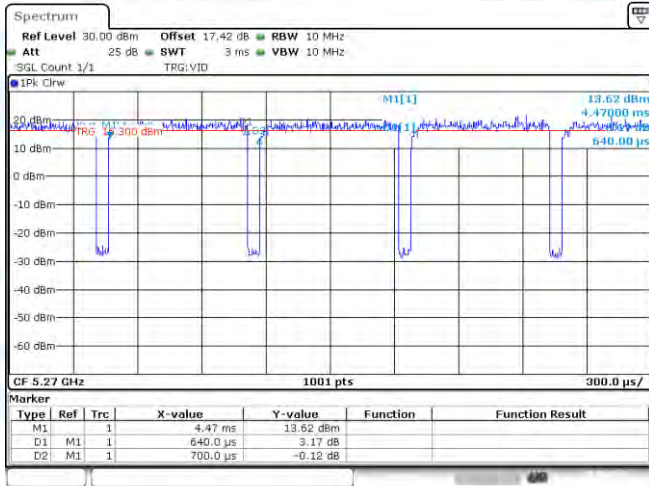
NTNV-11N40-CDD-Ant1-5270
