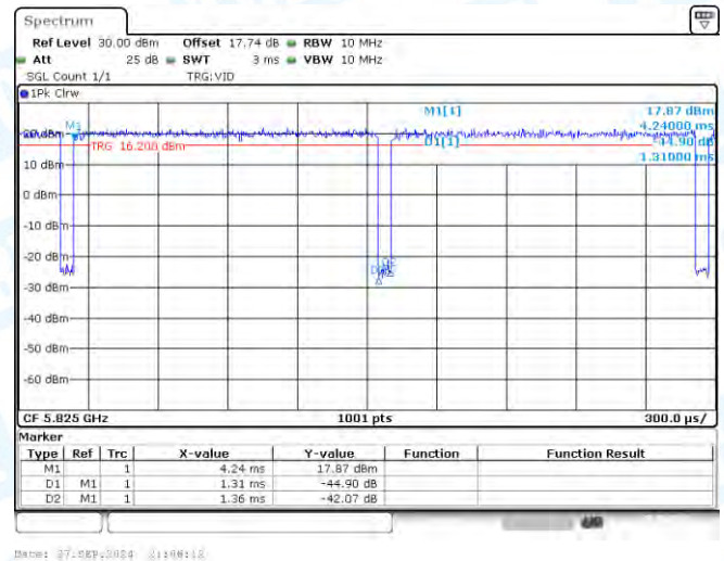
NTNV-11N20-CDD-Ant1-5825
