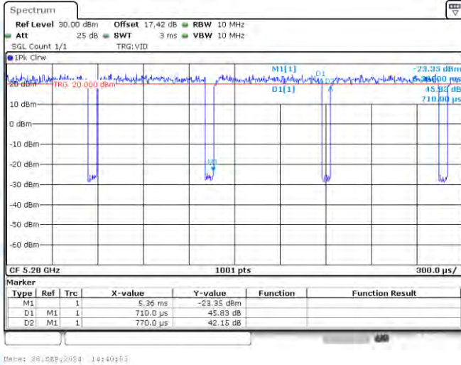
NTVN-11A-Ant1-5280
