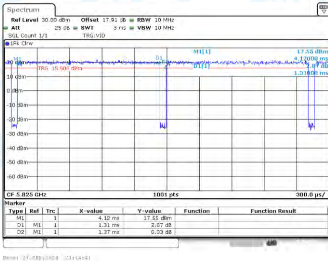
NTNV-11AC20-CDD-Ant3-5825
