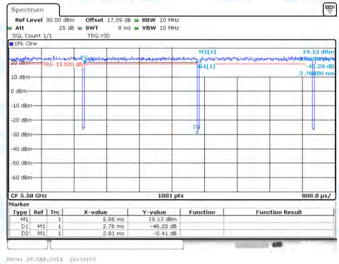
NTVN-11A-Ant1-5580
