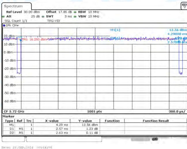
NTNV-11AC20-CDD-Ant2-5720
