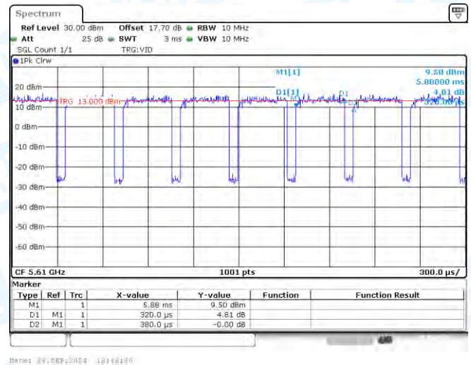
NTNV-11AC80-CDD-Ant1-5610
