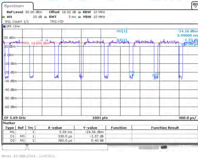
NTNV-11AC80-CDD-Ant3-5690
