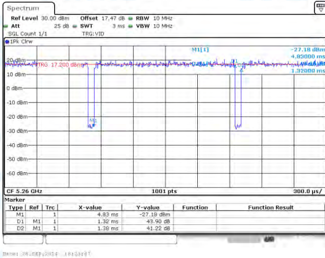
NTNV-11AC20-CDD-Ant1-5260
