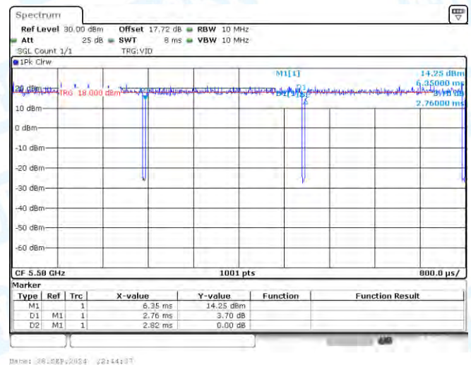
NTNV-11A-CDD-Ant3-5580
