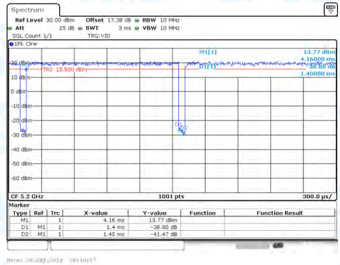
NTNV-11A-CDD-Ant1-5200
