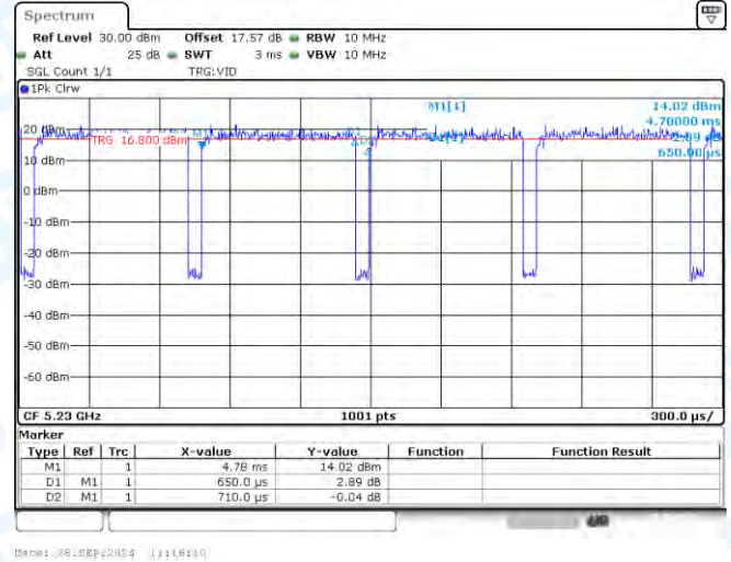
NTNV-11AC40-CDD-Ant2-5230
