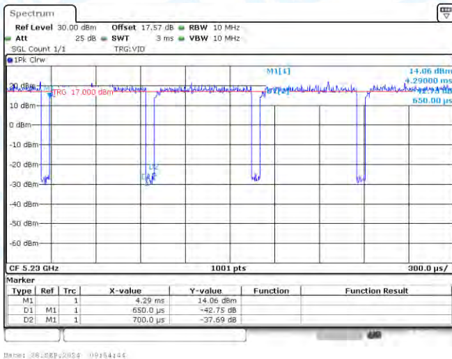
NTNV-11N40-CDD-Ant2-5230
