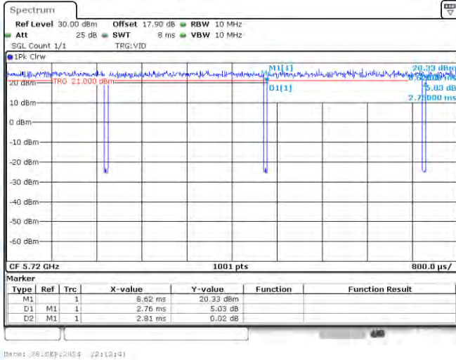
NTVN-11A-Ant1-5720
