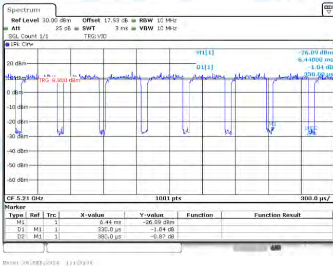
NTNV-11AC80-CDD-Ant3-5210
