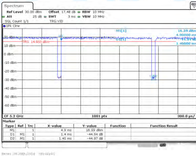
NTNV-11A-CDD-Ant2-5200
