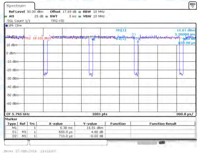
NTNV-11AC40-CDD-Ant1-5795
