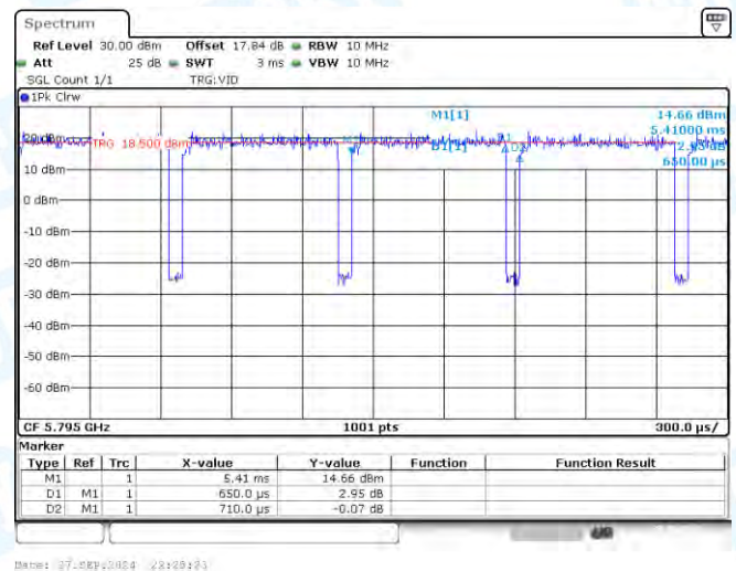
NTNV-11AC40-CDD-Ant3-5795
