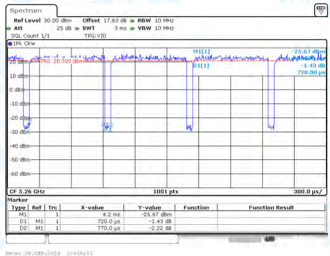
NTVN-11A-Ant3-5260
