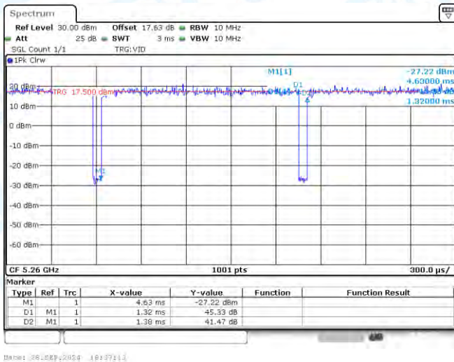
NTNV-11AC20-CDD-Ant3-5260
