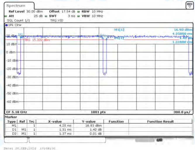
NTNV-11AC20-CDD-Ant3-5180
