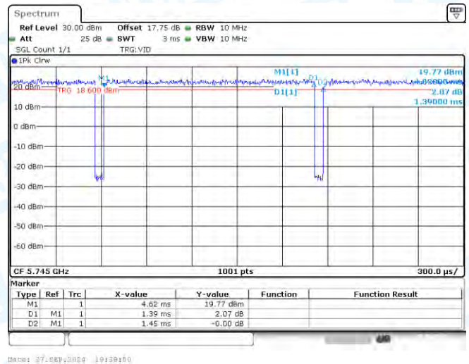
NTVN-11A-Ant1-5745
