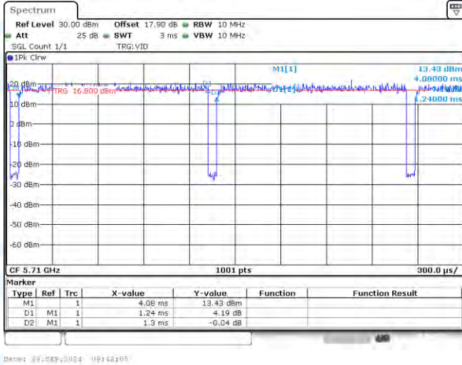
NTNV-11N40-CDD-Ant1-5710
