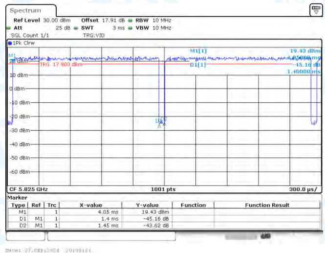
NTNV-11A-Ant3-5825
