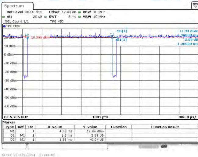
NTNV-11N20-CDD-Ant3-5785
