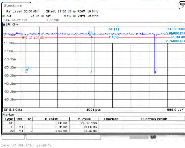
NTVN-11A-Ant3-5500
