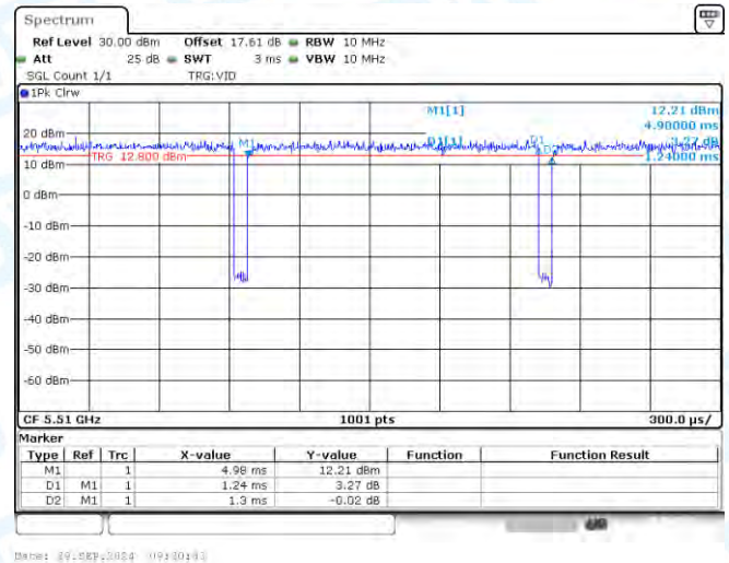
NTNV-11N40-CDD-Ant2-5510
