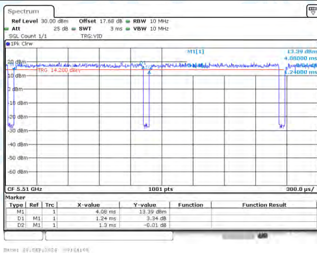
NTNV-11N40-CDD-Ant3-5510
