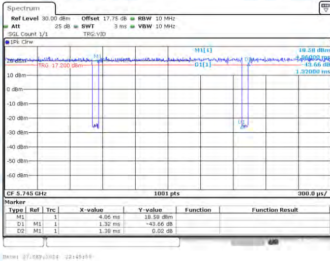
NTNV-11AC20-CDD-Ant1-5745
