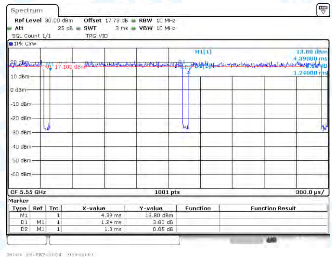
NTNV-11N40-CDD-Ant3-5550
