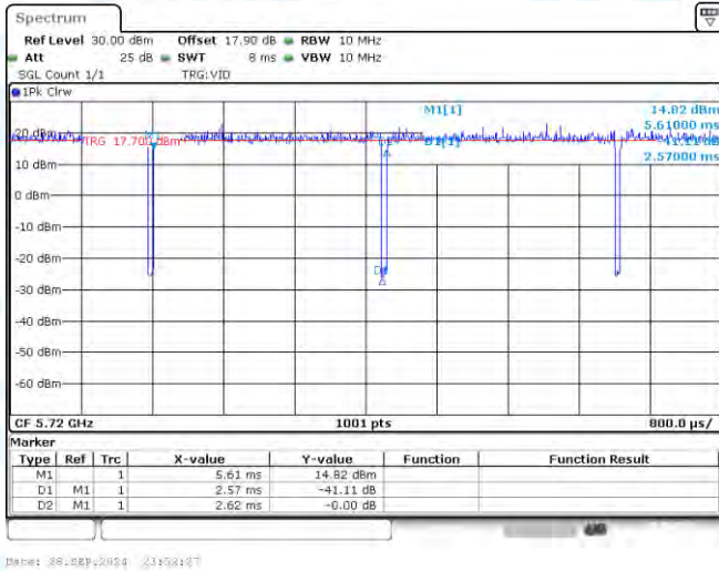
NTNV-11N20-CDD-Ant1-5720
