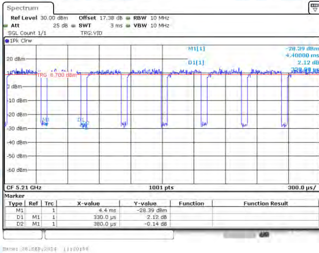
NTNV-11AC80-CDD-Ant1-5210
