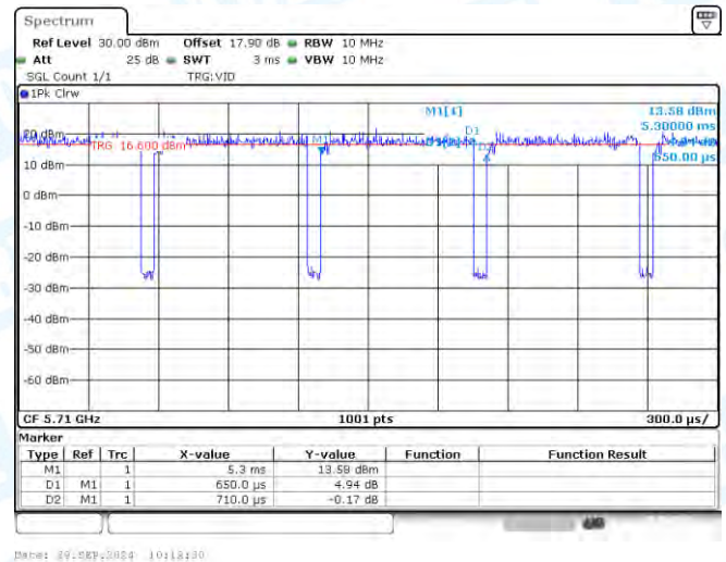
NTNV-11AC40-CDD-Ant1-5710
