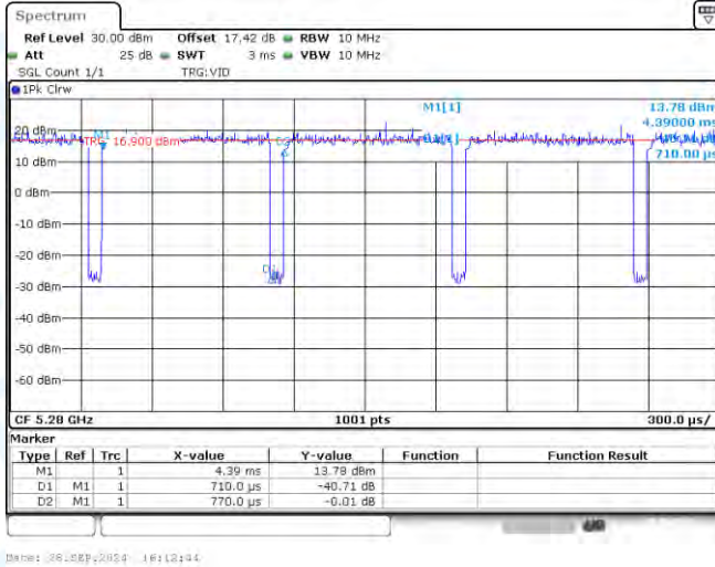
NTNV-11A-CDD-Ant1-5280
