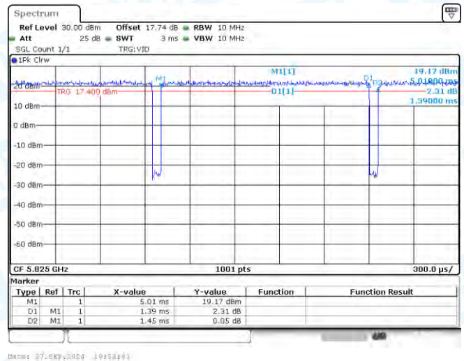
NTNV-11A-Ant1-5825
