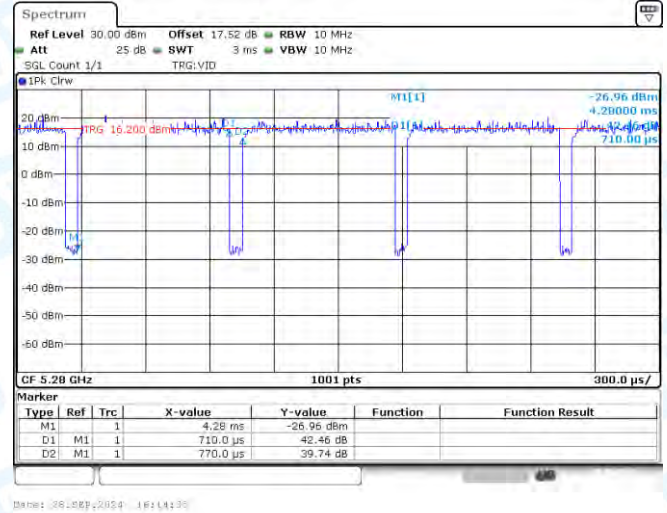
NTNV-11A-CDD-Ant2-5280
