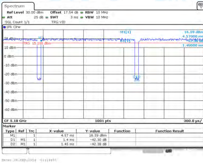
NTNV-11A-CDD-Ant3-5180
