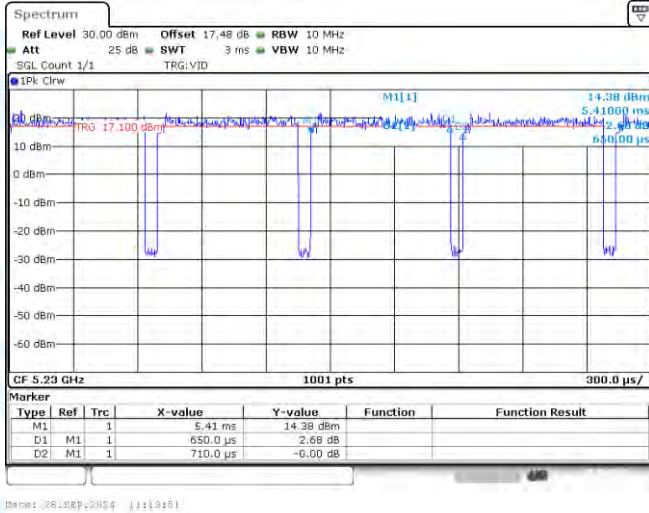
NTNV-11AC40-CDD-Ant1-5230
