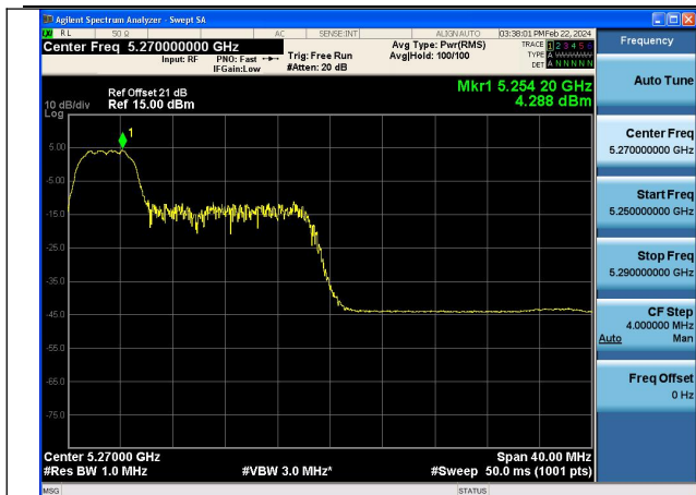
Mode:802.11ax HE40 Tone:52T Frequency:5270MHz Ant:Chain1
