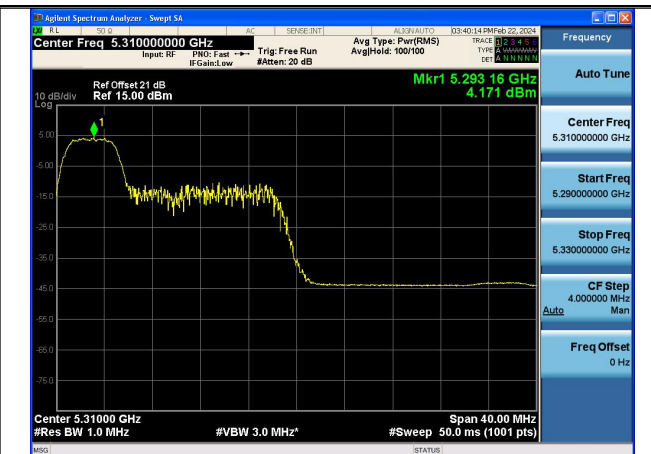
Mode:802.11ax HE40 Tone:52T Frequency:5310MHz Ant:Chain1
