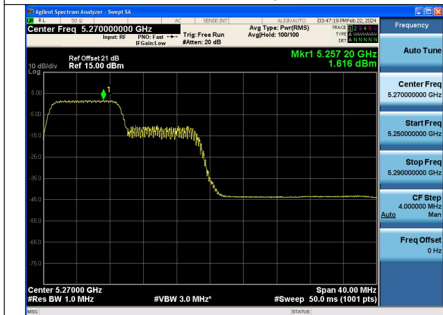
Mode:802.11ax HE40 Tone:106T Frequency:5270MHz Ant:Chain1
