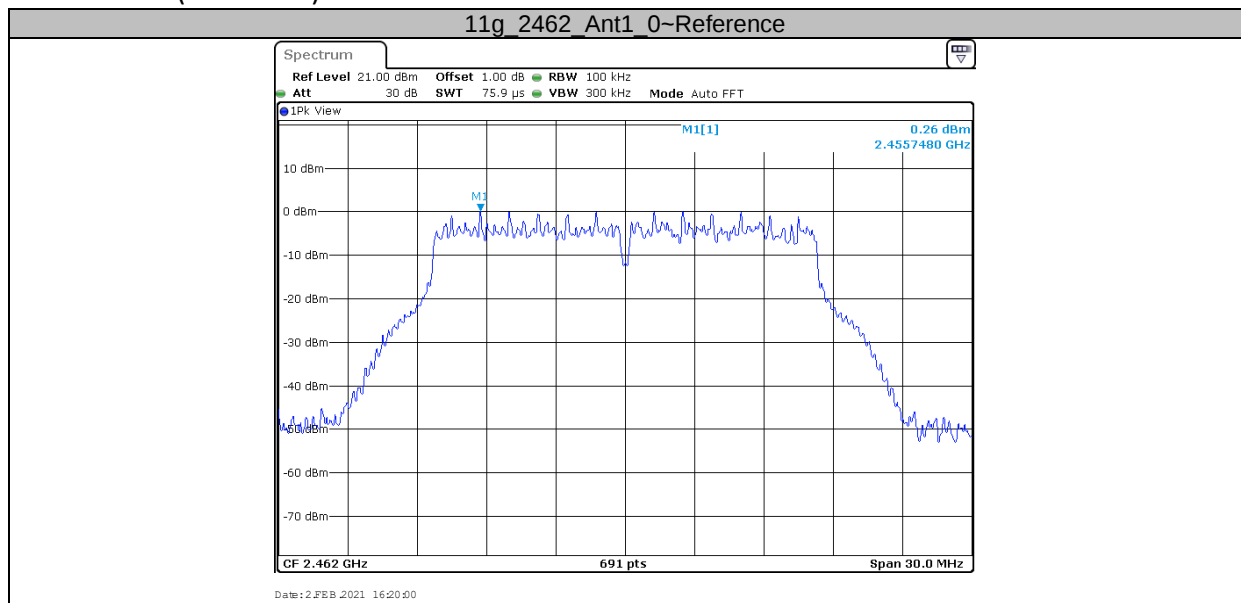
Channel 11 (2462MHz) Reference Level: 0.26dBm
