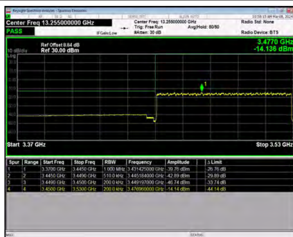
n77(3450-3550) SCS=30kHz DFT_64QAM BW=80MHz LowChannel=632668 RB=216@0
