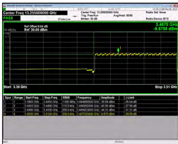
n77(3450-3550) SCS=30kHz DFT_BPSK BW=60MHz LowChannel=632000 RB=162@0
