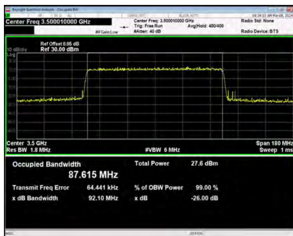
n77(3450-3550) SCS=30kHz CP_64QAM BW=90MHz Channel=633334 RB=245@0
