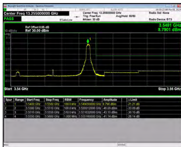
n77(3450-3550) SCS=30kHz DFT_BPSK BW=10MHz HighChannel=636332 RB=1@23
