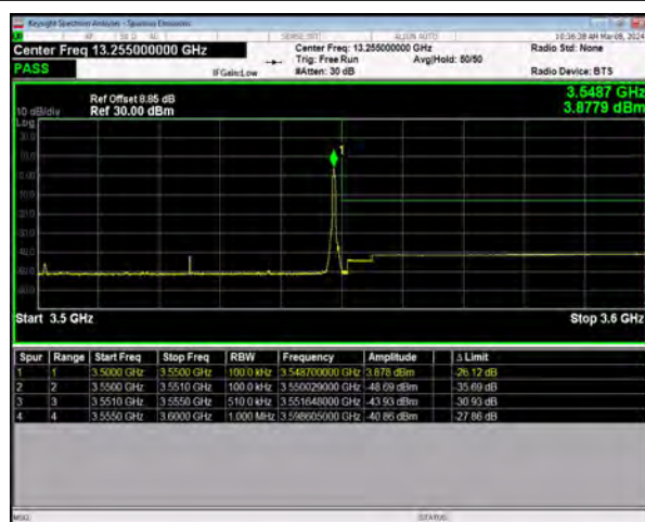
n77(3450-3550) SCS=30kHz DFT_256QAM BW=50MHz HighChannel=635000 RB=1@132
