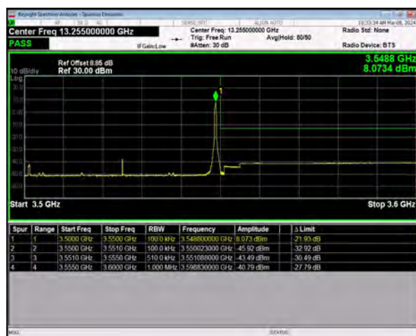
n77(3450-3550) SCS=30kHz DFT_BPSK BW=50MHz HighChannel=635000 RB=1@132
