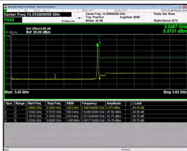
n77(3450-3550) SCS=30kHz DFT_64QAM BW=70MHz HighChannel=634332 RB=1@188
