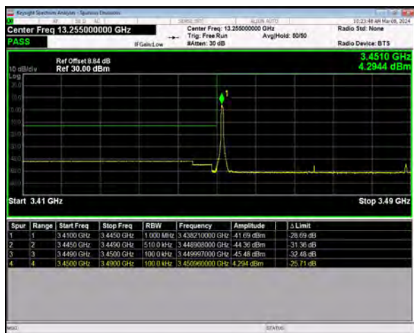
n77(3450-3550) SCS=30kHz DFT_256QAM BW=40MHz LowChannel=631334 RB=1@0
