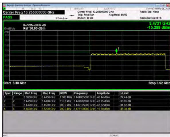
n77(3450-3550) SCS=30kHz DFT_256QAM BW=70MHz LowChannel=632334 RB=180@0
