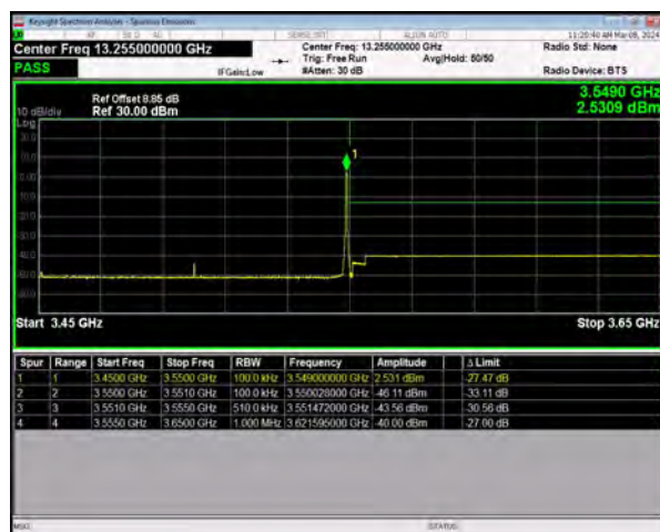
n77(3450-3550) SCS=30kHz DFT_256QAM BW=100MHz HighChannel=633334 RB=1@272
