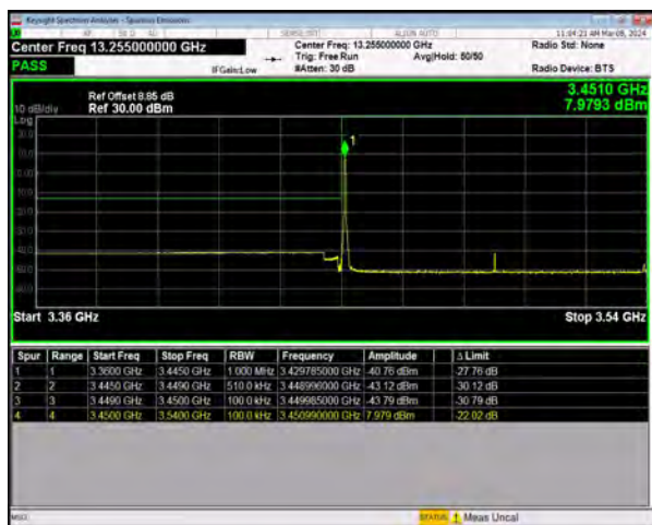
n77(3450-3550) SCS=30kHz DFT_BPSK BW=90MHz LowChannel=633000 RB=1@0
