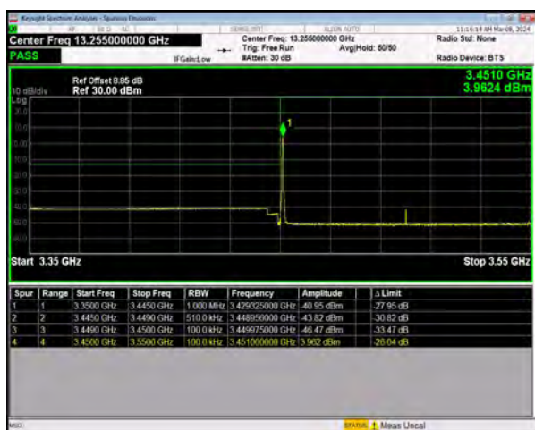
n77(3450-3550) SCS=30kHz DFT_256QAM BW=100MHz LowChannel=633334 RB=1@0
