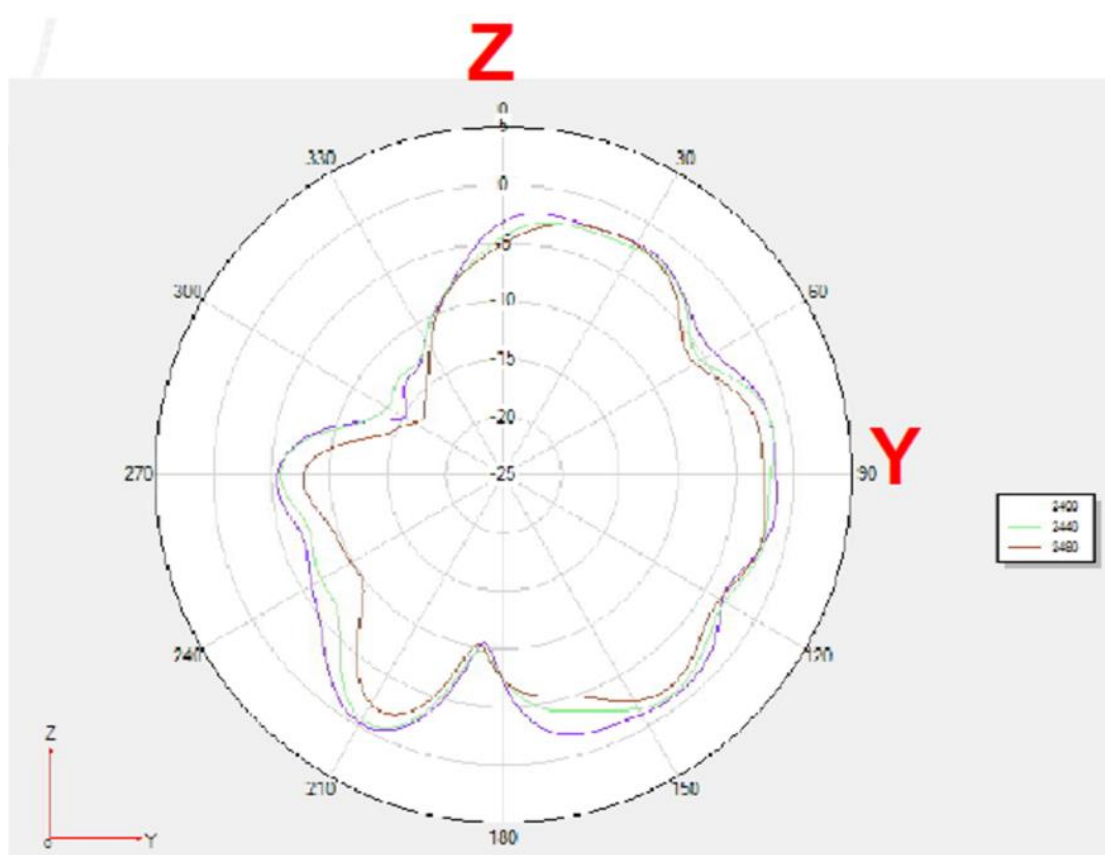
GFSK Antenna
