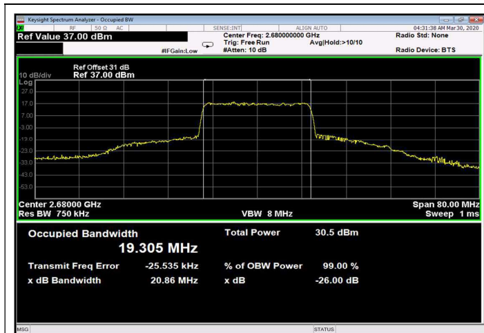
Figure 375: 64QAM 20MHz B.W.; 2680.0MHz, 15kHz Output
