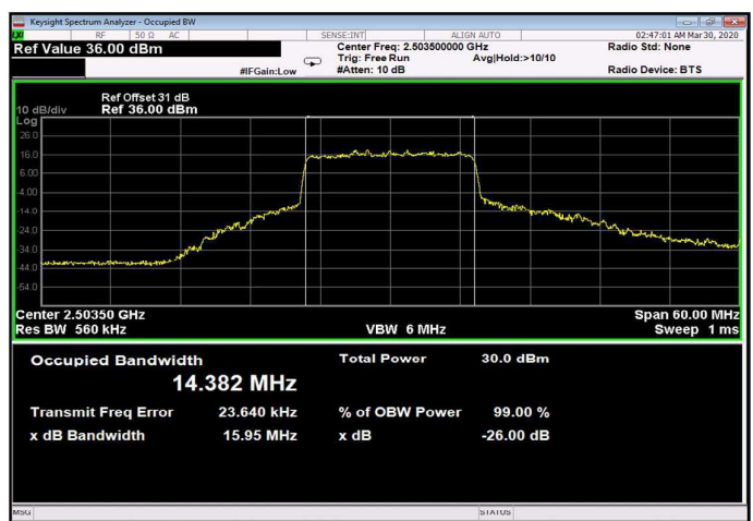
Figure 360: 64QAM 15MHz B.W.; 2503.5MHz, 15kHz Output
