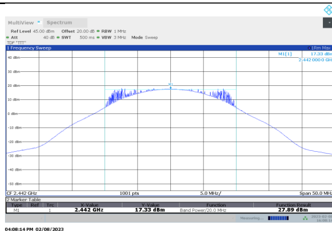
Figure 8.3-11: TSM-Bandwidth 20MHz Conducted output power, 2442 MHz
