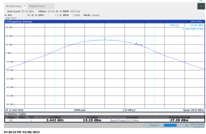
Figure 8.3-8: TSM-Bandwidth 10MHz Conducted output power, 2442 MHz
