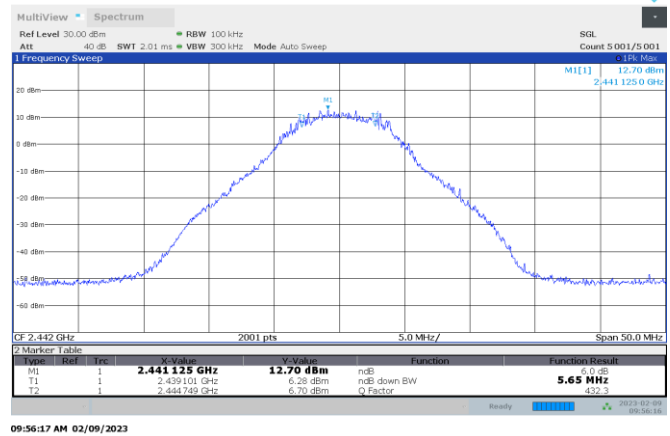
Figure 8.2-8: TSM Bandwidth 10MHz 6dB DTS bandwidth, 2442 MHz
