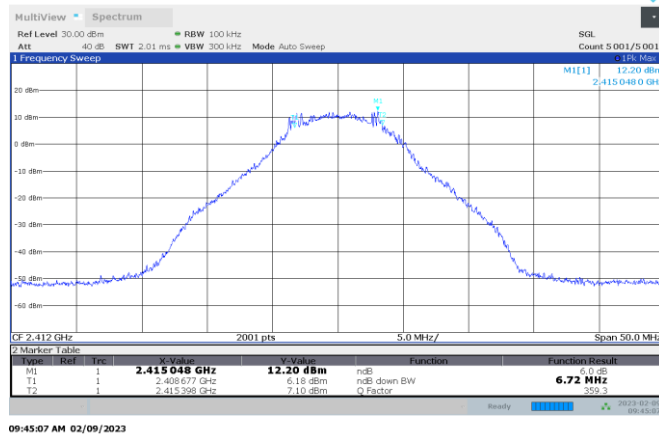
Figure 8.2-7: TSM Bandwidth 10MHz 6dB DTS bandwidth, 2412 MHz
