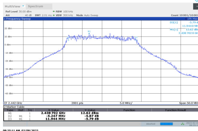
Figure 8.2-11: TSM Bandwidth 20MHz 6dB DTS bandwidth, 2442 MHz
