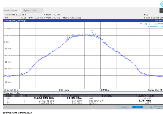
Figure 8.2-9: TSM Bandwidth 10MHz 6dB DTS bandwidth, 2465 MHz
