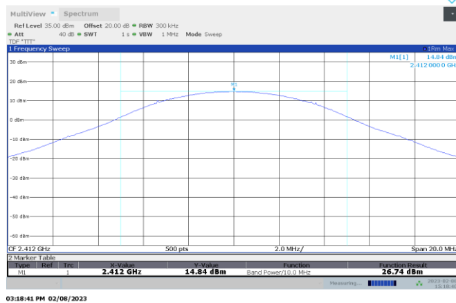
Figure 8.3-7: TSM-Bandwidth 10MHz Conducted output power, 2412 MHz
