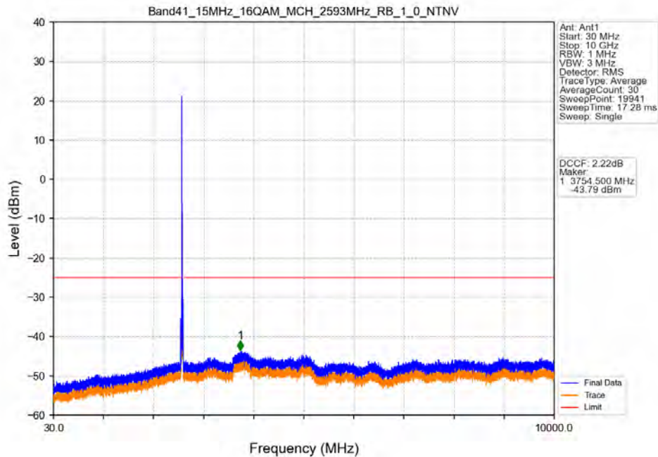
Band41_15MHz_16QAM_MCH_2593MHz_RB_1_0_NTNV
