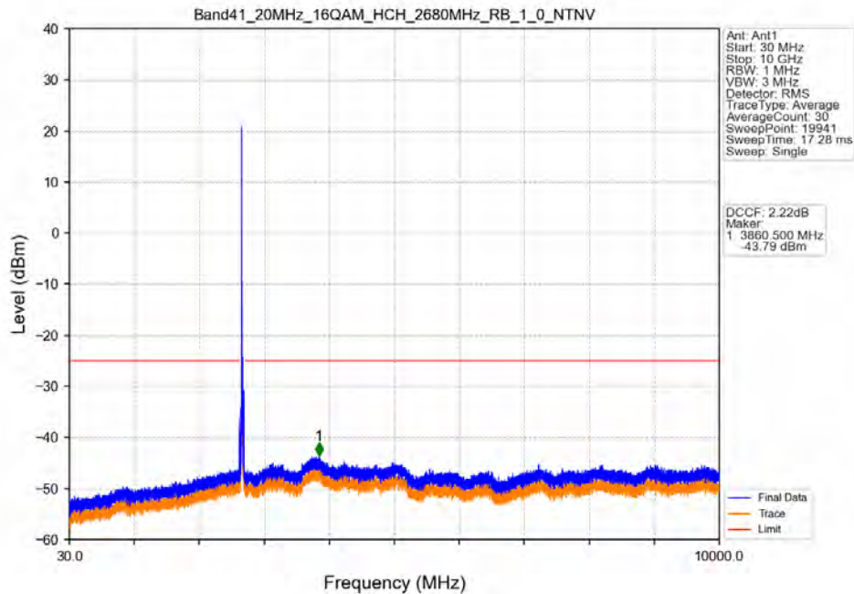
Band41_20MHz_16QAM_HCH_2680MHz_RB_1_0_NTNV
