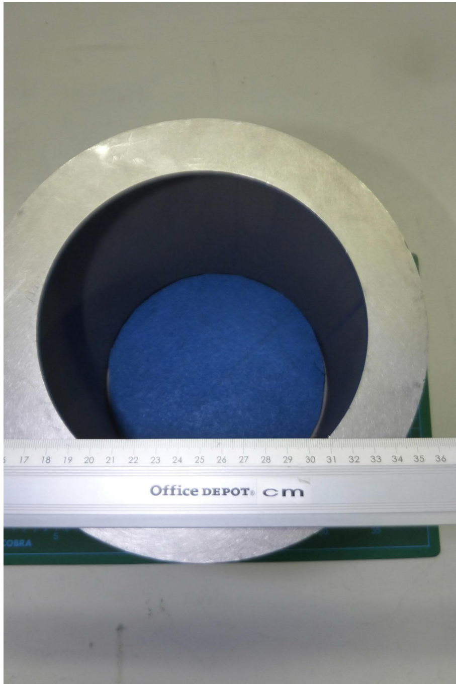
EUT 2, used tank, top view
