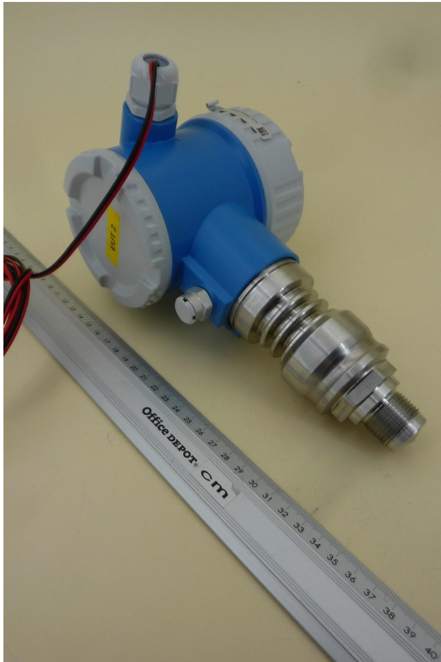
EUT 2, 3-D-view 1
