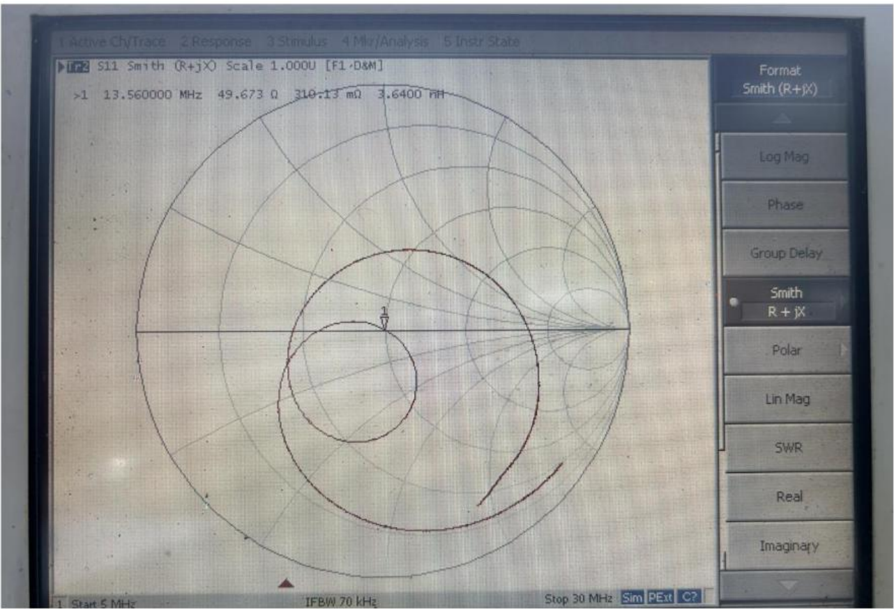
Smith Chart
