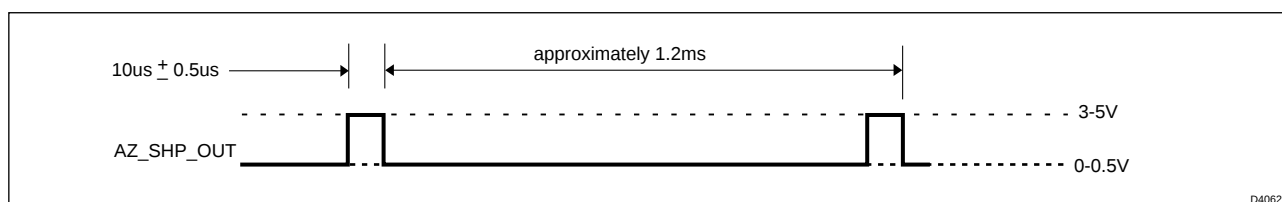
Figure 10. AZ_SHP_OUT / AZIM_DPOS
