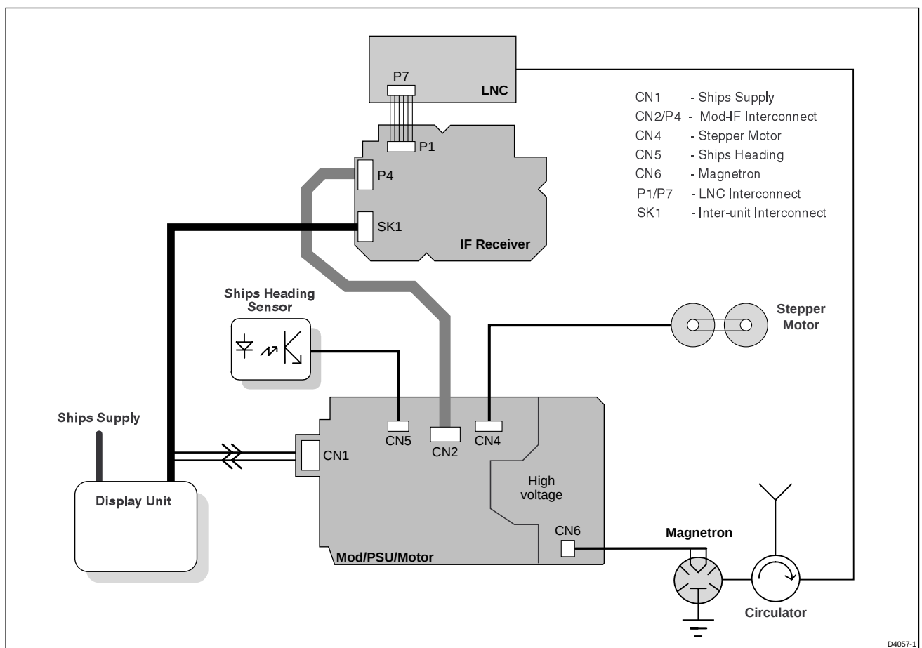
Figure 4. Scanner Interfaces
