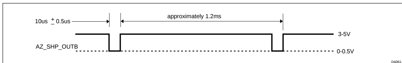
Figure 9. AZ_SHP_OUTB / AZIM_DNEG
