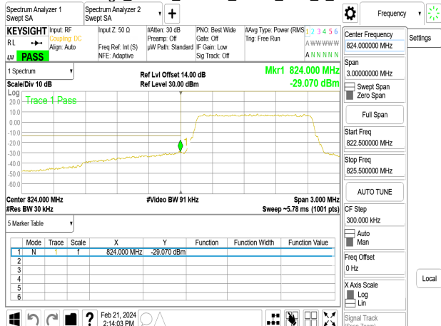
Band Edge_Band5_1.4MHz_QPSK_RB6_0_CH20407
