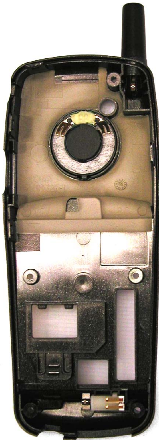
Figure 2-12 Rear housing
