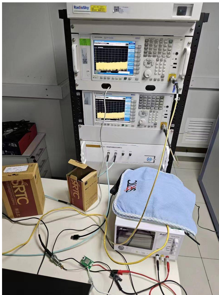
RF Conducted Test setup (WIFI)
